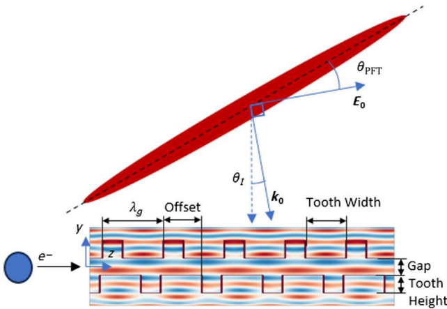
FIG. 1. A cartoon showing a linearly polarized laser with pulse-front-tilt angle \theta_{PFT} arriving at incident angle \theta_I on a structure with periodicity \lambda_g . We show the field distribution of the matched mode inside the structure.
