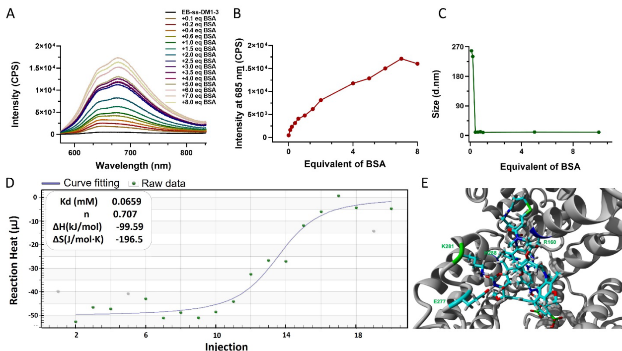
Fig. 2 (A) The emission spectra of EB-ss-DM1-3 and (B) fluorescence intensity at 685 nm and (C) hydrodynamic diameter in the presence of different equivalents of BSA (EB-ss-DM1-3, 5 \mu M in PBS; BSA, 0.5–40 \mu M in PBS. Excitation: 560 nm). (D) ITC determination of the binding thermodynamics of EB-ss-DM1-3 and BSA binding affinity. (E) Predicted structure of the EB-ss-DM1-3/HSA nanocomplex. HSA (gray) is represented in solid ribbon. EB-ss-DM1 prodrugs and the residues in the binding site of HSA are represented in stick.
