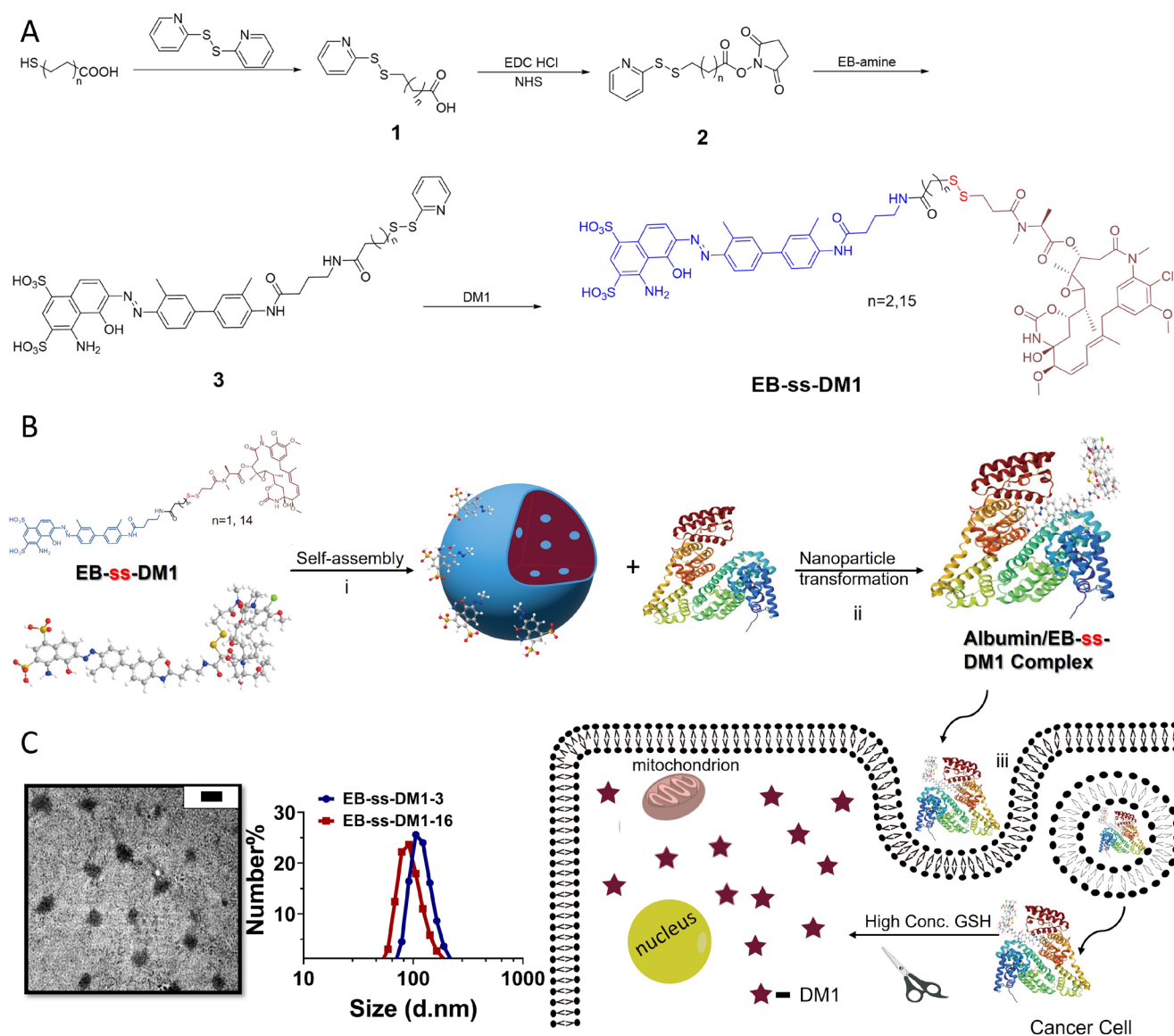
Fig. 1 (A) Synthesis of EB-ss-DM1 (EB-ss-DM1-3, n=1; EB-ss-DM1-16, n=14). (B) i. Formation of the nanoparticle from the self-assembly of amphiphilic DM1 prodrug. ii. Nanoparticle transformation through binding with albumin. iii. The responsive DM1 release in cancer cell. (C) Characterization of self-assembled EB-ss-DM1 nanoparticles (Left: A TEM image of EB-ss-DM1-3. The scale bar represents 200 nm; Right: Size distribution as measured by DLS).
