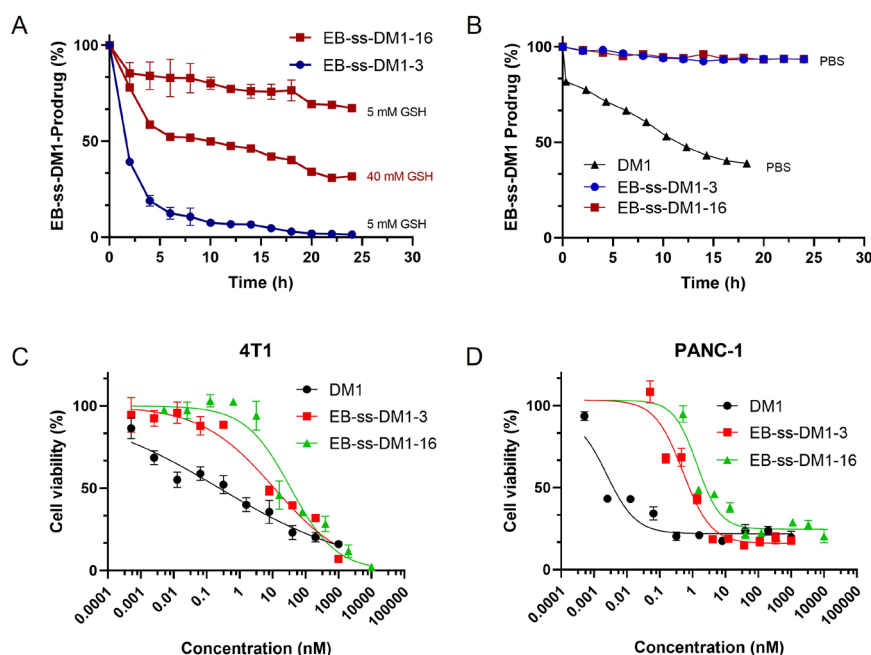
Fig. 3 In vitro drug release (A) in the presence of 5 mM or 40 mM GSH and (B) without GSH over 24 h at 25°C in PBS, as monitored by the decrease of EB-ss-DM1 prodrugs by HPLC, and in vitro cytotoxicities of EB-ss-DM1-3, EB-ss-DM1-16, and DM1 against (C) 4T1 and (D) PANC-1 cancer cells.
