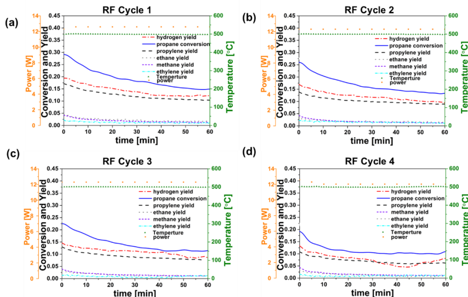
Figure 4. Time-on-stream conversion and yield for propane dehydrogenation reaction in a washcoated monolith reactor during RF heating for (a) Cycle 1, (b) Cycle 2, (c) Cycle 3, and (d) Cycle 4. The radio frequency during each reaction cycle was chosen to be 166 MHz. Experimental conditions: 6% C_3H_8 , 3% H_2 , balance Ar, total flowrate = 75 sccm.
