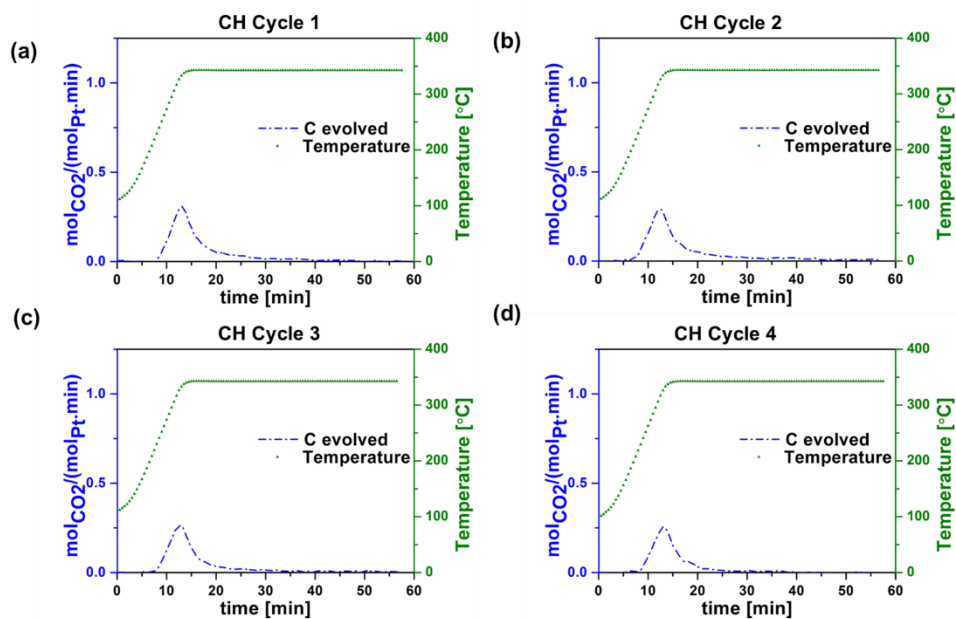
Figure 5. Carbon evolved during regeneration step during Conventional (oven) Heating (CH) in (a) Cycle 1, (b) Cycle 2, (c) Cycle 3, and (d) Cycle 4. Experimental conditions: 30 sccm (20 O 2 in argon)
