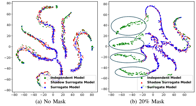
Figure 4. The t-SNE visualization of posterior probability for D_{train} from the CiteSeer dataset in Setting IV. Part (a) compares the target model, a shadow surrogate model, and the real surrogate model without masking ; Part (b) shows a similar comparison when masking 20% features . The circled regions in Part (b) highlight where the target model differs from the other two models.
