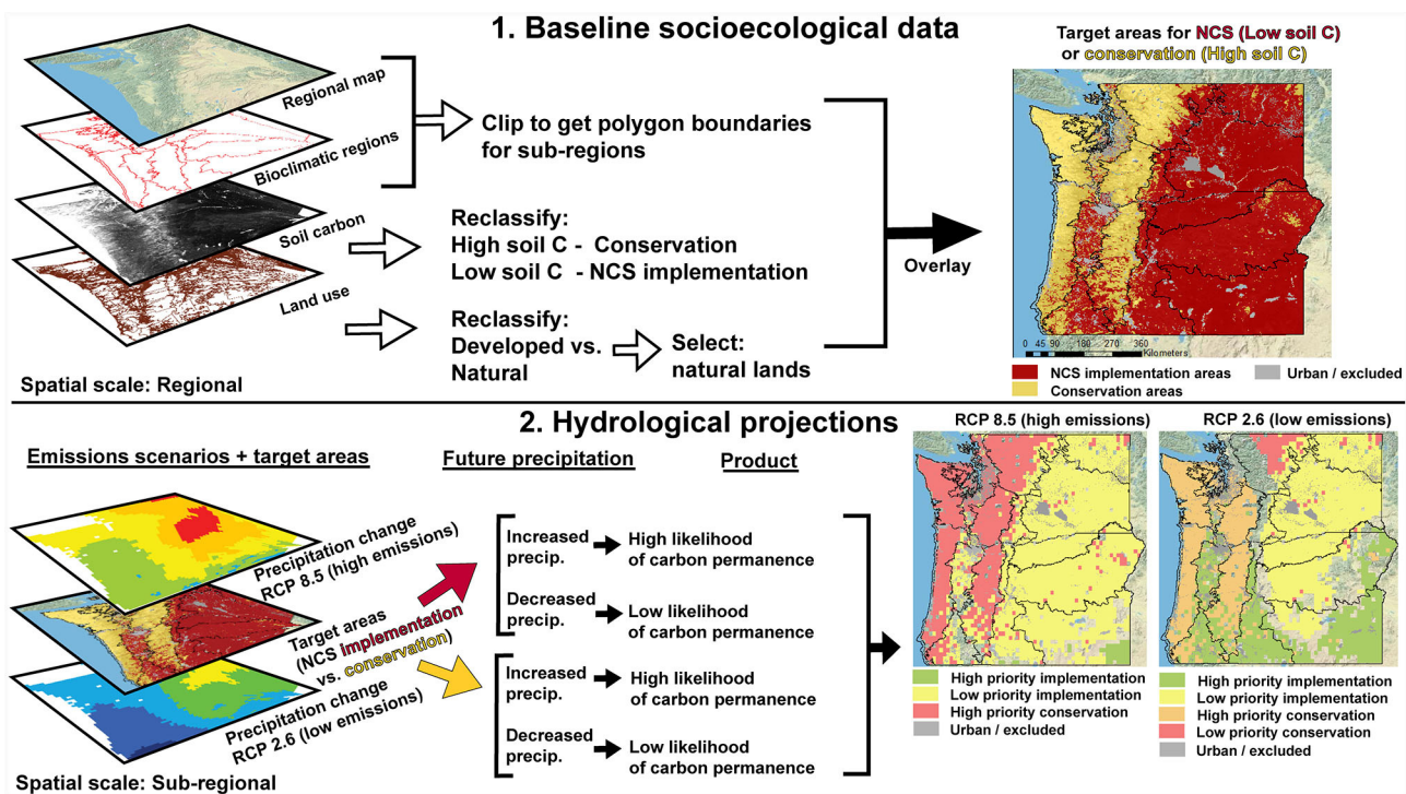
FIGURE 2 A proposed framework for prioritization of natural climate solutions (NCS) implementation areas or conservation across regional and local spatial scales. Step 1 uses baseline data of a socio-ecological context including bioclimatic zones, soil carbon stocks, and land use to identify target areas for NCS implementation and conservation, respectively. Step 2 combines those target areas with future projections of precipitation using both high and low emission scenarios to rank areas by priority.
