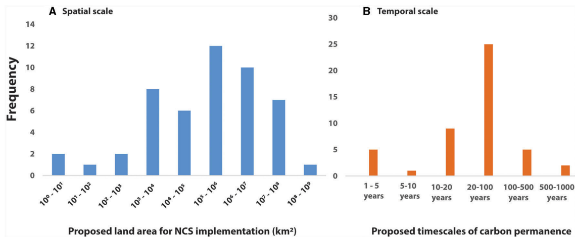
FIGURE 1 Data from previously published work showing the spatial and temporal domains of natural climate solutions (NCS) research. (A, B) Histograms of (A) the spatial scale of NCS implementation and (B) temporal scales of carbon permanence collectively gathered from a survey of 30 studies focused on natural climate solutions. Local scales are defined here as \sim 10^1 - 10^2 km 2 and regional scales are \sim 10^2 - 10^3 km 2 .
