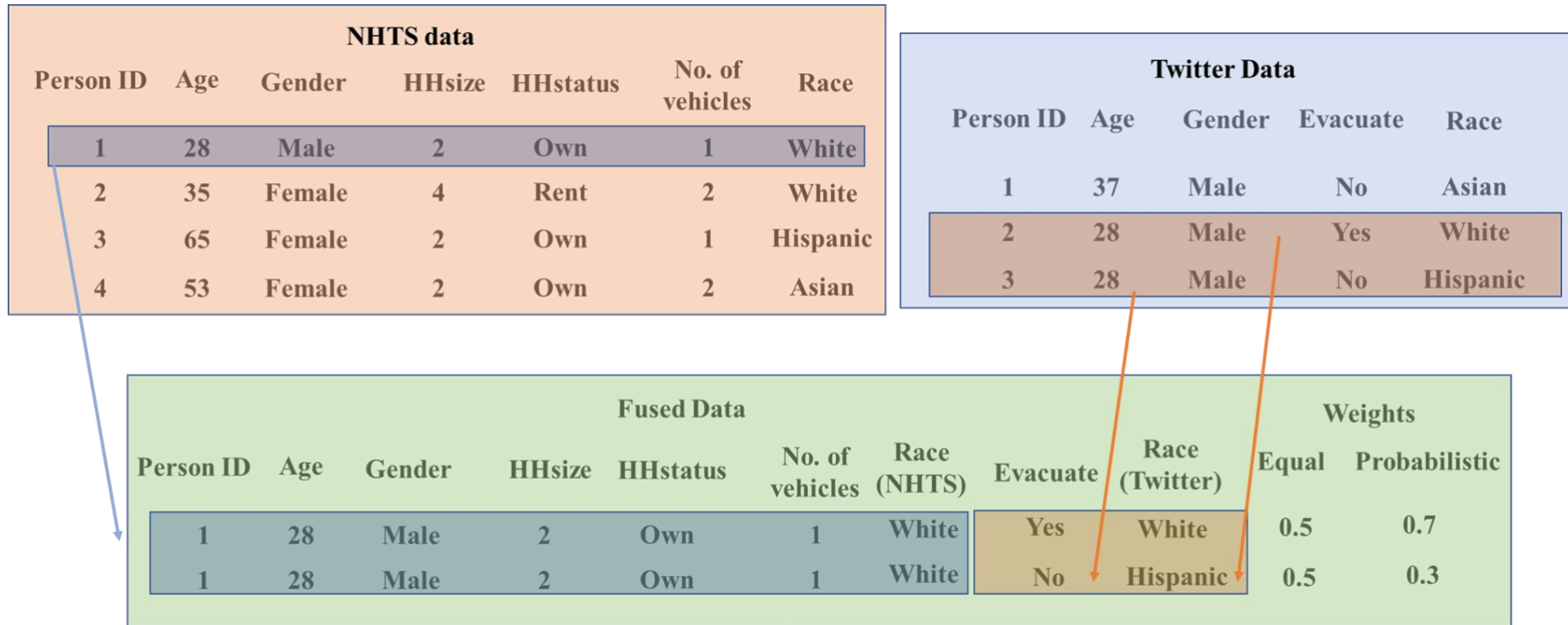
Figure 1: NHTS and Twitter Data Fusion Illustration
