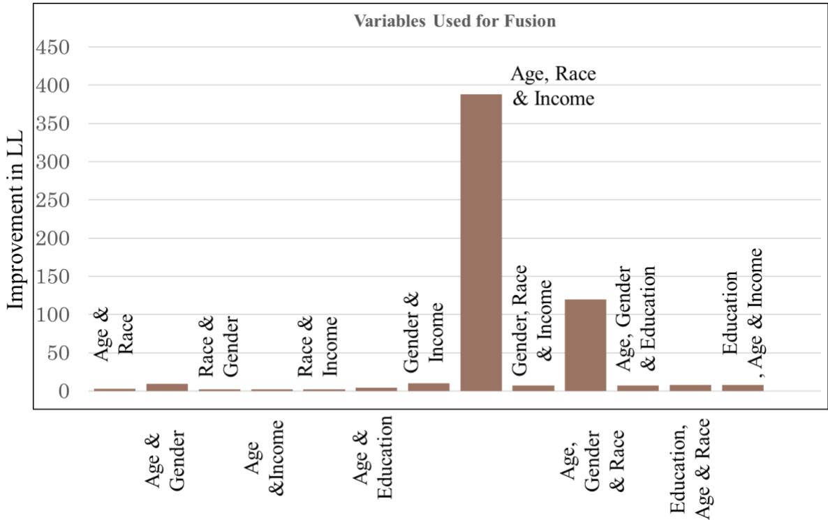
Figure 5: Model Fit Summary Across Different Variable Group Used for Fusion
