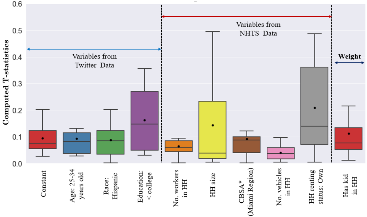
Figure 7: Test Statistics (t-statistics) for Parameter Estimates Across Samples for each Variables and Models
