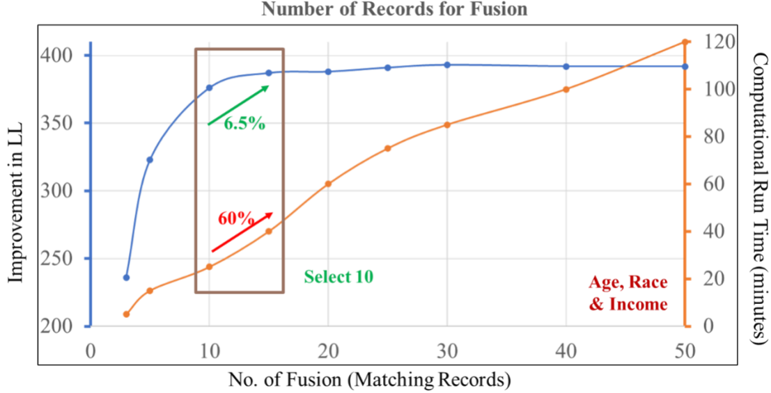
Figure 6: Model Fit Summary Across Different Number of Fusion
