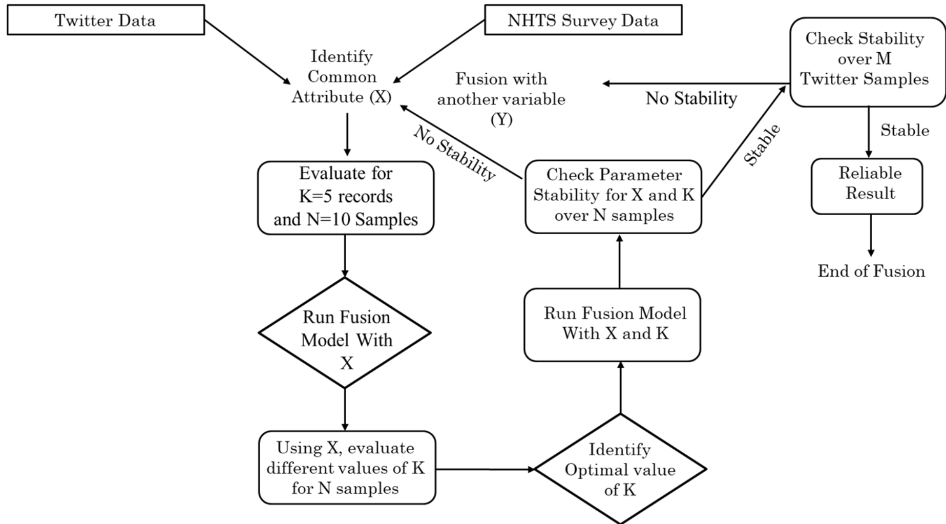
Figure 2: Flow Chart Showing the Framework of the Fusion Algorithm
