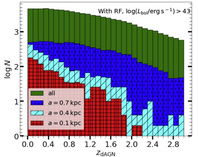
Figure 7. As Figure 1, but now showing the redshift distributions when including the effects of radiation feedback.
