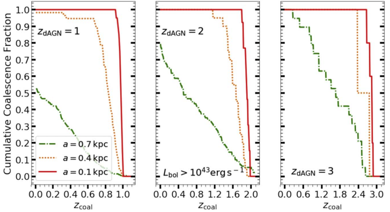
Figure 5. The cumulative coalescence fractions of dAGNs with L_{\text{bol}} > 10^{43} \text{ erg s}^{-1} at z_{\text{dAGN}} = 1, 2 , and 3 . The dotted–dashed green lines show the CCFs of dAGNs with separations of a = 0.7 \text{ kpc} , while the dotted orange lines and solid red lines represent dAGNs with separations of 0.4 and 0.1 \text{ kpc} , respectively.
