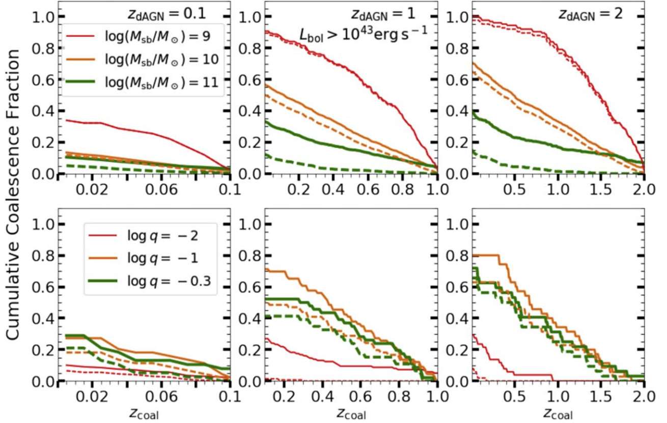
Figure 6. The cumulative coalescence fractions of dAGNs at z_{\text{dAGN}} = 0.1, 1 , and 2 with L_{\text{bol}} > 10^{43} \text{ erg s}^{-1} grouped by the stellar bulge mass (top row) and the MBH mass ratio (bottom row). The dashed lines show the CCFs of mergers that result in LISA events with S/N > 8 .
