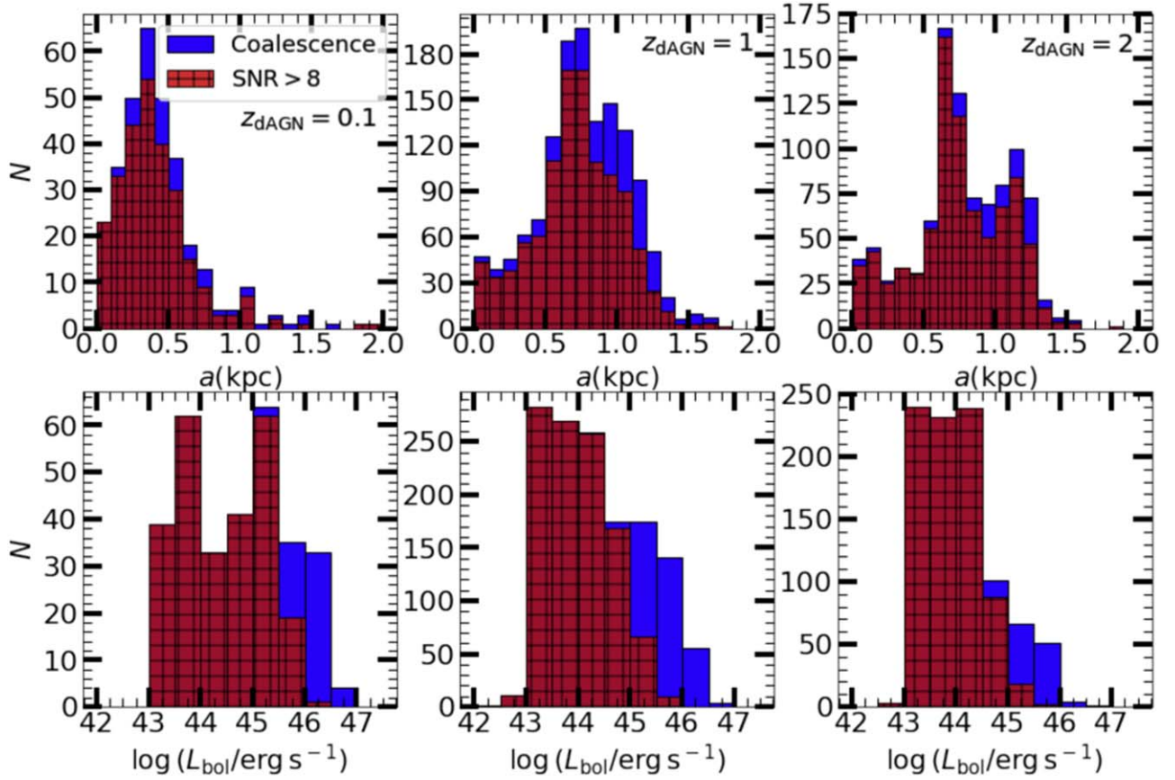
Figure 2. The separation and luminosity distributions at z_{\text{dAGN}} = 0.1, 1 , and 2 of dAGNs whose MBHs coalesce by z = 0 . The blue solid histograms show all dAGNs that eventually lead to coalescence by z = 0 , and the red hatched histograms show the systems in which the MBH merger has a LISA S/N > 8 .
