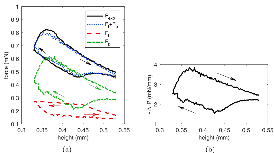
Figure 4. (a) Evolution of the force contributions to the normal force for two plates connected by a capillary bridge. Positive force measurements indicate the attraction between the plates. F_p , the force contribution due to the surface tension around the three-phase contact line, is indicated by the dash-dotted line. F_p , the force contribution due to the Laplace pressure inside the bridge, is indicated by the dashed line. The total force, F = F_l + F_p , is indicated by the dotted line. The experimentally measured force is indicated by a solid line. (b) Evolution of the Laplace pressure.
