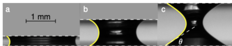
Figure 1. Experimental images for three different bridge heights. The bridge outlines are found through MATLAB image processing. (a) The bridge is at its minimum height; the contact radius and angle are both at their largest values. (b) The bridge is at an intermediate height. (c) The bridge is at its maximum height; the contact radius and angle are both at their minimum values.
