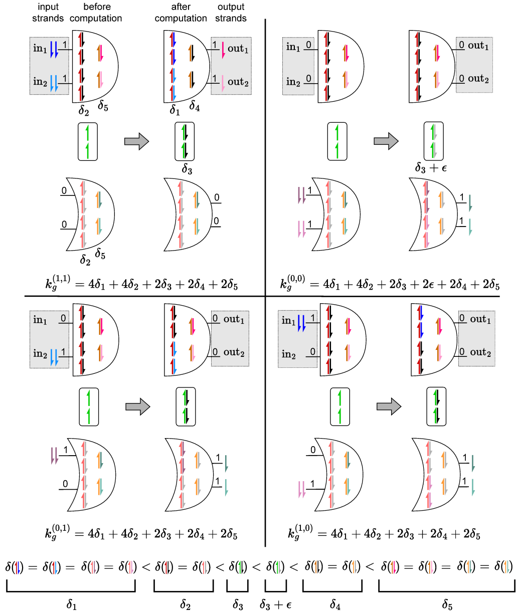
Figure 8 Gate gadget for proof of Theorem 18, showing the design for simulating a circuit consisting of a single AND gate (i.e. depth 1). Simulation of a single AND gate with input bits in_1, in_2 \in \{0, 1\} and output bits out_1, out_2 \in \{0, 1\} . Panels in row-major order respectively show input bit pair 11, 00, 01, and 10. Intuitively, the gadget simulates AND in a dual-rail fashion using three components: an AND component, plus two components that work together to act as a dual to the AND: a small intermediate component (green strands) and an OR component. Together, with a dual rail encoding of the input bits, the three components work to keep the gate energy ( \Delta G() ) almost constant (i.e. constant up to -\epsilon ). To simulate an OR gate, the same gadget is used, except that inputs are flipped, and the output comes from the OR instead of the AND component. k_g^{(x,y)} denotes the MFE of gate g with input (x, y) .
