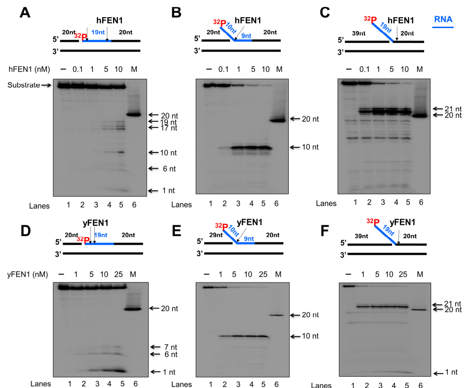
Figure 1. FEN1 endonucleolytic cleavage of an RNA strand in RNA:DNA hybrids. Human and yeast FEN1 cleavage activity on a RNA strand of RNA:DNA hybrid was measured by incubating different concentrations of FEN1 (0.1–25 nM) with the substrates (25 nM) that mimics the intermediates generated during DNA lagging strand processing. Substrates were radioactively labeled at the 5′-end of the downstream strand containing an RNA (blue) and DNA (black) fragment on the same strand. (A) Human FEN1 cleavage on the nicked RNA:DNA hybrid substrate. (B) Human FEN1 cleavage on the RNA:DNA hybrid substrate intermediate containing a 9 nt-RNA flap. (C) Human FEN1 cleavage on the substrate containing a 19 nt-RNA flap attached to a duplex DNA. (D) Yeast FEN1 cleavage on the substrate containing a nicked RNA:DNA hybrid. (E) Yeast FEN1 cleavage on the substrate containing a 9 nt-RNA flap in a RNA/DNA hybrid. (F) Yeast FEN1 cleavage on the substrate containing a 19 nt-RNA flap attached to a duplex DNA. Lane 1 represents substrate only. Lanes 2–6 represent the reaction mixture with increasing concentrations of FEN1. “M” represents a size marker of 20 nt. Substrates and products were separated in a 15% urea-denaturing polyacrylamide gel and detected by phosphorimager. All experiments were performed in triplicate.
