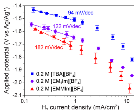
Figure 5. Tafel plots of H 2 formation in 0.2 M [TBA][BF 4 ] (blue), [EM 4 Im][BF 4 ] (purple), or [EMMIm][BF 4 ] (red) electrolytes with 0.05 M [Et 3 NH]Cl under Ar purging. The slope from 0.2 M [EMMIm][BF 4 ] in linear regime is much steeper than that from 0.2 M [EM 4 Im][BF 4 ] and 0.2 M [TBA][BF 4 ], indicating the more sluggish kinetics of proton reduction and hydrogen adsorption in 0.2 M [EMMIm][BF 4 ], likely due to the dense layer of potential driven assembly of [EMMIm] + on Ag electrode.
