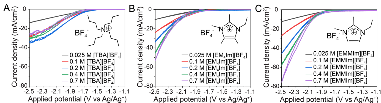
Figure 1. Cyclic voltammetry in CO 2 -purged (A) [TBA][BF 4 ], (B) [EM 4 Im][BF 4 ], and (C) [EMMIm][BF 4 ] electrolytes at concentrations ranging from 0.025 M to 0.7 M. All electrolytes contained 0.05 M [Et 3 NH]Cl as the proton donor and were scanned at 100 mV/s. At concentrations higher than 0.2 M, both [EM 4 Im][BF 4 ] and [EMMIm][BF 4 ] electrolytes give higher current density than [TBA][BF 4 ] electrolytes at matching concentrations, while the highest current density was achieved in [EMMIm][BF 4 ] electrolytes. These comparisons suggest the critical role of imidazolium ring structure in facilitating CO 2 reduction.
