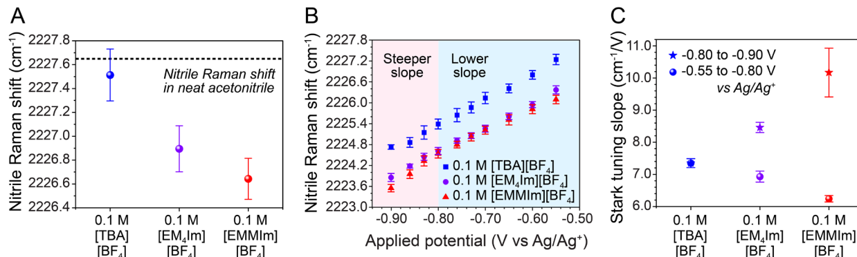
Figure 6. Raman shifts of the nitrile group from 4-MBN in 0.1 M [TBA][BF 4 ] (blue), [EM 4 Im][BF 4 ] (purple), and [EMMIm][BF 4 ] (red). (A) Raman shifts of the nitrile group at OCP in three electrolytes. The nitrile group exhibits redshifts in all three electrolytes. The redshifts are more significant in the two imidazolium-based electrolytes, indicating the stronger stabilization of the nitrile dipole by imidazolium. (B) Potential-dependent Raman shifts of the nitrile group in the three electrolytes. Larger redshifts of the nitrile group are observed in both imidazolium-based electrolytes across the whole potential range tested, suggesting that the potential-driven assembly of imidazolium gives rise to a stronger interfacial electric field that stabilizes the nitrile dipole. Further, two distinct Stark tuning slopes were observed for both imidazolium-based electrolytes in different potential ranges. (C) Potential-dependent Stark tuning slopes in three electrolytes. Compared to 0.2 M [TBA][BF 4 ], both 0.2 M [EM 4 Im][BF 4 ] and [EMMIm][BF 4 ] exhibit lower slopes under less cathodic applied potentials and steeper slope under more cathodic applied potentials, suggesting the ordered pre-assembly and more efficient potential-driven assembly of imidazolium in two potential ranges, respectively.
