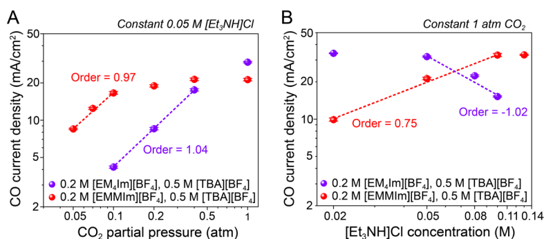
Figure 4 Reaction orders of CO formation with respect to (A) CO 2 and (B) [Et 3 NH] + in electrolytes consisting of 0.5 M [TBA][BF 4 ] and 0.2 M [EM 4 Im][BF 4 ] (purple) or 0.2 M [EMMIIm][BF 4 ] (red). For each trial, the potential was held at -2.5 V vs Ag/Ag + for 11 min under stirring (600 rpm) and purging. (A) CO formation rate, characterized by CO partial current density, shows a first-order dependence on CO 2 partial pressure in both [TBA] 0.5 /[EM 4 Im] 0.2 [BF 4 ] and [TBA] 0.5 /[EMMIIm] 0.2 [BF 4 ]. In [TBA] 0.5 /[EMMIIm] 0.2 [BF 4 ], the CO formation rate saturates at 0.1 atm CO 2 and achieves a maximum of around -20 mA/cm 2 , indicating the existence of other factors limiting the rate of CO 2 reduction. In [TBA] 0.5 /[EM 4 Im] 0.2 [BF 4 ], the CO formation rate continuously increases with CO 2 partial pressure until 1 atm CO 2 , where -30 mA/cm 2 of CO
