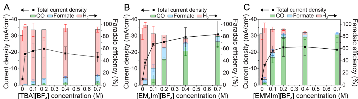
Figure 2. Total current density and product selectivity of electrochemical CO 2 reduction in (A) [TBA][BF 4 ], (B) [EM 4 Im][BF 4 ], and (C) [EMMIIm][BF 4 ] electrolytes at different concentrations with 0.05 M [Et 3 NH]Cl as the proton donor. For each trial, the potential was held at -2.5 V vs Ag/Ag + for 65 min under stirring (600 rpm) and CO 2 purging. Direct reduction of [Et 3 NH] + to H 2 is the dominant reaction pathway in [TBA][BF 4 ] electrolytes. In contrast, both [EM 4 Im][BF 4 ] and [EMMIIm][BF 4 ] electrolytes facilitate CO 2 reduction at concentrations higher than 0.1 M. [EM 4 Im][BF 4 ] electrolytes exhibit higher steady-state total current density and thus overall CO 2 conversion rate by producing both formate and CO, while [EMMIIm][BF 4 ] electrolytes yield lower steady-state total current density but higher selectivity towards CO.
