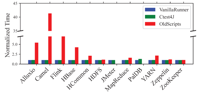
Figure 3: Execution time of running Ctests with Ctest4J, the Ctest scripts [7] (OldScripts), and the vanilla runner such as JUnit4 (VanillaRunner), normalized by VanillaRunner.
