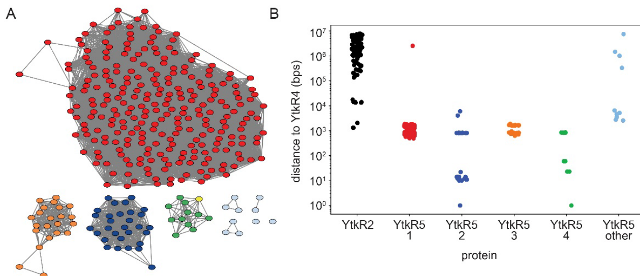
Figure 5. YtkR4 and YtkR5 are found together in clusters. (A) Sequence similarity network (SSN) of BLASTp hits for YtkR5. Nodes are clustered by sequence similarity and colored based on cluster membership, with all clusters with three or fewer members colored light blue. The YtkR5 query sequence is colored yellow. (B) Distance in base pairs in the genome between YtkR4 and YtkR2 or YtkR5 BLASTp hits. YtkR5 hits are further divided into subclasses based on the SSN, with colors corresponding to the SSN in panel a. The "YtkR5 other" category includes all proteins that were in a cluster with three or fewer members.
