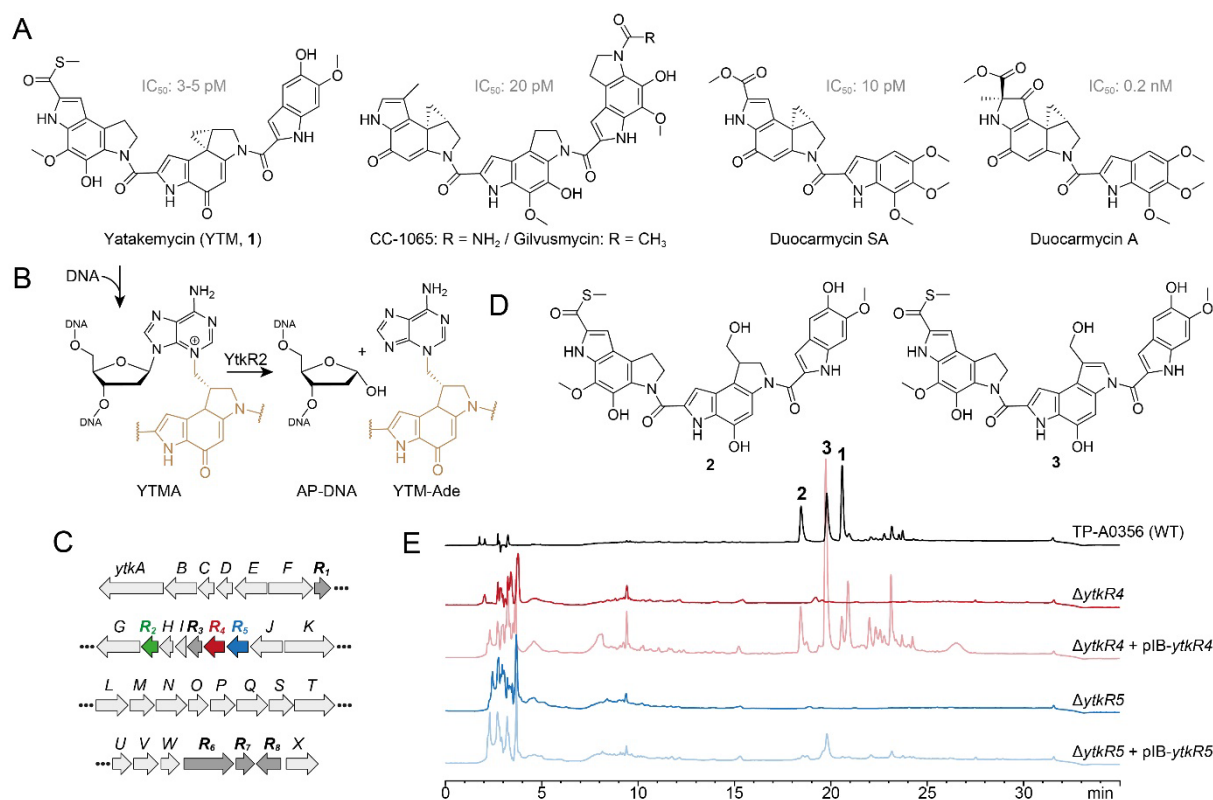
Figure 1. Effects of ytR4 and ytR5 on yatakemycin biosynthesis. (A) Structures of yatakemycin (YTM, 1 ), CC-1065, gilvusmycin, and duocarmycins. (B) YtkR2-catalyzed hydrolysis of a YTMA-DNA lesion yields an AP site in the DNA and free YTM-Ade. The YTM moiety is colored tan. (C) YTM biosynthetic gene cluster. Resistance ( ytR ) genes are labeled bold and highlighted in color or dark grey. (D) YTM hydrolysis products, 2 and 3 . (E) HPLC traces of fermentation products extracted from the wild-type TP-A0356 strain and \Delta ytkR4 and \Delta ytkR5 mutants. Each mutant was analyzed alone and complemented with the corresponding native ytR4 or ytR5 gene (pIB139 vector). The injected concentration of the extracted fermentation products from TP-A0356 is 1/20 that of the other strains. The detection wavelength used was 383 nm.
