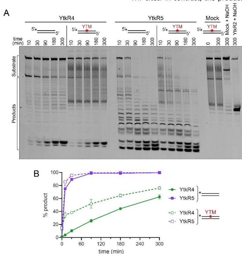
Figure 4. YTMA lesions do not inhibit exonuclease activities of YtkR4 or YtkR5. (A) Denaturing PAGE of YtkR4 and YtkR5 nuclease products on unmodified and YTM-modified dsDNA in the presence of 10 mM MgCl_2 . Mock, no enzyme control. The two lanes at the far right are controls to quantify the percentage of spontaneous depurination of YTMA (Mock + NaOH) and the percentage of DNA alkylated with YTM (YtkR2 + NaOH). Bands quantified as substrates and products are indicated. (B) Quantification of the gel shown in panel A. Data are represented as the mean \pm SD ( n = 2 ).
