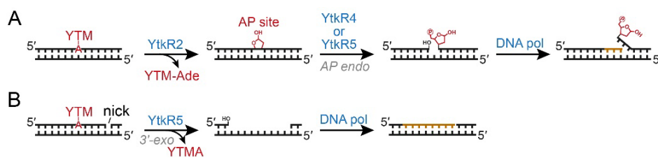
Figure 6. Two possible mechanisms for repair of a YTM-DNA adduct. (A) The YtkR2 glycosylase initiates a BER pathway by excising YTM-adenine. The AP site product is incised by YtkR4 or YtkR5 to generate a 3'-OH, which is a substrate for 5'-deoxyribosephosphate displacement synthesis by a DNA polymerase. (B) The 3'-exonuclease activity of YtkR5, acting at a downstream nick in the DNA, is capable of removing the YTMA nucleotide.
