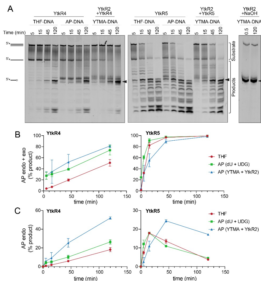
Figure 3. YtkR4 and YtkR5 have greater AP endonuclease activities on abasic sites generated by YtkR2 excision of YTMA. (A) Nuclease activities of YtkR4 and YtkR5 on dsDNA substrates containing either THF (THF-DNA), an AP site generated by UDG excision of deoxyuracil (AP-DNA), or the product of YtkR2 excision of YTMA (YTMA-DNA). The far-right panel shows non-enzymatic (NaOH) cleavage of the AP site generated from the YtkR2/YTMA-DNA glycosylase reaction. Bands quantified as substrates and products are indicated. Black triangles designate the bands resulting from AP endonuclease activity. (B) Quantification of both AP endo and exonuclease products. Data are represented as the mean \pm SD ( n = 2 ). (C) Quantification of AP endonuclease products. Mean \pm SD ( n = 2 ).
