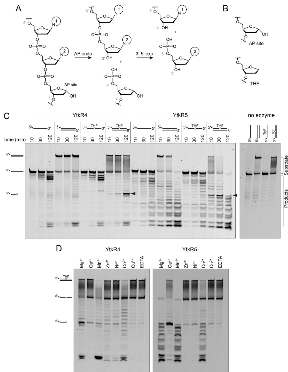
Figure 2. YtkR4 and YtkR5 exhibit 3'-5' exonuclease and AP endonuclease activity. (A) AP endonuclease and 3'-5' exonuclease chemical reactions. Nucleobases are labeled 1 and 2 for identification purposes. (B) Chemical structure of the tetrahydrofuran (THF) abasic analog compared to a natural AP site. (C) Denaturing PAGE of 5'-FAM-labeled substrates incubated with YtkR4 or YtkR5 for the indicated times or with buffer alone (no enzyme) for 120 min. Asterisks (*) in the substrate schematics denote the location of the FAM label. Bands corresponding to substrates and products are indicated to the right of the gel. Black triangles designate the bands resulting from AP endonuclease activity. Duplex DNA persists on the gel because of the high GC content (Supplementary Table S3). (D) Metal dependence for nuclease activity on a 5'-FAM-labeled double-stranded THF-DNA substrate. Reactions were carried out for 2 hr (YtkR4) or 90 min (YtkR5) and contained 10 \mu M protein, 100 nM DNA, and either 10 mM MgCl_2 , 5 mM CaCl_2 , 0.05 mM ZnCl_2 , 3 mM MnCl_2 , 1 mM NiCl_2 , 1 mM CuCl_2 , or 10 mM EDTA.
