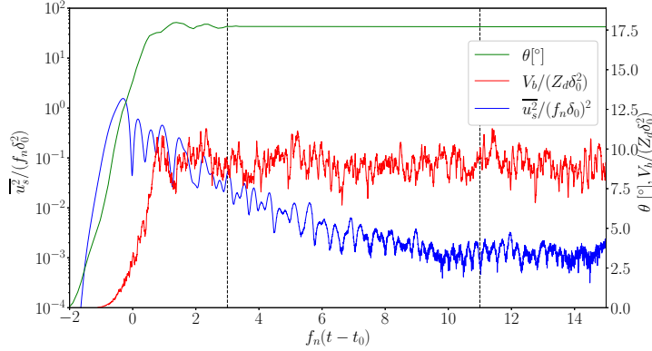
Figure 2: Temporal evolution of dimensionless specific panel kinetic energy, \overline{u_s^2}/(f_n\delta_0)^2 , (shown in blue with a logarithmic scale on the left vertical axis), separation bubble volume (shown in red with a linear scale on the right vertical axis), V_b/(Z_d\delta_0^2) , and wedge angle \theta (shown in green with a linear scale on the right vertical axis in degrees).
