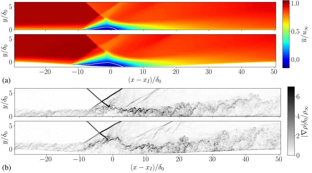
Figure 6: Flexible (bottom) and rigid panel (top) comparison of (a) mean streamwise velocity \bar{u} and (b) numerical schlieren |\nabla \rho| , above the panel ( 210 \leq x \leq 530 mm), along the midspan plane ( z = 0 mm), time-averaged ( t \in [20, 60] ms) for rigid- and flexible-wall simulations, zooming into the STBLI region. White contour lines on the mean velocity plots mark the time-averaged region of flow reversal. An animation for the full integration time of the simulation is provided as supplementary material.
