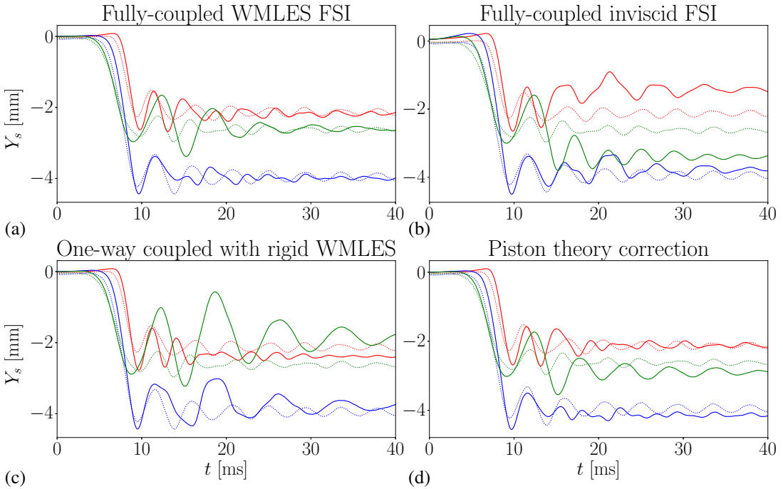
Figure 15: Time signals of vertical panel displacement at front (red), center (blue), and rear (green) probe locations of streamwise location and time, comparing fully-coupled FSI using WMLES (a); fully-coupled FSI using an inviscid flow assumption (b); one-way coupling with pressure from a precursor rigid WMLES (c); one-way coupling FSI with piston-theory correction of the rigid WMLES pressure (d). For each plot, solid lines correspond to the simulation results, and dotted lines correspond to the experiments.
