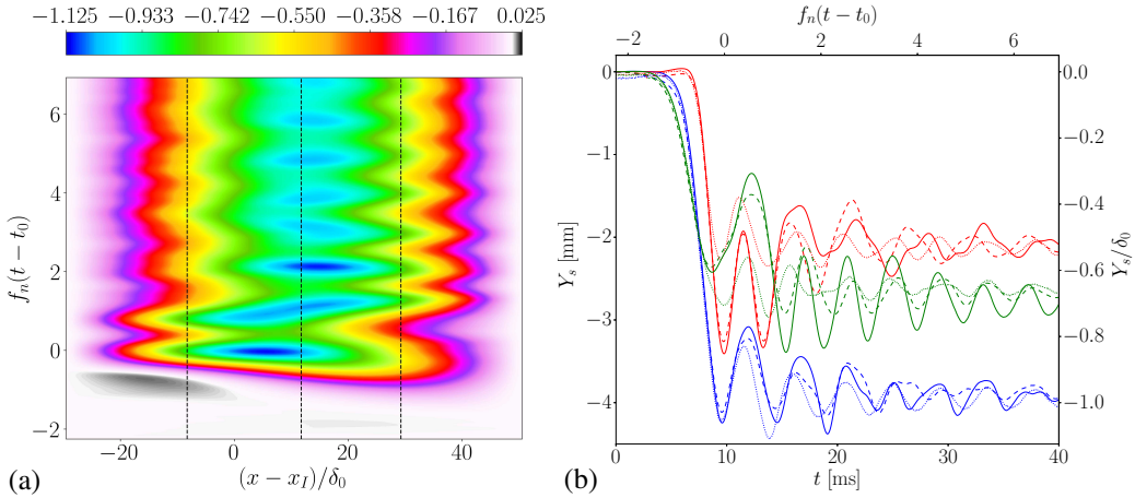
Figure 3: (a) Contours of vertical panel displacement, Y_s/\delta_0 , along the midspan plane as a function of the streamwise coordinate and time, obtained from the full-span simulation. Gray colors indicate positive vertical deflection. (b) Time signals of panel displacement measured at the front (red), center (blue), and rear (green) probe locations marked by vertical dashed lines in (a), comparing results from full-span simulations (solid), previous spanwise-periodic reduced-span simulations (dashed) by [?], and experiments (dotted) by [?].
