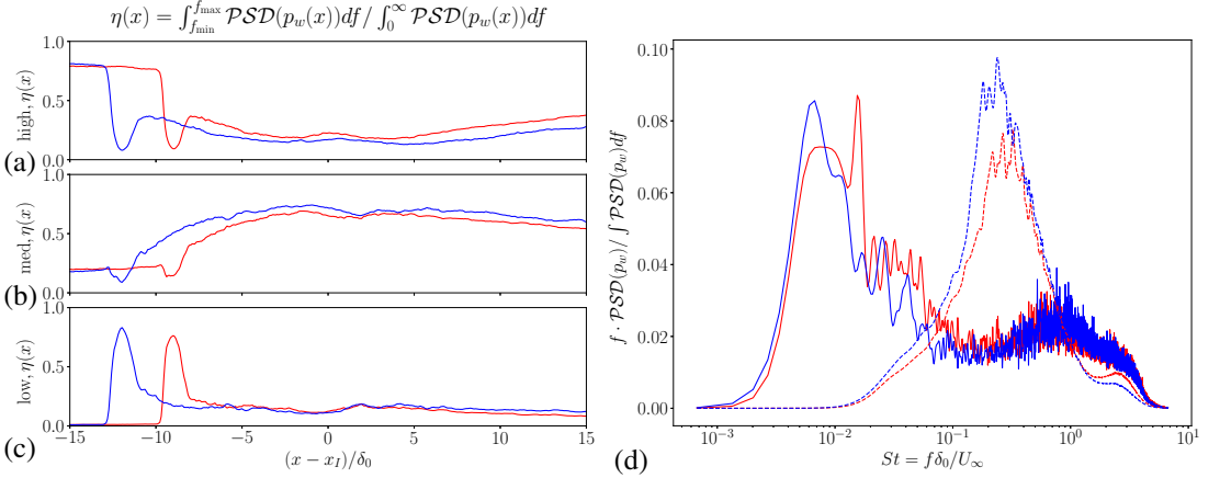
Figure 10: Band contribution \eta(x) to the signal power of wall pressure p_w(x) for (a) high frequency band 0.5 < St < \infty , (b) medium frequency band 0.05 < St < 0.5 , and (c) low frequency band 0 < St < 0.05 . (d) Comparison of rigid and flexible wall pressure PSD for the low frequency motions (solid line style (—)) and the separation bubble (dashed line (- -)). red line color (—) rigid-panel; blue line color (—) flexible-panel.
