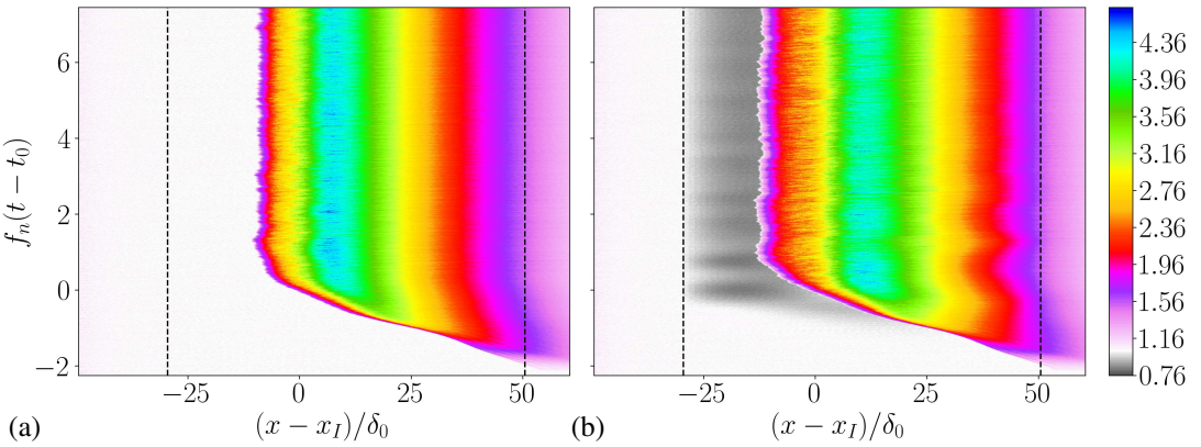
Figure 7: Contours of spanwise-averaged wall pressure p_w/p_\infty as a function of streamwise coordinate and time for rigid (a) and flexible (b) panel simulations. Vertical dashed lines mark the extent of the flexible panel.
