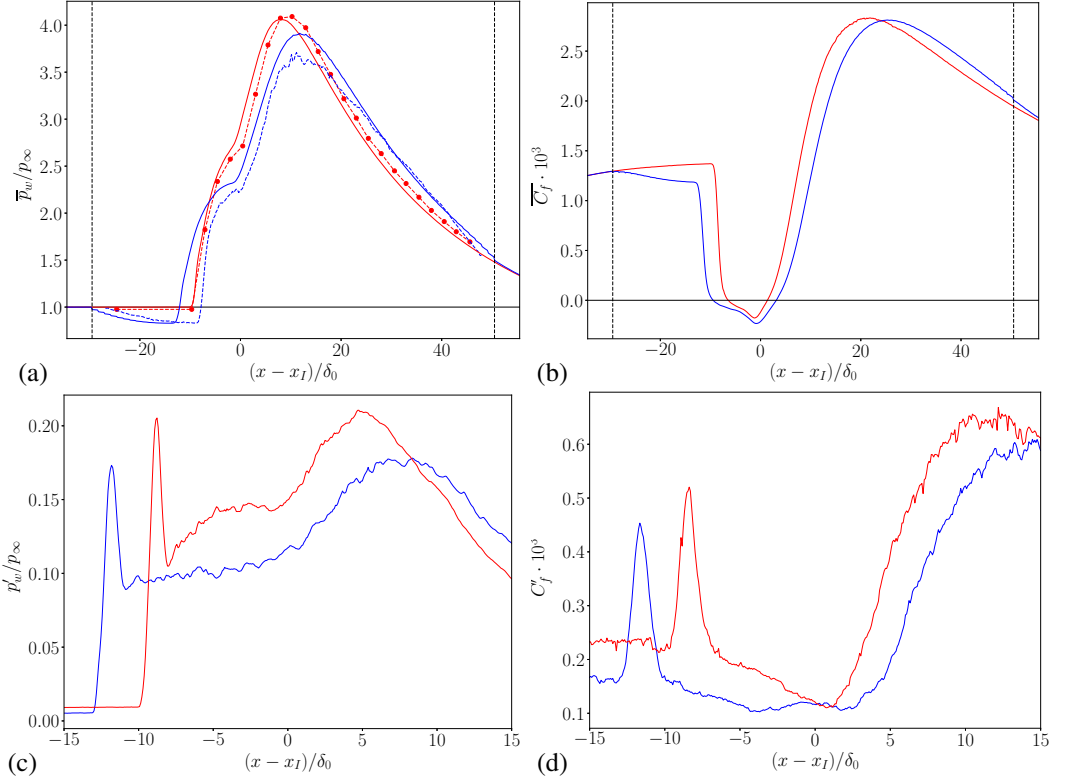
Figure 8: Time and spanwise-averaged streamwise profiles of (a) wall pressure, p_w , and (b) skin friction coefficient, C_f . Zoomed-in flexible and rigid panel comparison of band-limited ( St_{\text{sep}} = f L_{\text{sep}}/u_\infty < 1 ) root mean square of (c) wall-pressure p'_w fluctuations and (d) streamwise skin friction C'_f fluctuations. Solid red line (—): rigid-panel WMLES; solid blue line (—): flexible-panel WMLES FSI; dashed red line with symbols (---): rigid experimental data (?); dashed blue line (---): wall-resolved LES averaged over one oscillation period in the transient phase (?). Black vertical dashed lines in (a,b) mark the extent of the flexible panel.
