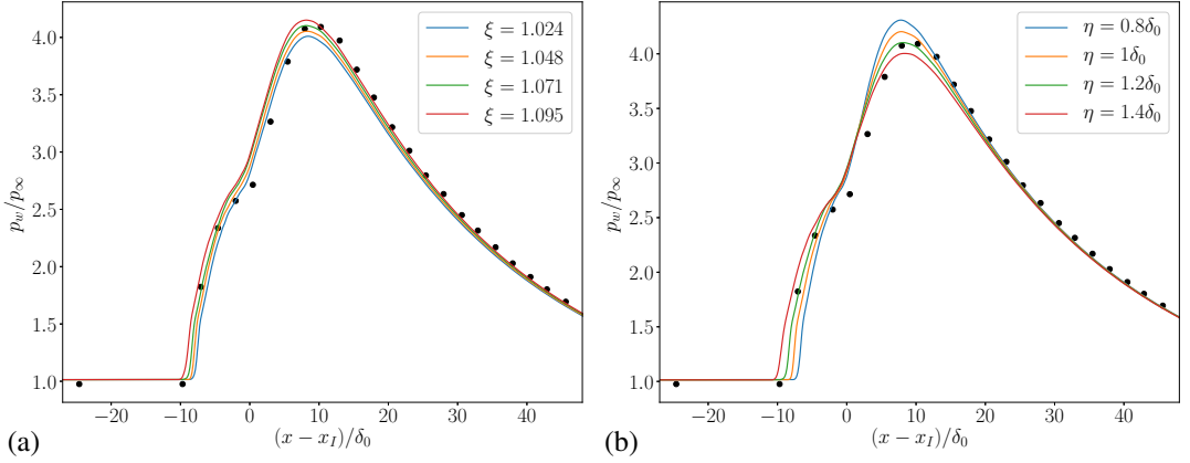
Figure 5: Sensitivity of streamwise profiles of time- and spanwise-averaged wall pressure over a rigid panel to variations in: (a) wedge length ( \xi ) for an incoming boundary layer thickness with \eta = 1.2 ; and (b) incoming boundary layer thickness ( \eta ) for a wedge extension with \xi = 1.069 . Symbols represent experimental measurements by ?.
