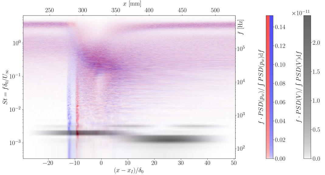
Figure 9: Superposition of power spectral densities (PSD) of wall pressure for rigid (red) and flexible (blue) walls, and of flexible panel displacement (grayscale) as a function of the streamwise location, showing the extent corresponding to the length of the flexible panel. Normalized colorbars use an arbitrary scale (the same for rigid and flexible wall cases).
