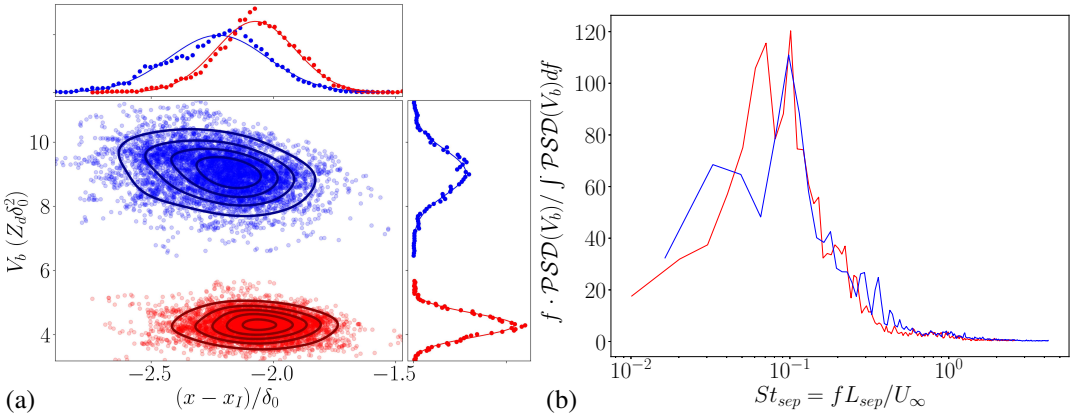
Figure 11: (a) Joint and marginal probability distribution (shown with contour lines) of separation bubble volume and separation bubble x-centroid, after the transient, t' > 3 , with Gaussian distribution fits shown in the marginal PDFs. Markers in the joint PDF correspond to sampled snapshots every 100 time steps. (b) Premultiplied, and normalized power spectral density of separation bubble volume scaled by the Strouhal number based on the separation length ( St_{sep} = fL_{sep}/u_\infty ). The flexible panel results are shown in blue and the rigid panel results are shown in red.
