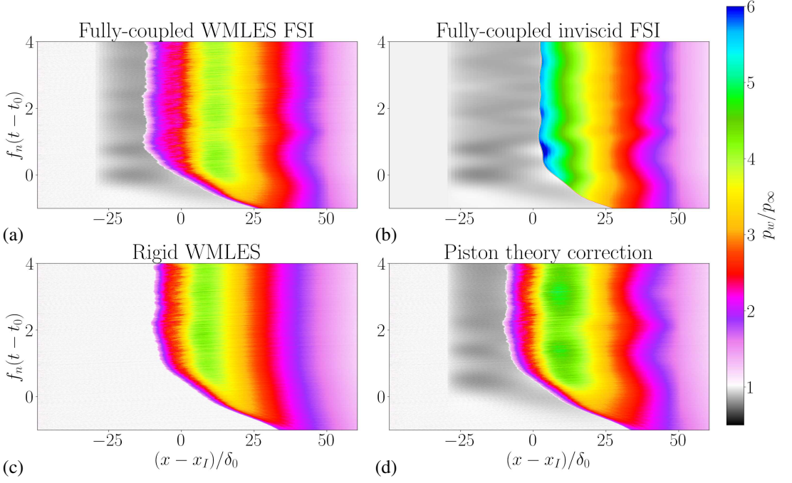
Figure 13: Streamwise wall pressure p_w comparison of fully-coupled WMLES FSI to Rigid WMLES, piston-theory correction of rigid WMLES, and fully-coupled inviscid FSI.
