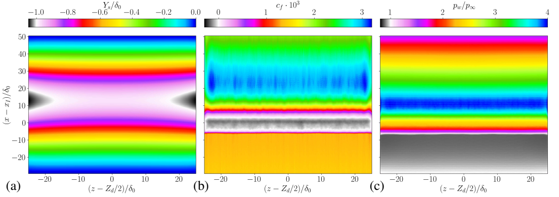
Figure 4: (a) Normalized panel displacement, Y_s/\delta_0 , (b) skin friction coefficient, C_f \cdot 10^3 , and (c) normalized wall pressure, p_w/p_\infty , time-averaged ( t \in [20, 60] ms) on the streamwise-spanwise ( xz ) plane, for the full-span FSI simulation.
