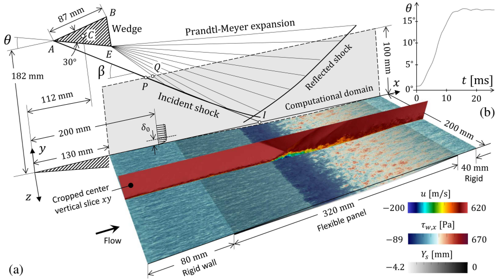
Figure 1: (a) Problem setup following experiments by ? with the simulation domain highlighted in gray on the back vertical plane. Colored contour maps are obtained from an instantaneous snapshot at t = 15 ms from the full-span simulation of the present study, showing the flexible panel vertical displacement, Y_s , the streamwise component of the wall shear stress vector, \tau_{w,x} (in translucent color), and the streamwise component of the fluid flow velocity, u . The latter is shown on a cropped vertical slice ( xy ) at the center of the spanwise domain, highlighting the incident and reflected shocks, the turbulent boundary layer, and the separation bubble.
