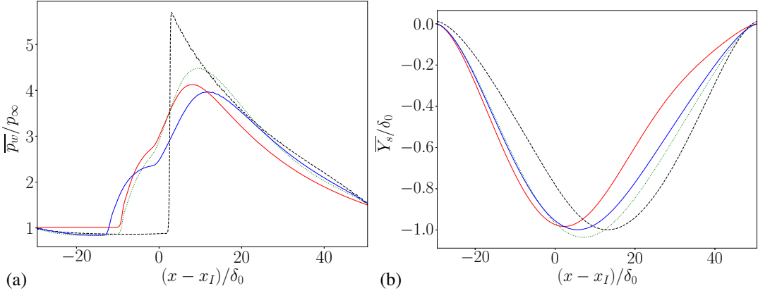
Figure 16: Comparison of time- and spanwise- averaged (a) pressure, p_w , and (b) panel deflection, Y_s , along the streamwise ( x ) direction using: two-way coupled WMLES FSI (solid blue, —); one-way coupled simulation with rigid-wall WMLES pressure time history (solid red, —); one-way coupling simulation with localized piston theory correction (dotted green, ····); two-way coupled FSI with inviscid flow assumption (dashed black, - - -).
