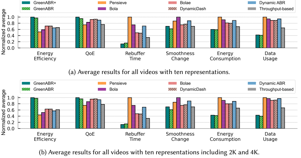
Fig. 5. Comparison of GreenABR with other approaches with ten representations. For QoE, the higher, the better. For other metrics, the lower, the better.
