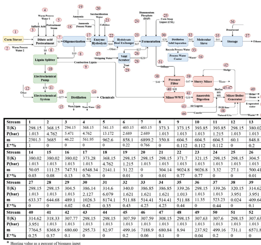
Fig. 5 Process diagram and material stream table for the corn stover to ethanol and EC lignin chemicals biorefinery.
