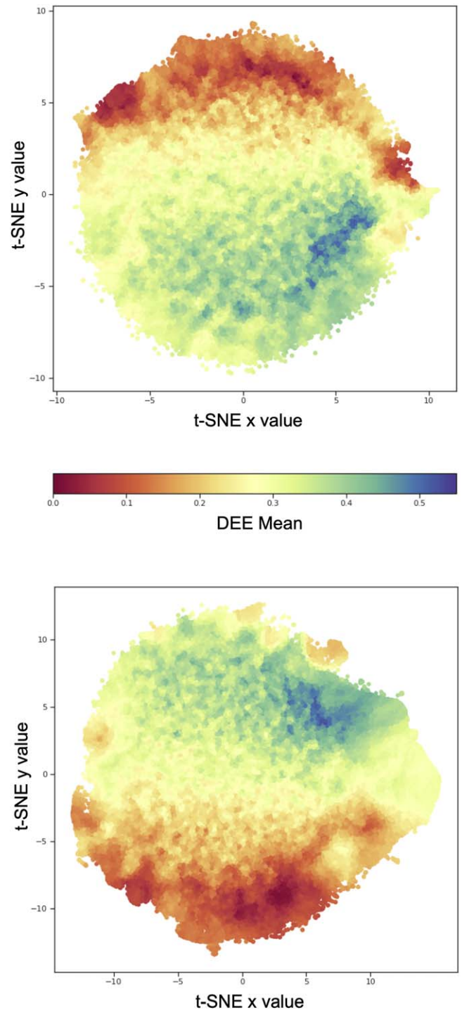
Figure 4. The results of the t-SNE ML algorithm, each with the same hyperparameters. The colors represent the DEE_mean which was developed using the nearest neighbors method. Note: The orientation of the t-SNE axes relative to the data points has no inherent meaning or significance beyond the visualization itself. This is simply a characteristic of the dimensionality reduction algorithm.
