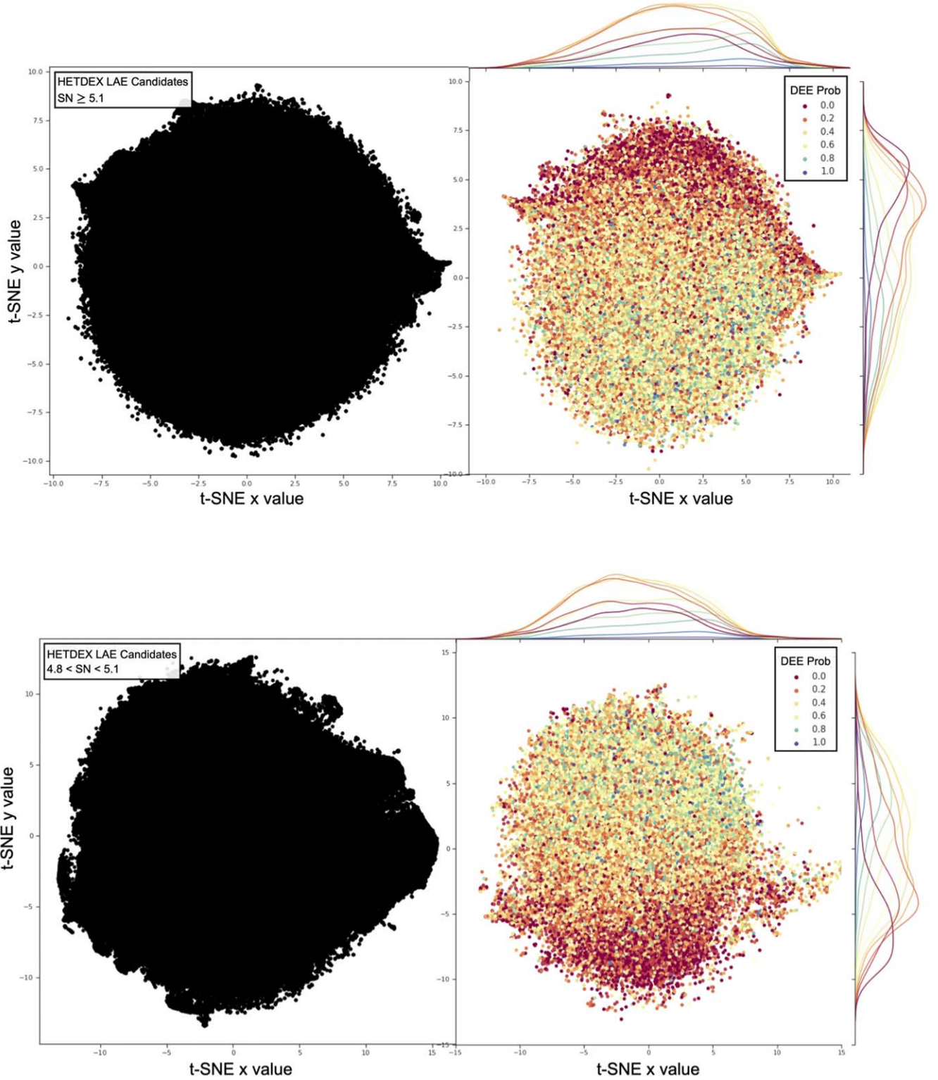
Figure 3. The results of the t-SNE ML algorithm, each with the same hyperparameters and each row has the same t-SNE projection. On the left-hand side, the plots shown in black are \approx 1.2 million HETDEX LAE candidates. On the right-hand side, the colored plots shown are a result of the \approx 190,000 LAE candidates that have been labeled by Dark Energy Explorers and assigned a DEE_probability. The top two plots show the LAE candidates above SN ratio \geq 5.1 and the two bottom plots show the LAE candidates with 4.8 < \text{SN} < 5.1 . Note: The orientation of the t-SNE axes relative to the data points has no inherent meaning or significance beyond the visualization itself. This is simply a characteristic of the dimensionality reduction algorithm.
