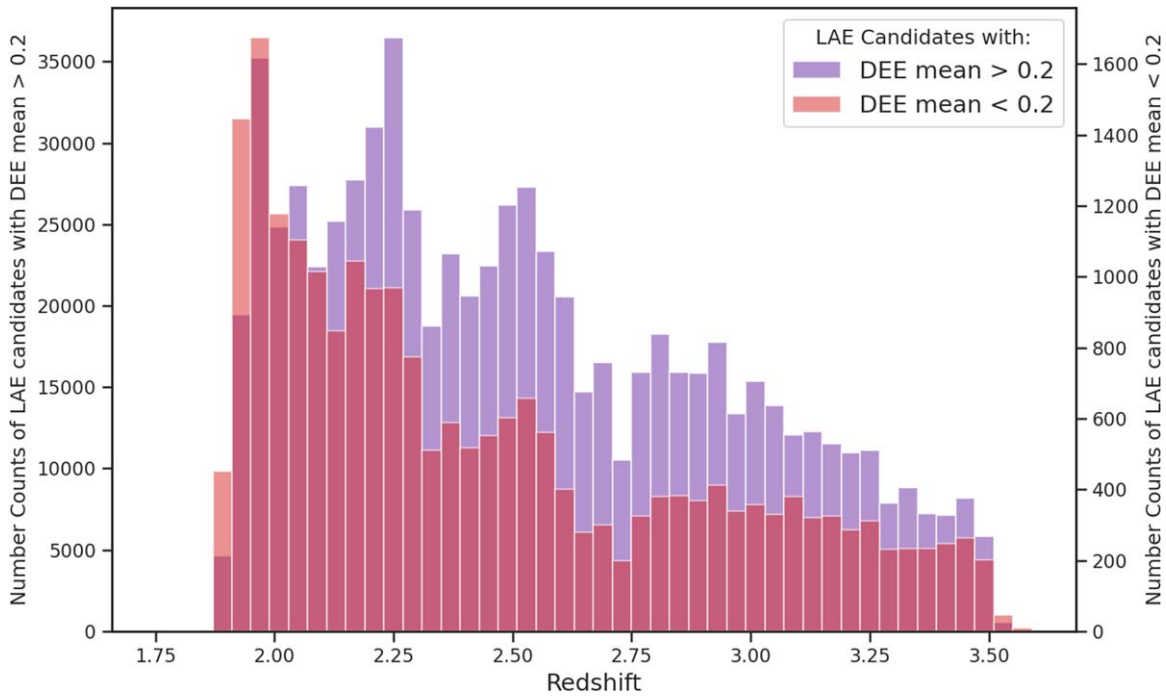
Figure 5. The redshift distribution of the 1.2 million HETDEX LAE candidates with the cut on DEE_mean. DEE_mean is created using the nearest neighbors technique. The histogram in pink identifies the false positives with a DEE_mean < 0.2 and the purple represents a DEE_mean > 0.2, each cut is scaled for comparison, differing by approximately a factor of 20.
