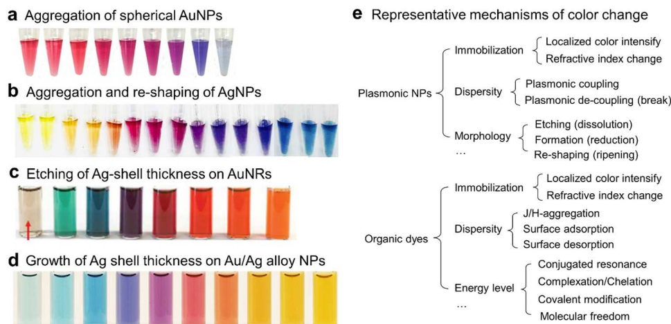
Fig. 3 Representative mechanisms of color changes based on inorganic NPs include: (a) aggregation of AuNPs. 16 (b) Aggregation and re-shaping of AgNPs. 20 (c) Etching of Ag-coated AuNRs. 45 (d) Growth of Ag shell on the Au/Ag alloy NPs. 46 (e) General mechanisms of colorimetric sensing using various colorants. (a) Reproduced with permission from ref. 16. Copyright 2022 Wiley. (b) Reprinted with permission from ref. 20. Copyright 2022 American Chemical Society. (c) Reproduced from ref. 45 (2020) with permission from the Royal Society of Chemistry. (d) Reproduced from ref. 46 in accordance with CC BY-NC-ND 4.0. Copyright 2021 American Chemical Society.
