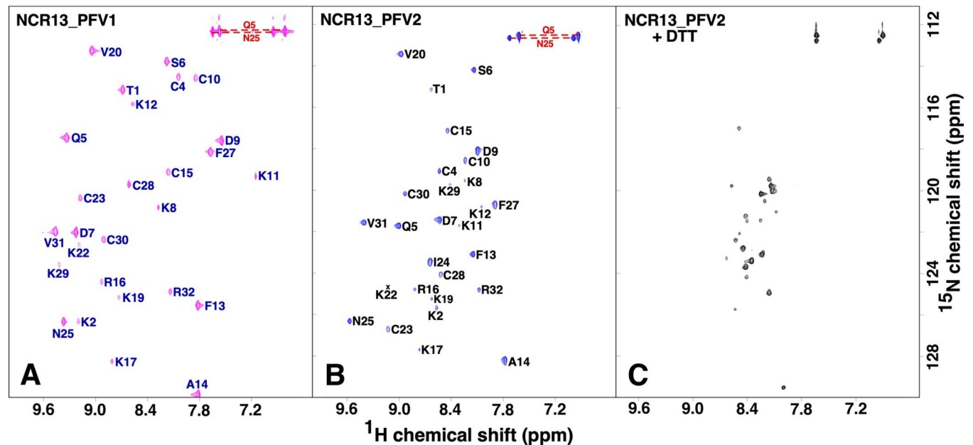
Fig 2. Fingerprint ^1\text{H} - ^{15}\text{N} HSQC spectra for oxidized and reduced NCR13. Assigned ^1\text{H} - ^{15}\text{N} HSQC spectra for oxidized (disulfide) NCR13_PFV1 (A) and NCR13_PFV2 (B). (C) The ^1\text{H} - ^{15}\text{N} HSQC spectrum of fully reduced (dithiol) NCR13_PFV1 and NCR13_PFV2 were identical (the spectrum for NCR13_PFV2 is illustrated). All spectra collected on ~ 1 mM samples at 20°C in 20 mM sodium acetate, 50 mM NaCl, pH 5.3 at a ^1\text{H} resonance frequency of 600 MHz. Amide side chain resonance pairs are connected by a red dashed line. Not within the displayed spectral boundaries is the G26 amide resonance for NCR13_PFV1 and NCR13_PFV2 at 8.66/103.1 ppm and 7.99/101.7 ppm, respectively, and the I24 amide resonance for NCR13_PFV1 at 8.72/132.0 ppm.
