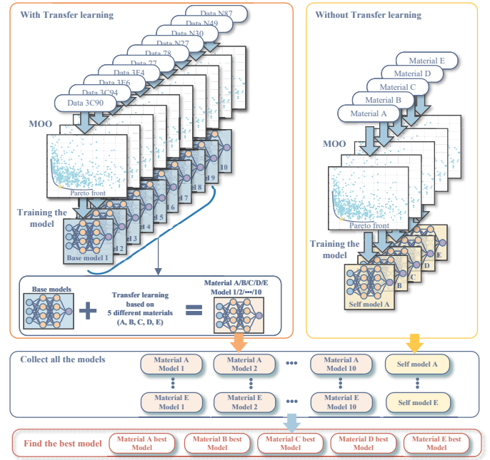
FIGURE 13. The multi-material transfer learning and multi-objective optimization method proposed by TU Delft [42].
