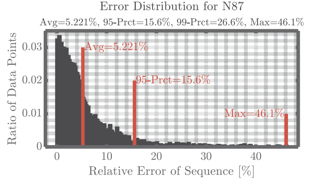
FIGURE 4. Histogram of the prediction error of an example model, together with labeled average, 95 th percentile error, and maximum error.
