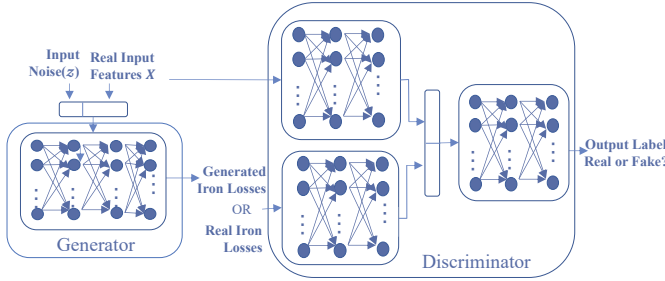
FIGURE 15. The cGANET architecture developed by KU Leuven [43].
