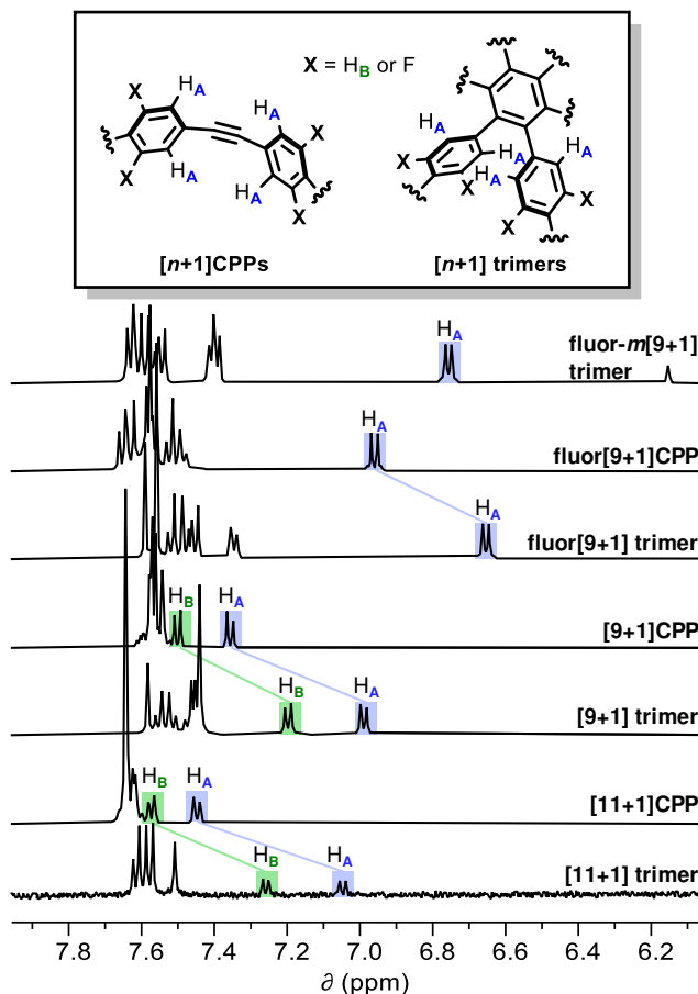
Figure 3. Diagnostic ^1\text{H} NMR shifts for trimers and associated [n+1]\text{CPPs} in \text{CD}_2\text{Cl}_2 .
