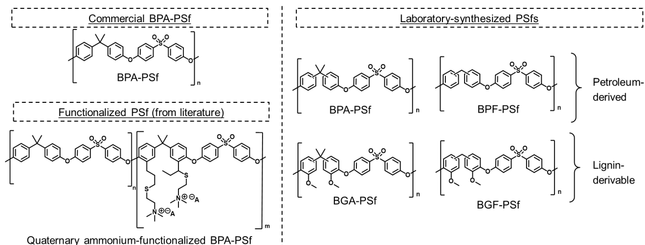
Figure 4: Molecular structures of commercial, functionalized, and synthesized PSfs.
