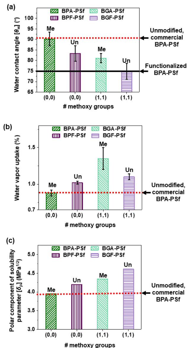
Figure 2: (a) \theta_w , (b) water vapor uptake, and (c) \delta_p values as a function of methoxy groups on the aromatic rings for laboratory-synthesized BPA/BGA/BPF/BGF-PSfs. The bar label indicates the bridging-carbon substitution type for the PSfs. The red dashed line represents a reported value ( \theta_w \sim 90^\circ , water vapor uptake \sim 0.8\% , polar component of solubility parameter \sim 3.9 ) for unmodified, commercial BPA-PSf [Udel ® PSU, Solvay], 2 whereas the black solid line in panel (a) indicates an average reported value in the literature ( \theta_w \sim 75^\circ ) for functionalized BPA-PSf. 10
