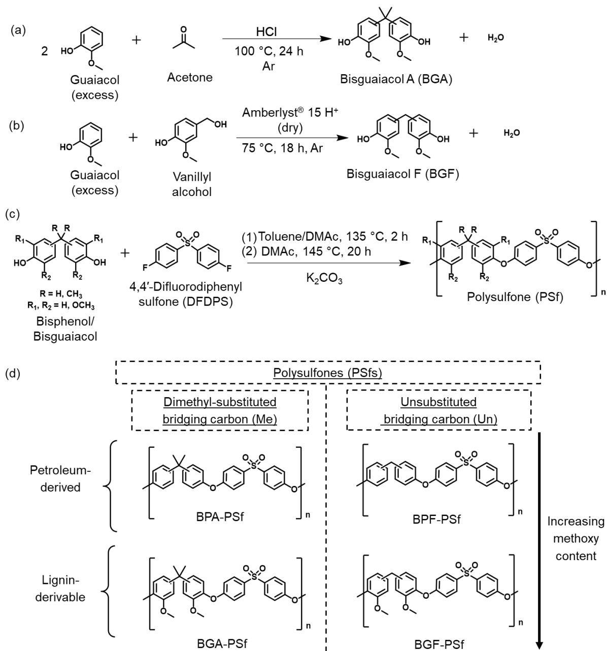
Figure 1: (a) Synthesis of BGA using guaiacol and acetone. (b) Synthesis of BGF using guaiacol and vanillyl alcohol. (c) Synthesis of PSf from respective bisphenol and DFDPS. (d) Molecular structures of synthesized PSfs, wherein the petroleum-derived analogues, BPA/BPF-PSfs (on the top), have no methoxy groups on either ring (0,0), and the lignin-derivable, BGA/BGF-PSfs (on the bottom) have two methoxy groups, one on the right-most and one on the left-most bisphenol aromatic ring (1,1).
