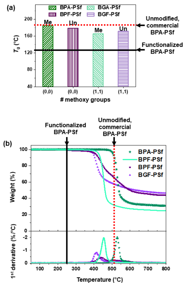
Figure 3: (a) T_g for laboratory-synthesized BPA/BGA/BPF/BGF-PSfs. (b) Representative thermogravimetric analysis traces and the respective first-derivative curves of sample mass remaining versus temperature for laboratory-synthesized BPA/BGA/BPF/BGF-PSfs obtained at a heating rate of 10 °C/min in an N_2 atmosphere. The red dashed line represents a reported value ( T_g \sim 185 °C, T_{d5\%} \sim 510 °C) for unmodified, commercial BPA-PSf [Udel® PSU, Solvay], 2 whereas the black solid line indicates an average reported value in the literature ( T_g \sim 130 °C, T_{d5\%} \sim 250 °C) for functionalized BPA-PSf. 10
