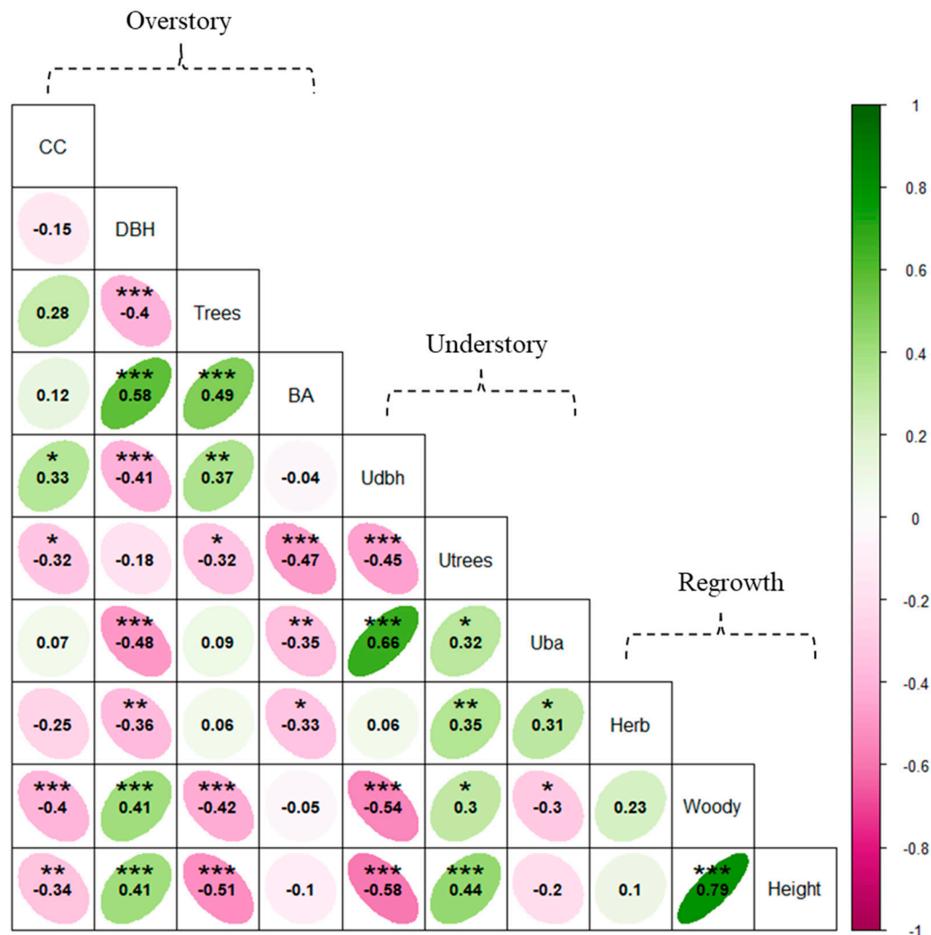
Figure 10. Plots of the relationship between forest attributes pairs. U—understory variables. Overstory variables include DBH, trees/ha, and basal area. Understory variables include U-DBH, U-trees/ha, and U-basal area. Shrub and regrowth layer variables include herb coverage (%), woody plant coverage (%), and maximum shrub height (m). * Significant at the 0.05 level, ** significant at the 0.01 level, *** significant at the 0.001 level.
