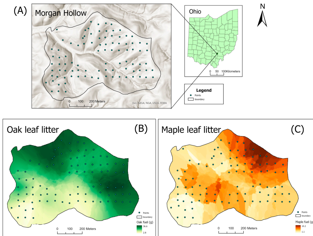
Figure 1. (A) Study area (Morgan Hollow) located in Zaleski State Forest, southern Ohio. The black dots indicate the location of 94 sample plots, approximately 60 m apart from each other and distributed evenly in a gridwork across the study site to capture the differences in forest attributes and fuel characteristics; (B) oak leaf litter distribution; (C) maple leaf litter fuel distribution. Missing points appeared on the northwest and middle south areas of the gridwork due to inaccessible dense vegetation.
