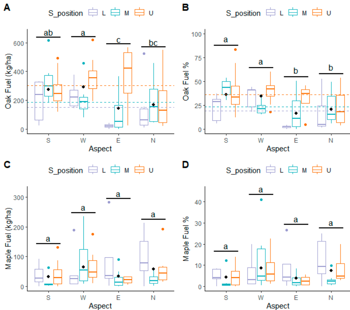
Figure 4. Oak and maple fuel at different aspects in three slope positions (L—lower, M—middle, U—upper). Specifically, (A) oak fuel load (kg/ha), (B) oak litter fuel as a percentage of total 1 h and 10 h fuel load (%), (C) maple fuel load (kg/ha), and (D) maple litter fuel as a percentage of total 1 h and 10 h fuel load (%) over aspects in three slope positions. Figures with the same lower-case letters are not different between aspects within each graph (post hoc Tukey–Kramer test, p = 0.05 ). Black diamonds represent group means for each aspect. Dashed lines represent group means for each slope position. S_position in the legend means slope positions.
