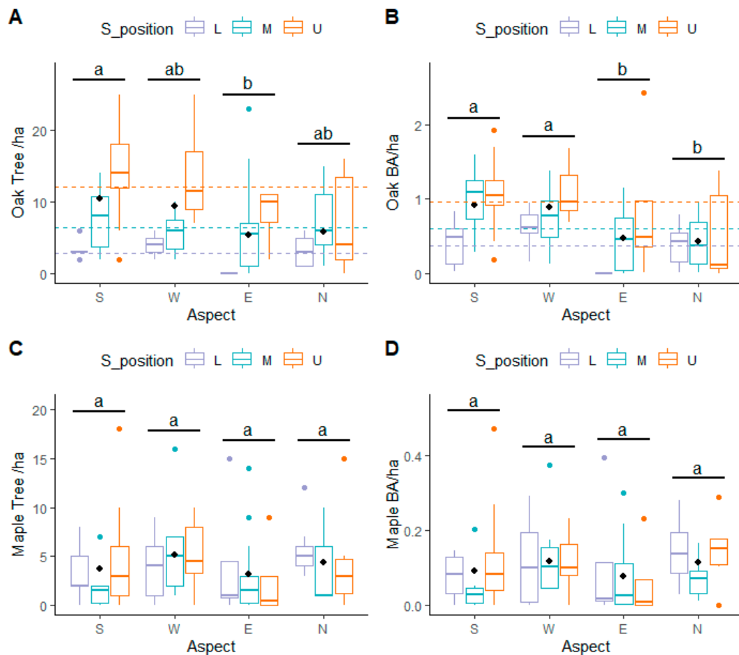
Figure 9. Oak and maple tree numbers per hectare and basal area of overstory at different aspects in three slope positions (L—lower, M—middle, U—upper). Specifically, (A) oak tree numbers/ha, (B) oak basal area ( m^2 /ha), (C) maple tree numbers/ha, and (D) maple basal area over aspects in three slope positions. Figures with the same lower-case letters are not different between aspects within each graph (post hoc Tukey–Kramer test, p = 0.05 ). Black diamonds represent group means for each aspect. Dashed lines represent group means for each slope position. S_position in legend means slope positions.
