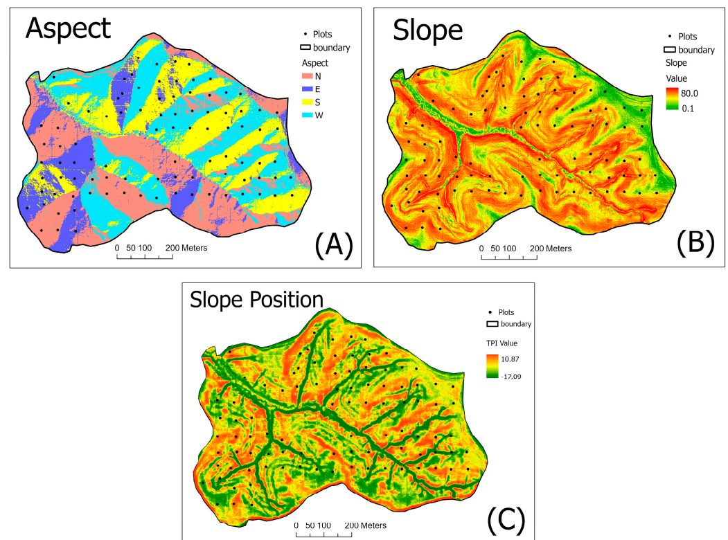
Figure 2. (A) Aspects, (B) slope degrees, and (C) slope position (Topographic Position Index, TPI) of the study site, Morgan Hollow. Total plots, n = 94 . Division by aspects, N = 22, E = 22, S = 24, W = 26. Division by slope position, upper = 37, middle = 36, lower = 21.
