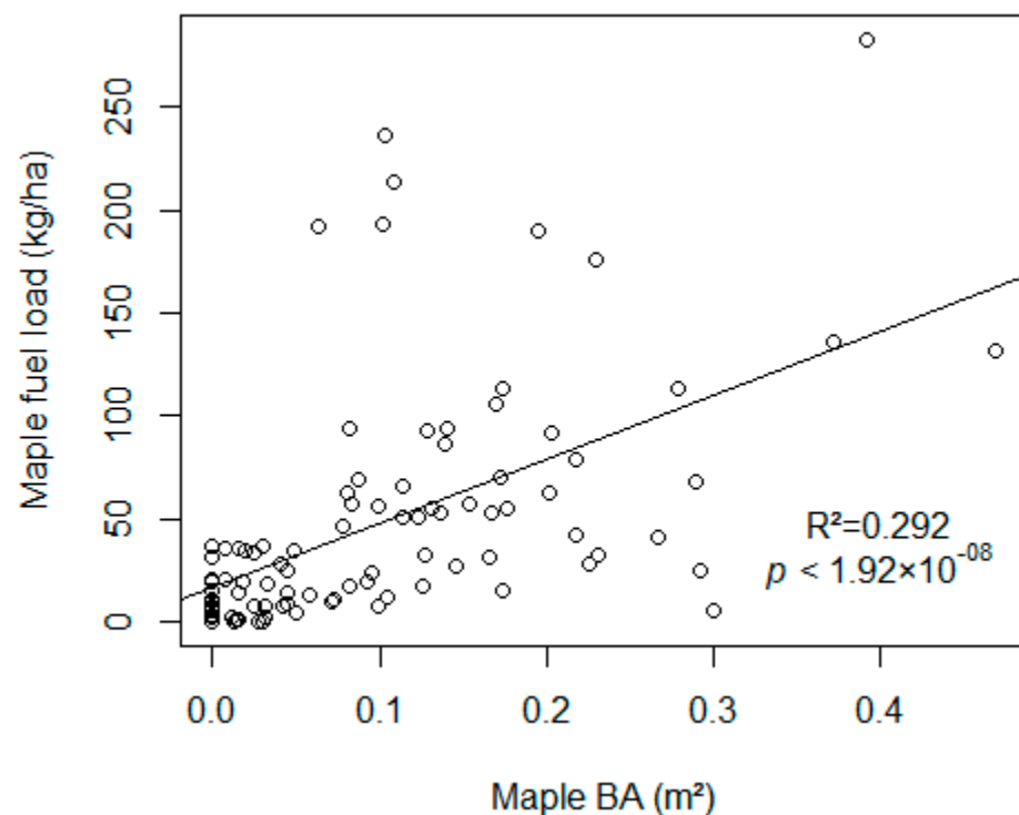
Figure 12. The linear regression between maple basal area (tree > 10 cm DBH) and maple litter fuel load (kg/ha).
