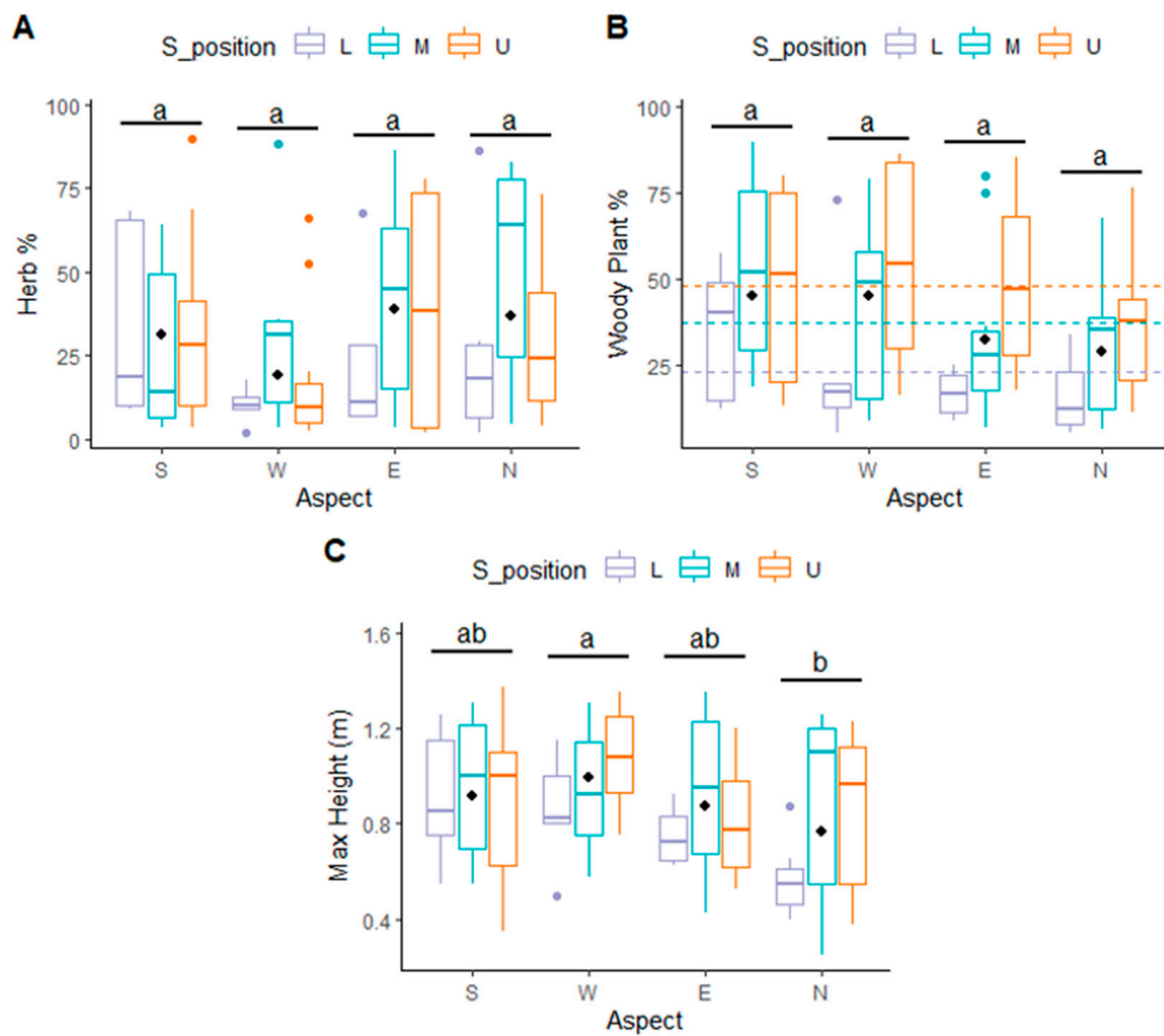
Figure 5. Shrub and regrowth layer attributes at different aspects in three slope positions (L—lower, M—middle, U—upper). Specifically, (A) herb coverage (%), (B) woody plant coverage (%), and (C) maximum shrub height (m) over aspects in three slope positions. Figures with the same lower-case letters are not different between aspects within each graph (post hoc Tukey–Kramer test, p = 0.05 ). Black diamonds represent group means for each aspect. Dashed lines represent group means for each slope position. S_position means slope positions.
