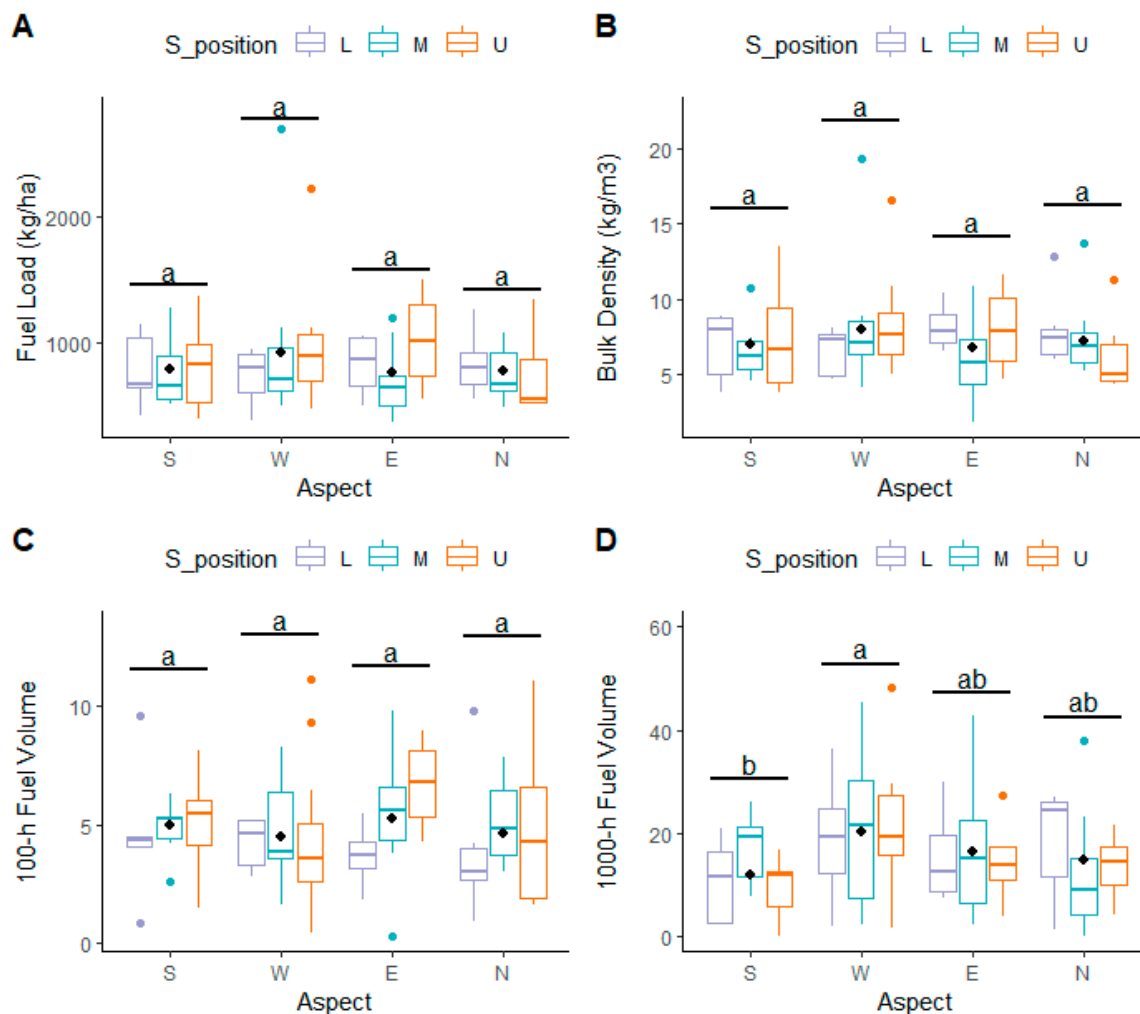
Figure 3. Surface fuel conditions at different aspects in three slope positions (L—lower, M—middle, U—upper). Specifically, (A) 1 h and 10 h fuel load (kg/ha), (B) 1 h and 10 h fuel bulk density (kg/m 3 ), (C) 100 h fuel volume (m 3 /ha), and (D) 1000 h fuel volume (m 3 /ha) over aspects in three slope positions. Figures with the same lower-case letters are not different between aspects within each graph (post hoc Tukey–Kramer test, p = 0.05 ). Black diamonds represent group means for each aspect. S_position means slope positions.
