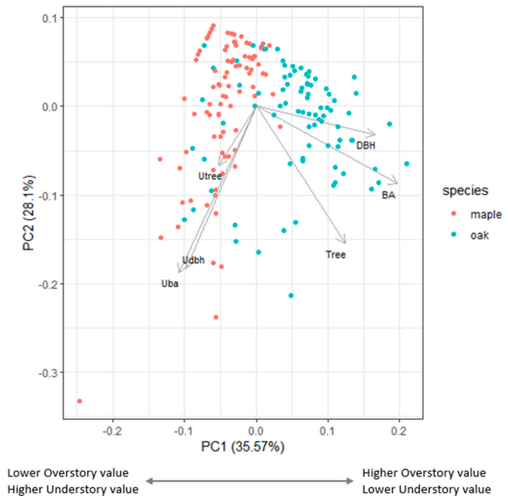
Figure 8. Biplot of principal component analysis (PCA) for overstory and understory oak and maple attributes. U—understory variables. Overstory values include DBH, trees/ha, and basal area. Understory values include U-DBH, U-trees/ha, and U-basal area.
