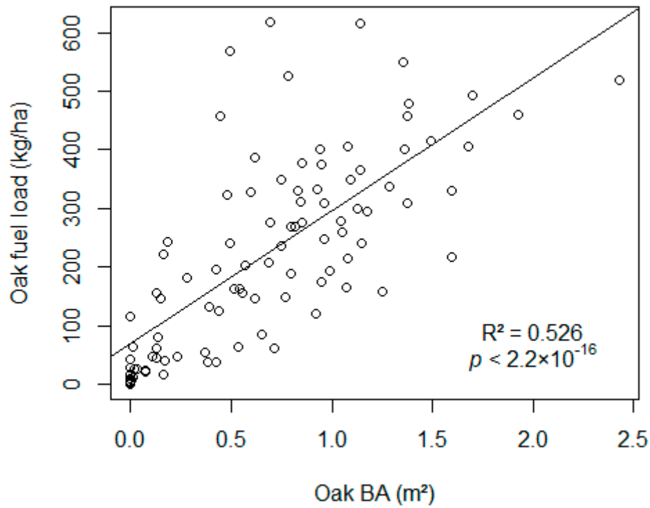
Figure 11. The linear regression between oak basal area (tree > 10 cm DBH) and oak litter fuel load (kg/ha).
