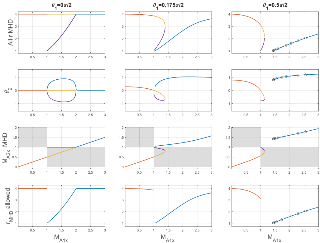
FIGURE 2. Upper row: density jump r for different angles \theta_1 in terms of M_{A1x} = M_{A1} / \cos \theta_1 , defined by (2.6). Sometimes there is more than 1 solution. Second row: angle \theta_2 of the field \mathbf{B}_2 with the x axis (see figure 1). Third row: evolutionarity criterion. Some branches, namely the ones crossing the shaded areas, are to be excluded. Lower row: same as upper row, but without the branches excluded by the evolutionarity criterion. There is now but 1 solution for a given M_{A1x} , or none. The black circles for \theta_1 = 0.5\pi/2 are the results of our MHD simulations (see § 3.1).
