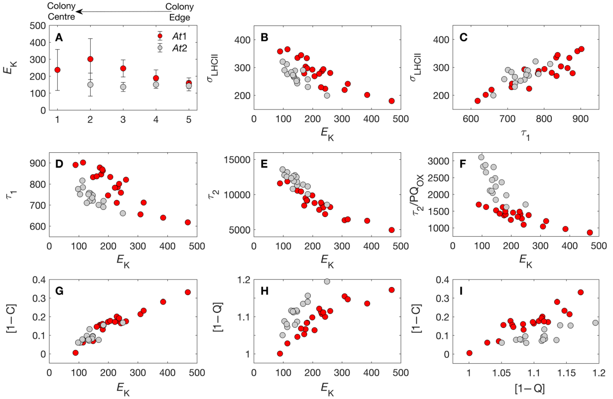
Fig. 3. LIFT-FRRf parameters retrieved from FLC protocols conducted across two different Acropora tenuis colonies (At 1 , At 2 ). Panel (A) shows the mean \pm standard deviation ( n = 4 ) light-saturation intensity for PSII photochemistry ( E_K , \mu\text{mol photons m}^{-2} \text{s}^{-1} ; 445 nm) for samples arbitrarily binned into positions sampled systematically from colony center to colony edge (as described in Supporting Information Fig. S2). Panels (B–I) compare LIFT-FRRf parameters for all samples collected across the coral surface for either colony: PSII effective cross section ( \sigma_{\text{LHCII}} , \text{\AA}^2 \text{quanta}^{-1} ; 445 + 505 nm) vs. (B) E_K , or vs. (C) the minimum electron turnover time Q_A to PQ ( \tau_1 , \mu\text{s} ); also, (D) \tau_1 , (E) \tau_2 (minimum time for PQ pool reoxidation; \mu\text{s} ), (F) \tau_2/\text{PQ}_{\text{OX}} (minimum downstream transfer of electrons from PQ to PSI; \mu\text{s} ), (G) extent of photochemical quenching ( [1 - C] , dimensionless), and (H) extent of non-photochemical quenching ( [1 - Q] , dimensionless), vs. E_K . Also shown is (I) [1 - C] vs. [1 - Q] . ANOVA for data in Panel (A) and linear regression equations and correlation coefficients for all comparisons (B–I) are given in Supporting Information Table S3.
