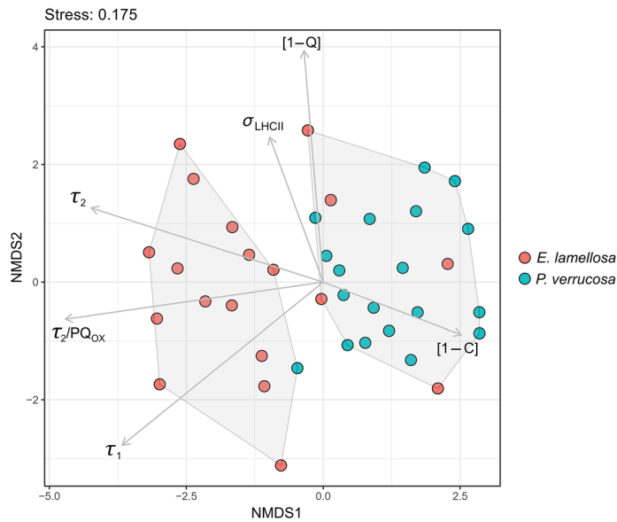
Fig. 8. NMDS based on how all LIFT-FRRf parameters—and in turn E_K —are optimized ( \sigma_{LHCII} , \tau_1 , \tau_2 , \tau_2/PQ_{OX} ) and dynamically regulated ( [1-C] , [1-Q] ) for all Echinopora lamellosa and Pocillopora verrucosa . Significance of individual parameters was assessed against an alpha value of 0.05 (see the main text).
