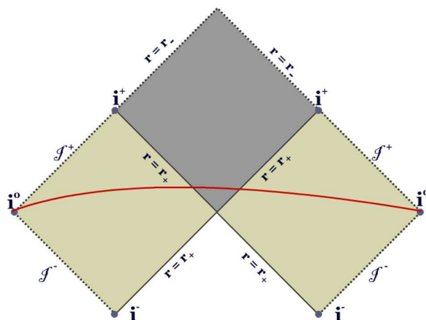
Figure 1: The Penrose diagram of Kerr for 0 < |a| < m .
