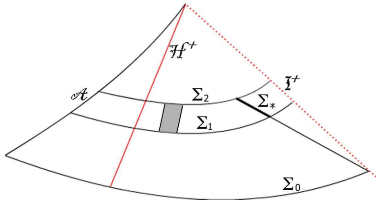
Figure 4: The spacetime region \mathcal{M}(\tau_1, \tau_2) = \mathcal{M} \cap \{\tau_1 \leq \tau \leq \tau_2\} between the spacelike hypersurfaces \Sigma_1 = \Sigma(\tau_1) and \Sigma_2 = \Sigma(\tau_2) , with the grey region denoting the trapped set.
