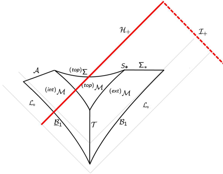
Figure 3: The GCM admissible space-time \mathcal{M}
