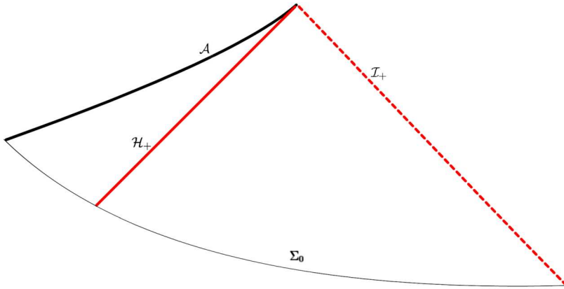
Figure 2: The Penrose diagram of the final space-time in the Main Theorem 1.2.
