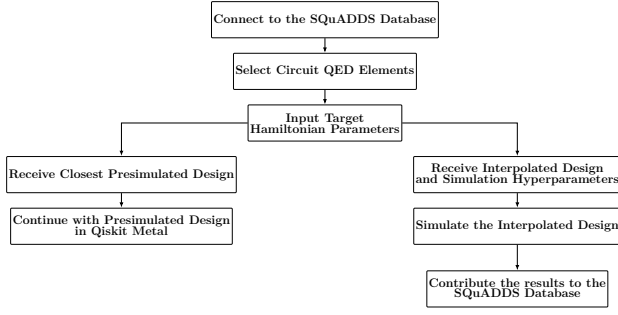
Figure 5: Process workflow of the SQuADDS database from a user perspective. The user selects a device type and target parameters, and optionally defines a cost function. SQuADDS searches the database for the closest pre-simulated design and experimentally validated design, and outputs these designs (and specified E_J values) and code to generate and simulate them. It also interpolates a best-guess design and gives the user code to generate and simulate it, along with estimated Hamiltonian parameters.
