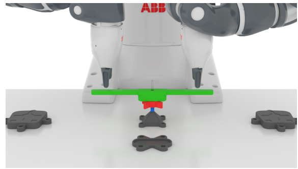
Figure 5: Potential solution: The spacer at the bottom (in blue), the gear in the middle (in red), and the propeller at the top (in green), all placed into the small metal shaft. There is no specific order of how the objects had to be placed.
