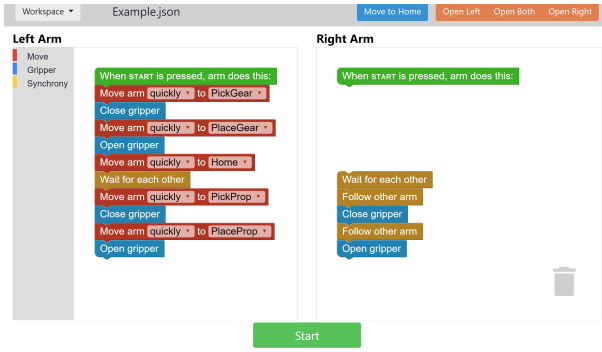
Figure 2: Interface of the Duplo programming language. Users can drag blocks from a toolbox on the left onto the programming canvases and attach them to existing blocks to create a program. Blocks that affect both arms are duplicated across canvases and vertically aligned.
