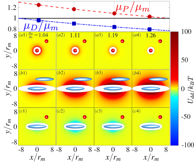
Figure 4: The induced dipole-dipole interaction energy with a fixed parallel orientation between (a) two paramagnetic spheres \tilde{r}^P = 1 , (b) two diamagnetic ellipsoids \tilde{r}_x^D/\tilde{r}_y^D = 5 , and (c) a paramagnetic sphere \tilde{r}^P = 1 and a diamagnetic ellipsoid \tilde{r}_x^D/\tilde{r}_y^D = 5 as a function of the separation distance between particles and the medium permeability \mu_m/\mu_0 . The pairwise dipolar interaction energy U_{dd} is in k_B T units. The magnetic field is directed perpendicular to the plane. The white region corresponds to the excluded volume between particles for the considered particle orientations.
