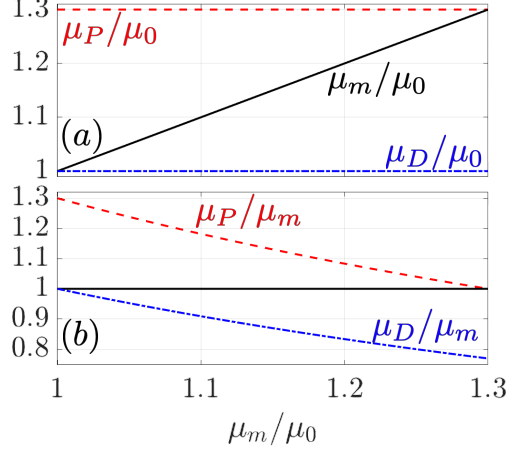
Figure 3: (a) Variation of medium permeability between the diamagnetic and paramagnetic permeabilities. (b) Relative permeabilities of the diamagnetic and paramagnetic particles with respect to the medium permeability.
