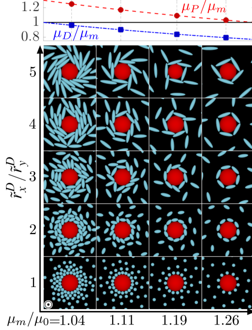
Figure 7: Snapshots of the Monte Carlo simulations of the directed assembly of binary systems composed of a paramagnetic sphere (red) with radius \tilde{r}^P = 5 and diamagnetic ellipsoids (cyan) with different aspect ratios \tilde{r}_x^D/\tilde{r}_y^D at \alpha_s = 10^4 .
