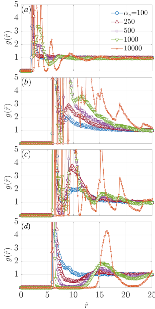
Figure 10: Radial distribution function g(\tilde{r}) between the central diamagnetic particle and surrounding paramagnetic particles for different dipole-field interaction parameters \alpha_s . (a) A central diamagnetic ellipsoid ( \tilde{r}_x^D/\tilde{r}_y^D = 6 ) and satellite paramagnetic spheres ( \tilde{r}^P = 1 ) at \mu_m/\mu_0 = 1.11 , (b) – (d) a central paramagnetic sphere ( \tilde{r}^P = 5 ) and satellite diamagnetic ellipsoids ( \tilde{r}_x^D/\tilde{r}_y^D = 4 ) at (b) \mu_m/\mu_0 = 1.04 , (c) \mu_m/\mu_0 = 1.11 , and (d) \mu_m/\mu_0 = 1.26 .
