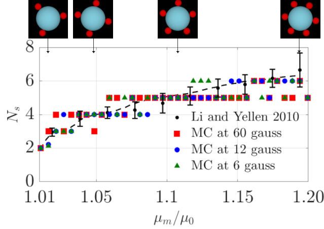
Figure 5: Average number N_s of paramagnetic spheres in the binary structure as a function of medium permeability. The dashed line and the black dots correspond to the reported experimental results from Ref. [Li and Yellen(2010)]. The colored dots represent the results from Monte Carlo (MC) simulations at different magnetic fields. Renderings are shown at the top with the diamagnetic particle (cyan) and the surrounding paramagnetic particles (red) for different medium permeabilities.
