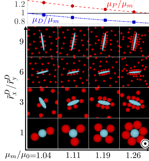
Figure 6: Snapshots of the Monte Carlo simulations of the directed assembly of binary systems composed of a central diamagnetic ellipsoid with different aspect ratios ( \tilde{r}_x^D/\tilde{r}_y^D ) surrounded by paramagnetic spheres ( \tilde{r}^P = 1 ) at \alpha_s = 10^4 . The representative assembled structures are presented as a function of the relative medium permeability.
