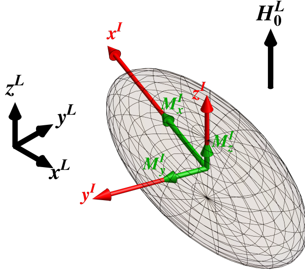
Figure 1: Schematic representation of a magnetizable ellipsoidal particle I with an arbitrary position and orientation with respect to the laboratory coordinates (x^L, y^L, z^L) , represented in black. The particle coordinate system (x^I, y^I, z^I) , in red, is attached to the principal semi-axes of the particle. \mathbf{H}_0^L is the uniform applied field directed along the z^L -axis of the laboratory coordinates. The components (M_x^I, M_y^I, M_z^I) of the induced particle magnetization \mathbf{M}^I are represented in green along the main axes of the particle.
