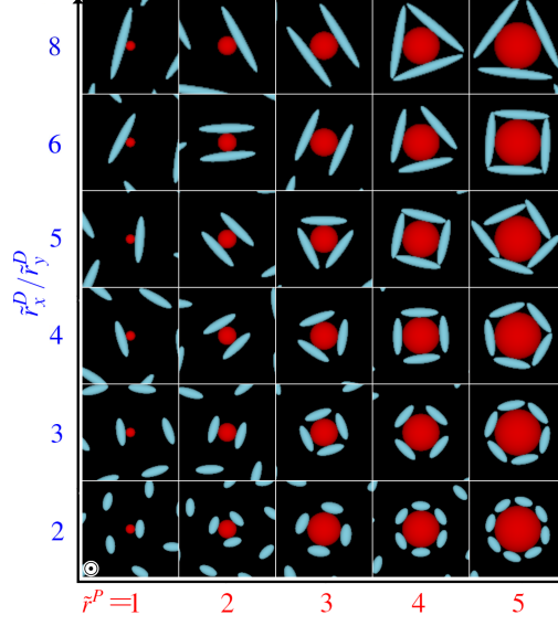
Figure 9: Snapshots of the Monte Carlo simulations of the directed assembly of binary suspensions composed of a paramagnetic sphere (red) with radius \tilde{r}^P and diamagnetic ellipsoids (cyan) with different aspect ratios \tilde{r}_x^D/\tilde{r}_y^D at \alpha_s = 10^4 and \mu_m/\mu_0 = 1.26 .
