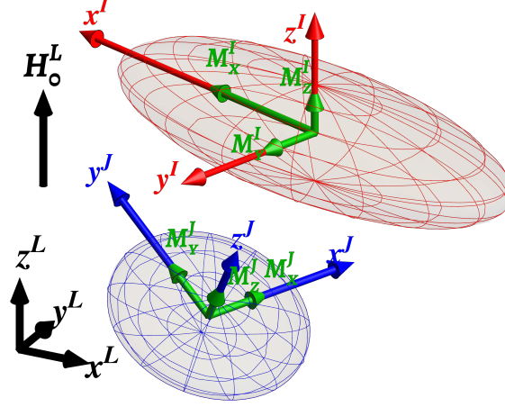
Figure 2: Schematic representations of two interacting magnetizable ellipsoidal particles under the influence of a uniform magnetic field \mathbf{H}_0^L . Both particles are arbitrarily positioned and oriented with respect to the laboratory coordinates. The red coordinate system (x^I, y^I, z^I) is attached to the principal semi-axes of particle I , while the blue coordinate system (x^J, y^J, z^J) is attached to the principal semi-axes of particle J . The components of the induced particle magnetization are represented in green along the main axes of each particle.
