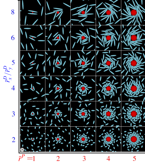
Figure 8: Snapshots of the Monte Carlo simulations of the directed assembly of binary suspensions composed of a paramagnetic sphere (red) with radius \tilde{r}^P and diamagnetic ellipsoids (cyan) with different aspect ratios \tilde{r}_x^D/\tilde{r}_y^D at \alpha_s = 10^4 and \mu_m/\mu_0 = 1.04 .
