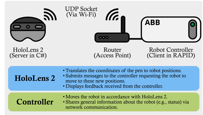
Figure 4: Pen-robot synchronization system description.
