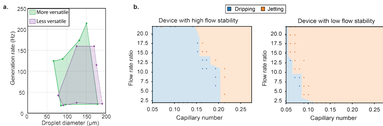
Fig. 7. Generalization of versatility and stability to novel fluid combinations (LB media and mineral oil). (a.) Using the droplet generators from Figure 4, differences in versatility were still apparent between the more and less versatile devices. (b.) With the droplet generators from Figure 5, a marked shift in regime change boundary was observed in both devices. However, relative stability in the dripping regime between the more and less stable devices.
