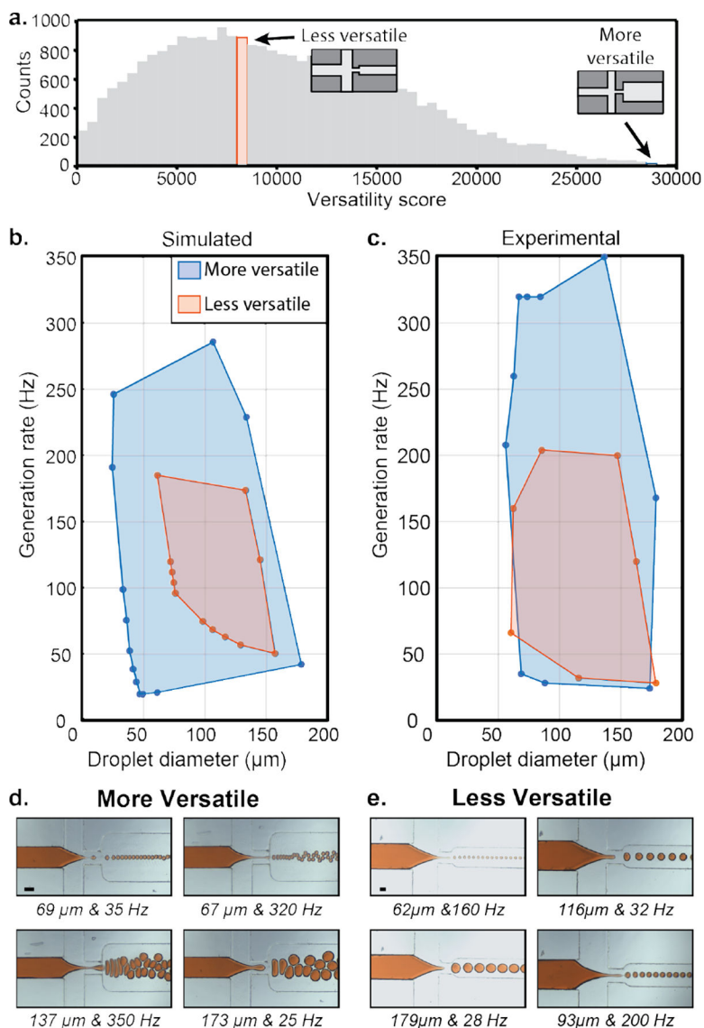
Fig. 4. Direct comparison of versatile and non-versatile droplet generators. (a.) Two droplet generators capable of generating 100 \mu\text{m} diameter droplets at 100 Hz but drastically different versatility scores in the dripping regime and device geometry were manually selected. (b.) The predicted performance range of the more versatile design fully encompassed the deliverable performance range of the less versatile design. (c.) The more versatile design delivered an experimentally observed performance convex hull area approximately two times larger than the less versatile design while almost completely encompassing its performance space in the dripping regime. (d.-e.) Images of experimental results.
