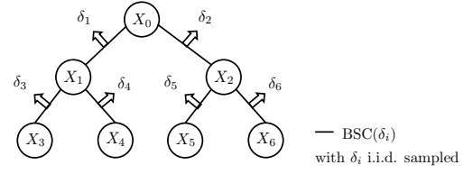
(a) Crossover probabilities being i.i.d. random and known to the estimator.
