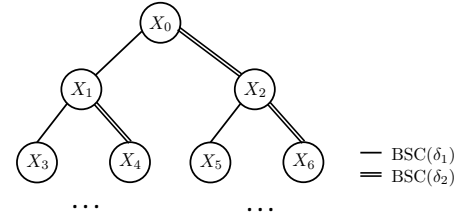
(c) Nonisotropic, i.e., each vertex is connected through a fixed list of channels, each with distinct crossover probabilities.
