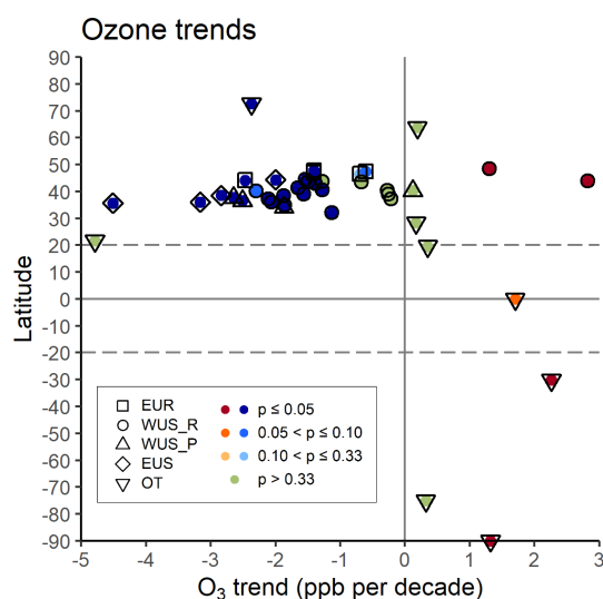
Figure 2. Decadal \text{O}_3 trends (50th percentile) for the 41 high-elevation sites used in this study. The reference periods for trend calculation for the different sites are listed in Table 1. Trends are ordered by latitude (y axis), and the colors indicate the sign and p value on the trend, with blue shades for negative trends ( p \leq 0.33 ), red shades for positive trends ( p \leq 0.33 ), and green shades for trends of either sign ( p > 0.33 ). The shapes identify the different regions, i.e., EUR – Europe, WUS_R – western US “rural”, WUS_P – western US “polluted”, EUS – eastern US, OT – other.
