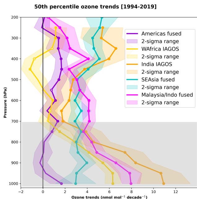
Figure 6. Vertical profiles of ozone trends ( \text{nmol mol}^{-1} \text{ decade}^{-1} ) between 1994 and 2019 at 50 hPa vertical resolution. Trends are calculated for the five IAGOS regions in the tropics: the Americas, western Africa, India, Southeast Asia, and Malaysia and Indonesia. SHADOZ data are available for three out of the five IAGOS regions and used to produce fused trends (IAGOS + SHADOZ). Filled circles indicate trends with p values less than 0.05. Open circles indicate trends with p values between 0.05 and 0.1. The zero-trend value is indicated with a vertical black line. The vertical range below 700 hPa is shaded gray to indicate that the fused trends are based on several sites and airports influenced by different local air masses. The 2\sigma values associated with the ozone trends are shown in shaded colors.
