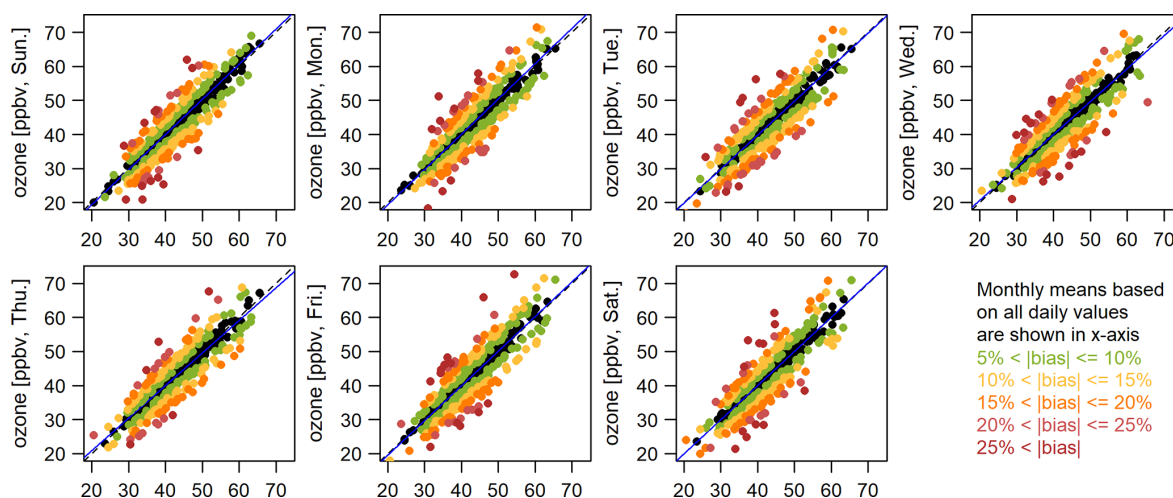
Figure 3. Demonstration of exceedance bias (at different thresholds) from once-per-week samples in monthly means: panels show the scatterplots between monthly means based on full sampling (x axis) and once-per-week sampling (y axis, by each day of the week). The result are based on daily nighttime observations measured at MLO (1980–2021). The solid blue line in each panel is the 1 : 1 line, and the dashed blue line represents the overall correlation.
