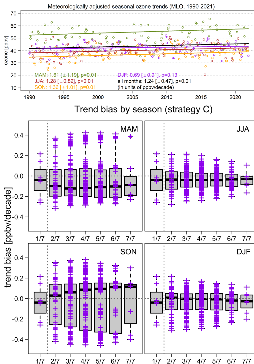
Figure 7. MLO ozone seasonal trends under full sampling (upper panel) and seasonal trend bias (each cross represents the difference between a subsampled trend and the true trend, with meteorological adjustments – lower panel) under mixed sampling (1990–2021, strategy C): 1/7 indicates the baseline scenario representing once-per-week sampling for all months, and k/7 ( k = 2, \dots, 7 ) indicates x samples per week for a particular season, while the other seasons remain at once-per-week sampling.
