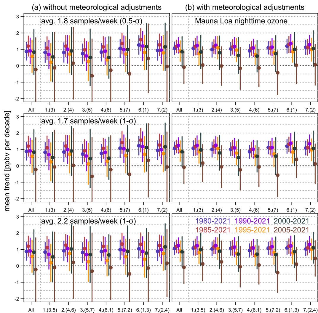
Figure 10. Same as Fig. 5, but the anomaly-based sampling strategy is incorporated. From top to bottom: the 1(+1) : 0.5 \sigma , 1(+1) : 1 \sigma , and 1(+2) : 1 \sigma schemes. Numbers in parentheses in the x axis indicate the extra sampling days of the week.
