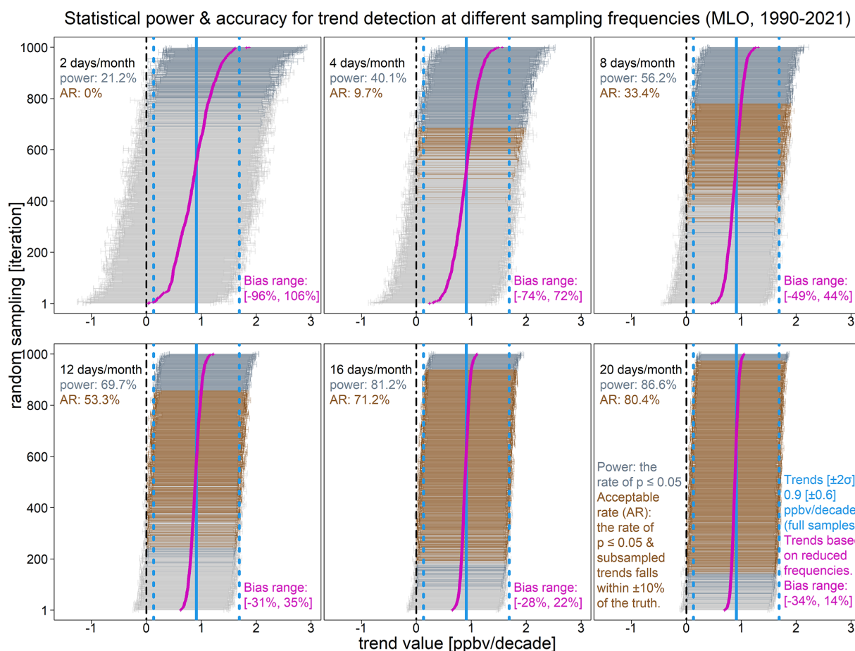
Figure 6. Statistical power and accuracy for trend detection: this figure illustrates how trend values can become noisy and uncertain when the data set is thinned from full sampling (every day of the month) to 2, 4, 8, 12, 16, and 20 samples per month. The vertical blue lines represent the 1990–2021 ozone trend based on the full record (without meteorological adjustments), with the solid line being the mean trend value and the dashed lines representing the 2\sigma interval. For each panel, subsamples are generated randomly and independently over 1000 iterations, and resulting subsampled trends are sorted along the y axis from the lowest to the highest values (purple line – the lowest and highest values are indicated in the bias range); each horizontal line indicates the 2\sigma interval. Subsampled trends with p values \leq 0.05 (dark gray and orange) are summarized by statistical power. Subsampled trends with p values \leq 0.05 and within \pm 10\% bias (orange) are summarized by the acceptable rate.
