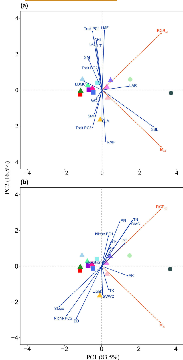
FIGURE 2 Ordination plot of species growth and mortality (PC1 and PC2) with respect to functional traits and ecological niches based on a linear model for seedlings of 14 species in the Xishuangbanna forest dynamics plot, China. The linear regression analysis finds the direction in the growth–mortality ordination space that has maximal correlation with the driver variables (Jongman et al., 1995), which in our case are the functional traits (a) and ecological niche variables (b). The direction and length of the vectors for each trait and niche variable were determined by the envfit function in the vegan package (Oksanen et al., 2011), indicating the direction of the gradient and the strength of the correlation, respectively. The interspecific growth–mortality relationship (PC1) was estimated based on the species' 90 th quantile of relative growth rate in height ( RGR_{90} ) and the mortality rate of the 30% slowest growing individuals ( M_{30} ) for each species. See Table S2 for species information and Table 1 for information about functional traits and ecological niche variables. Symbol colours and shapes match those in Figure 1.
