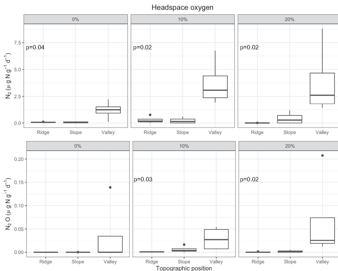
Figure 2. Dinitrogen and nitrous oxide emissions from ridge, slope, and valley positions (macrotopography) near the El Verde Field Station measured at 0%, 10%, and 20% headspace O_2 .
