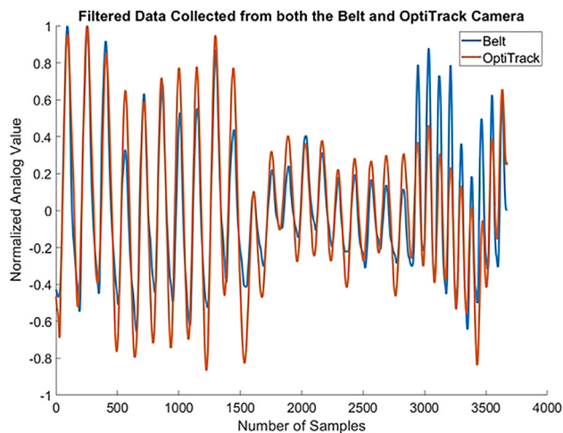
Figure 5. Filtered data collected from belt and camera
