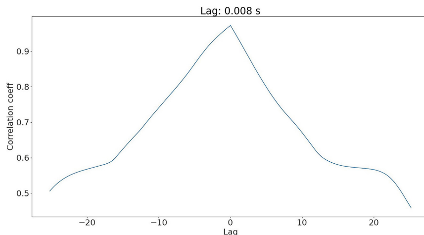
Figure 6. Cross-correlation between respiration rate computed using the belt and camera data
