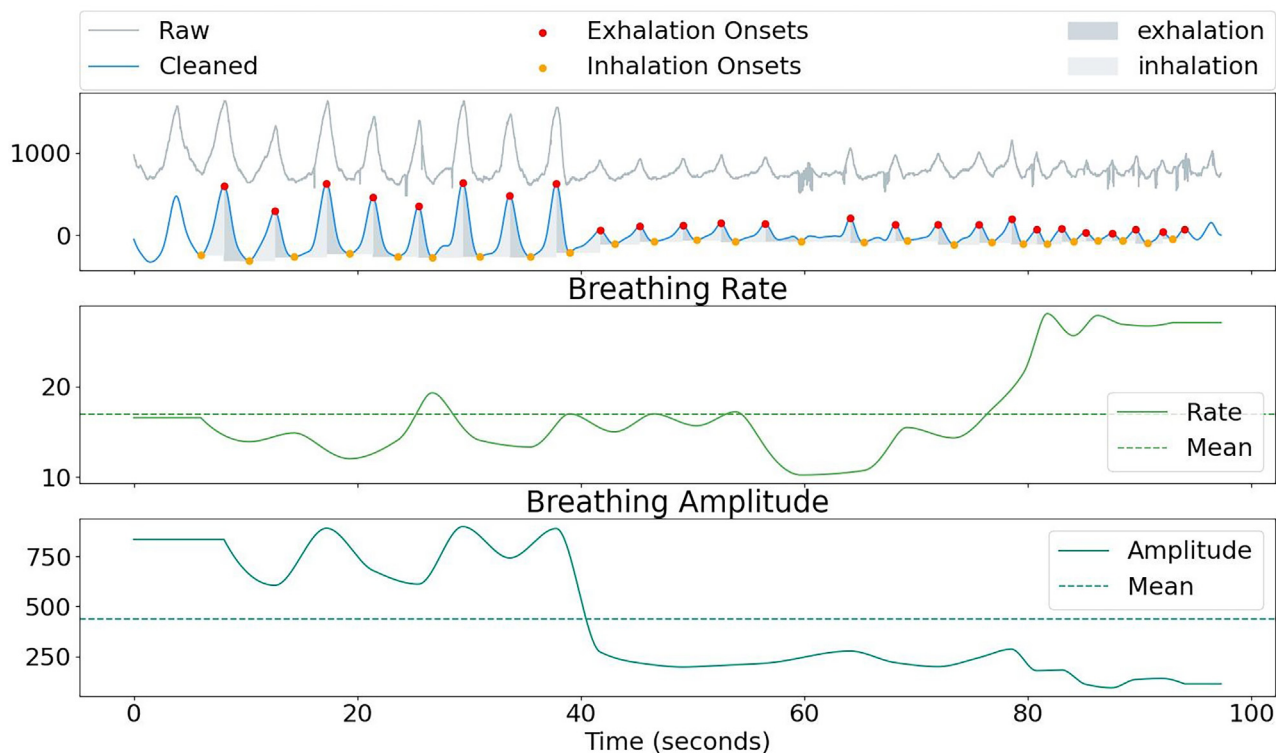
Figure 4. Raw data, filtered data, breathing rate, and breathing amplitude of the data collected from the belt during standing
