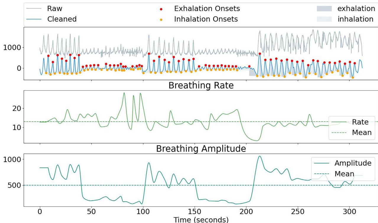
Figure 3. Raw data, filtered data, breathing rate, and breathing amplitude of the data collected from the belt
