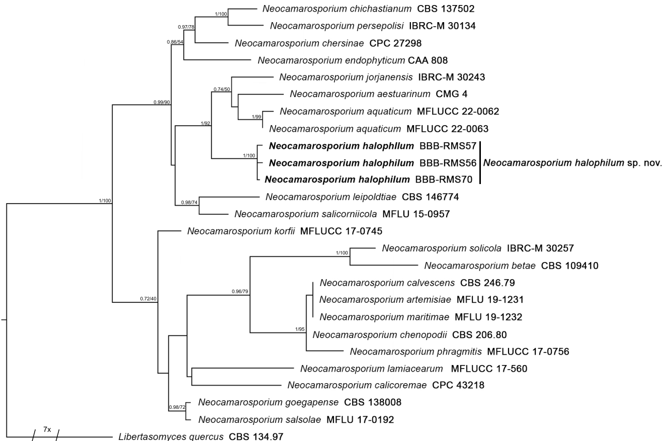
FP1579-2 Phylogenetic tree of Neocamarosporium species inferred from a concatenated dataset: ITS (536 bp) + LSU (850 bp), using MrBayes v. 3.2.7 (Ronquist et al. 2012) with Libertasomyces quercus CBS 134.97 as outgroup. Bayesian posterior probability (BPP) and maximum likelihood Bootstrap support (BS) values above 0.7 and 50 %, respectively, are shown at the nodes. Bootstrap support values have been calculated based on 1000 replicates under maximum likelihood using IQ-TREE v. 2.1.3 (Minh et al. 2020). A supplementary table (FP1579-1) with the GenBank accession numbers of the sequences used is provided. The trees and alignment were deposited at figshare.com (doi: 10.6084/m9.figshare.24212298).
