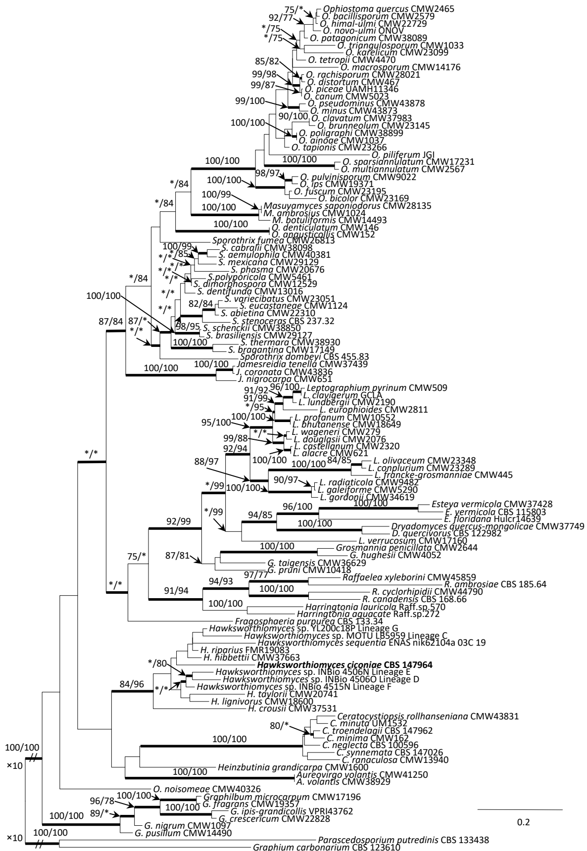
FP1567-1 Phylogram from Maximum Likelihood (ML) analyses of the combined datasets of ITS and LSU for the members of the Ophiostomatales order carried out with PhyML v. 3.0 (Guindon et al. 2010) using the GTR+I+G model. Maximum Parsimony (MP) analyses were performed using PAUP v. 4.0b10 (Swofford 2003) while Bayesian Inference (BI) analyses using Markov Chain Monte Carlo (MCMC) methods were carried out with MrBayes v. 3.1.2 (Ronquist & Huelsenbeck 2003). The novel species is shown in bold face . The bootstrap support values ( \geq 75\% for ML and MP analyses) are presented at nodes as follows: ML/MP. Bold branches indicate posterior probabilities \geq 0.95 obtained from BI analyses. * Indicates bootstrap support values < 75\% . The tree is drawn to scale (see bar) with branch lengths indicating the expected number of substitutions per site. Graphium carbonarium and Parascedosporium putredinis were used as outgroup taxon. The alignment and tree are available in TreeBASE (study ID: S30522).
