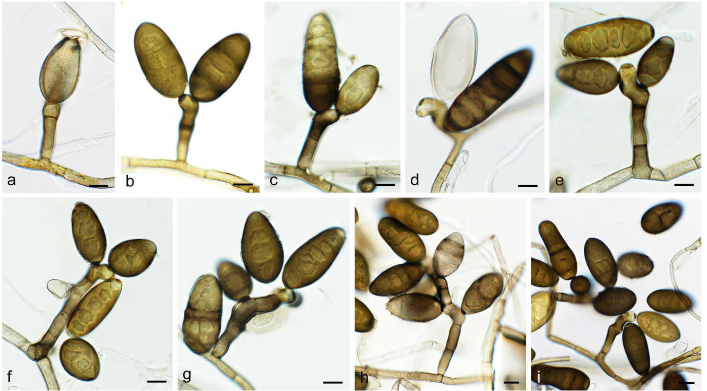
FP1597-2 Conidiophores and conidia of Alternaria iridis (CBS 226.66). Scale bars = 10 μm.
