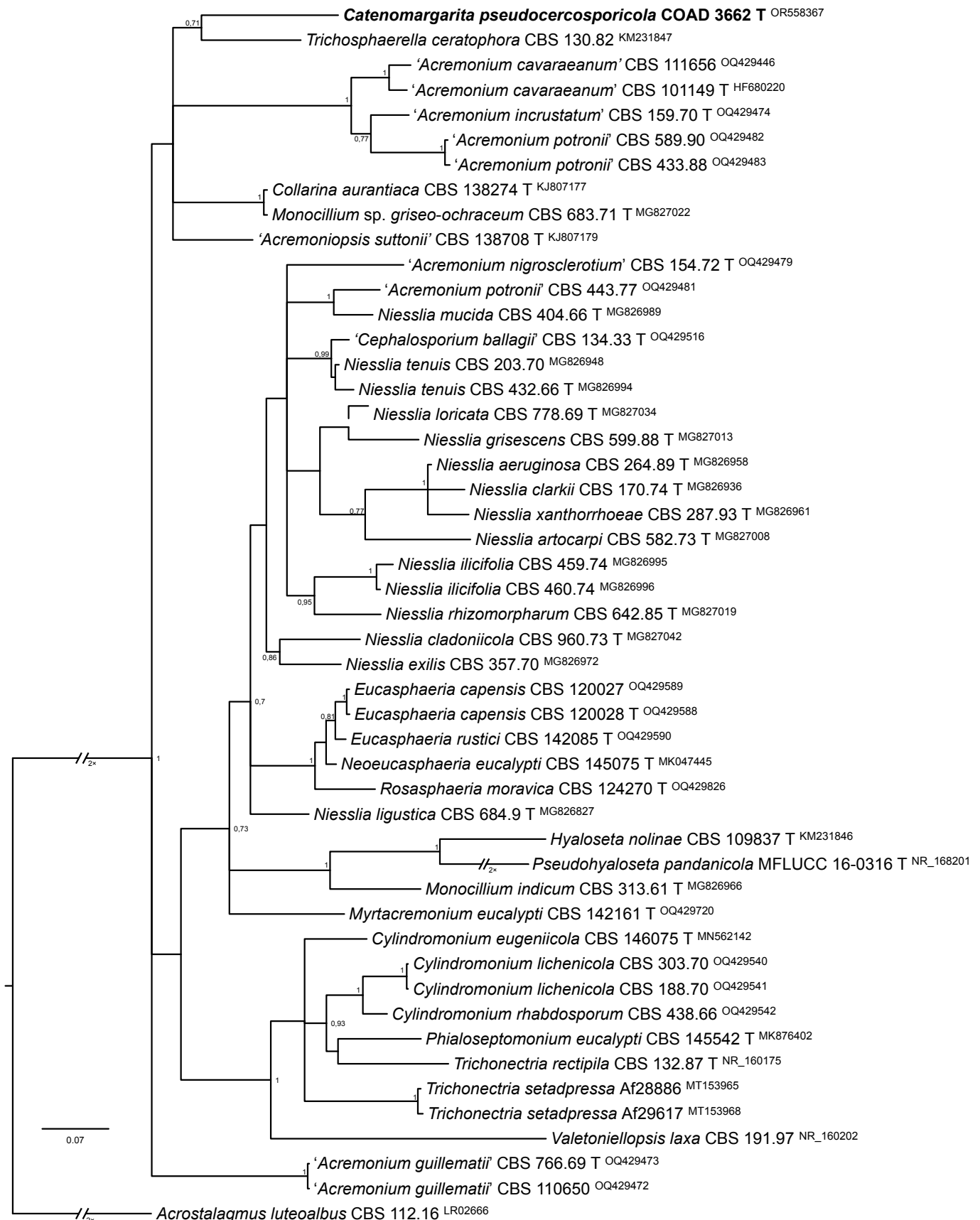
FP1556 Bayesian inference tree obtained by phylogenetic analyses of ITS sequences conducted in MrBayes v. 3.2.7a on XSEDE in the CIPRES science gateway. Bayesian posterior probability values above 0.70 are indicated at the nodes. Strains with a type status are indicated with a 'T'. The new species is indicated in bold face. Acrostalagmus luteoalbus (CBS 112.16) was used as outgroup. The alignment and tree were deposited at figshare.com (doi: 10.6084/m9.figshare.24146700).
