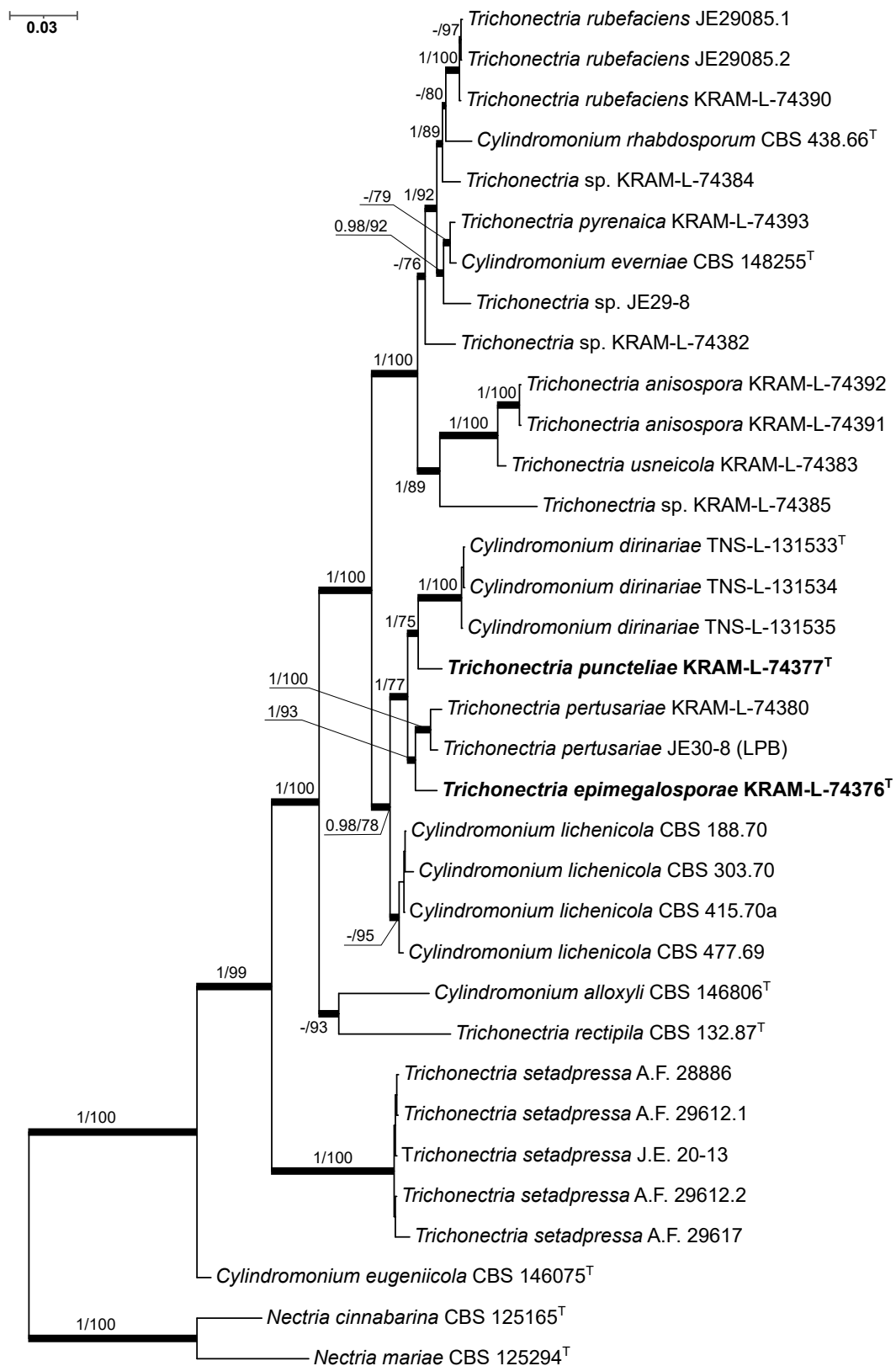
FP1589 & FP1590-2 Phylogenetic relationships of Trichonectria epimegalosporae and T. puncteliae (in bold ), Cyindromonium and Trichonectria species inferred from a Bayesian Inference analysis (BI) of a combined ITS, LSU, SSU, tef1 and rpb1 dataset. Nectria cinnabarina and Nectria mariae were used as the outgroup. Thickened branches represent either Bayesian posterior probabilities \geq 0.97 and/or bootstrap support values \geq 75\% . PartitionFinder2 was used to select the best partition for our data and substitution models (Lanfear et al. 2016). A single substitution model was selected for each region (GTR+G for ITS1 and ITS2, TRNEF+I+G for 5.8S and LSU, JC for SSU, F81+I+G for tef1 , TIM+I for rpb1 ) under a greedy search algorithm and the Akaike information criterion (AIC) (Lanfear et al. 2012). Maximum likelihood (ML) and BI analyses were performed on the concatenated dataset using substitution models obtained from PartitionFinder 2. Maximum likelihood analyses were carried out using a heuristic search as implemented in IQ-TREE v. 2.1.2 on XSEDE and 100 bootstrap interactions on 1000 replicates to estimate branch support. Bayesian inference of the phylogenetic relationships was calculated using the Markov chain Monte Carlo (MCMC) approach as implemented in MrBayes v. 3.2.6 on XSEDE (Ronquist et al. 2012) using the partitions and substitution models obtained by PartitionFinder2. Two independent parallel runs were started each with four incrementally heated (0.15) chains. This MCMC was allowed to run for 100 M generations, sampling every 1000th tree and discarding the first 50 % of the sampled tree as a burn-in factor. The analysis was stopped after 1 M generations when the standard deviation of split frequencies had dropped below 0.01. Voucher data and GenBank accession numbers of sequences, the alignment and tree were deposited at figshare.com (doi: 10.6084/m9.figshare.24114249 and 10.6084/m9.figshare.24114252 ).
