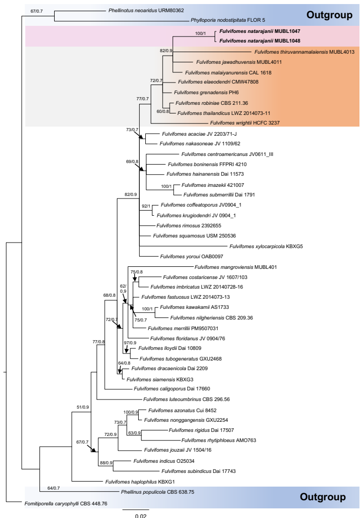
FP1565-2 Phylogenetic tree inferred from LSU sequences of Fulvifomes natarajanii (MUBL1047 and MUBL1048) and related species rooted with Fomitiporella caryophylli (CBS 448.76) and Phellinotus neoaridus (URM80362). The maximum likelihood analysis was performed using MEGA v. X (Kumar et al. 2018) and the same data were used for Bayesian analysis using MrBayes v. 3.2.7 (Ronquist et al. 2012). Branches are labelled with maximum likelihood bootstrap support and Bayesian posterior probabilities values. Novel species are in bold . The alignment and tree are available from TreeBASE (study ID: S30227).
