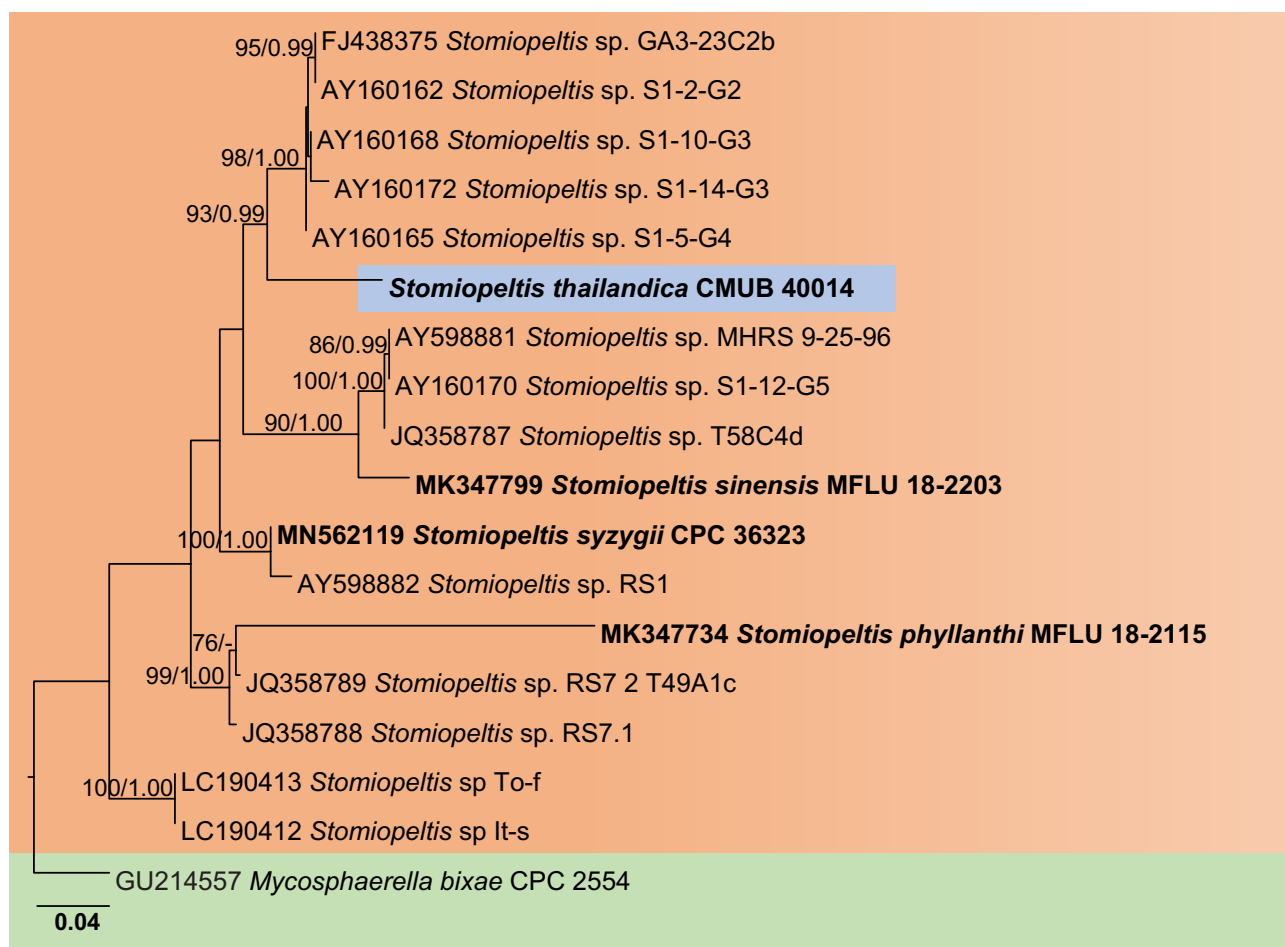
FP1587-2 Phylogenetic analysis of Stomiopeltis thailandica sp. nov. inferred from a maximum likelihood (ML) analysis of ITS/LSU sequences. The analysis was performed with RAxML v. 8.2.12 (Stamatakis 2014) using the rapid bootstrapping and search algorithm, with GTR+GAMMA nucleotide substitution model, and 1000 bootstrap replicates. Bayesian Inference (BI) approaches under MrBayes v. 3.2.6 (Ronquist et al. 2012). Bootstrap support values for ML greater than 75 % and Bayesian posterior probabilities greater than 0.95 are indicated at the nodes. The tree is rooted with Mycosphaerella bixae (CPC 2554). Ex-type strains are in bold . The novel species is indicated in a blue box. Scale bar on the tree indicates the expected number of changes per site. The matrix and the resulting tree have been deposited at TreeBASE (study ID; S30728).
