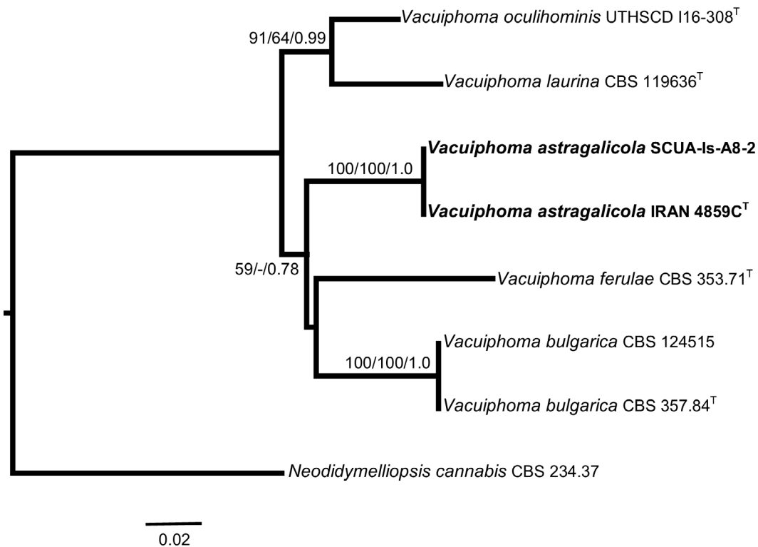
FP1592-2 RAxML phylogenetic tree constructed from a maximum likelihood analysis based on the combined ITS, tub2 and rpb2 sequences of Vacuiphoma species. The tree was rooted to Neodidymelliopsis cannabis CBS 234.37. Bootstrap support values (MLBS, MPBS, respectively) obtained in maximum likelihood (ML, GTR + G + I) and maximum parsimony (MP) analyses > 50 % and Bayesian posterior probability values (BPP) ≥ 0.5 are shown at the nodes, respectively. (ML: raxmlGUI v. 2.0 beta; Edler et al. 2019; MP: MEGA v. 7; Tamura et al. 2013; BI: jModelTest2 and MrBayes v. 3.2.6; Darriba et al. 2012, Ronquist et al. 2012). Taxa retrieved newly from Iran are shown in bold . The trees and alignment were deposited in XXfigshare/TreeBASE/Zenodo/etcXX.
