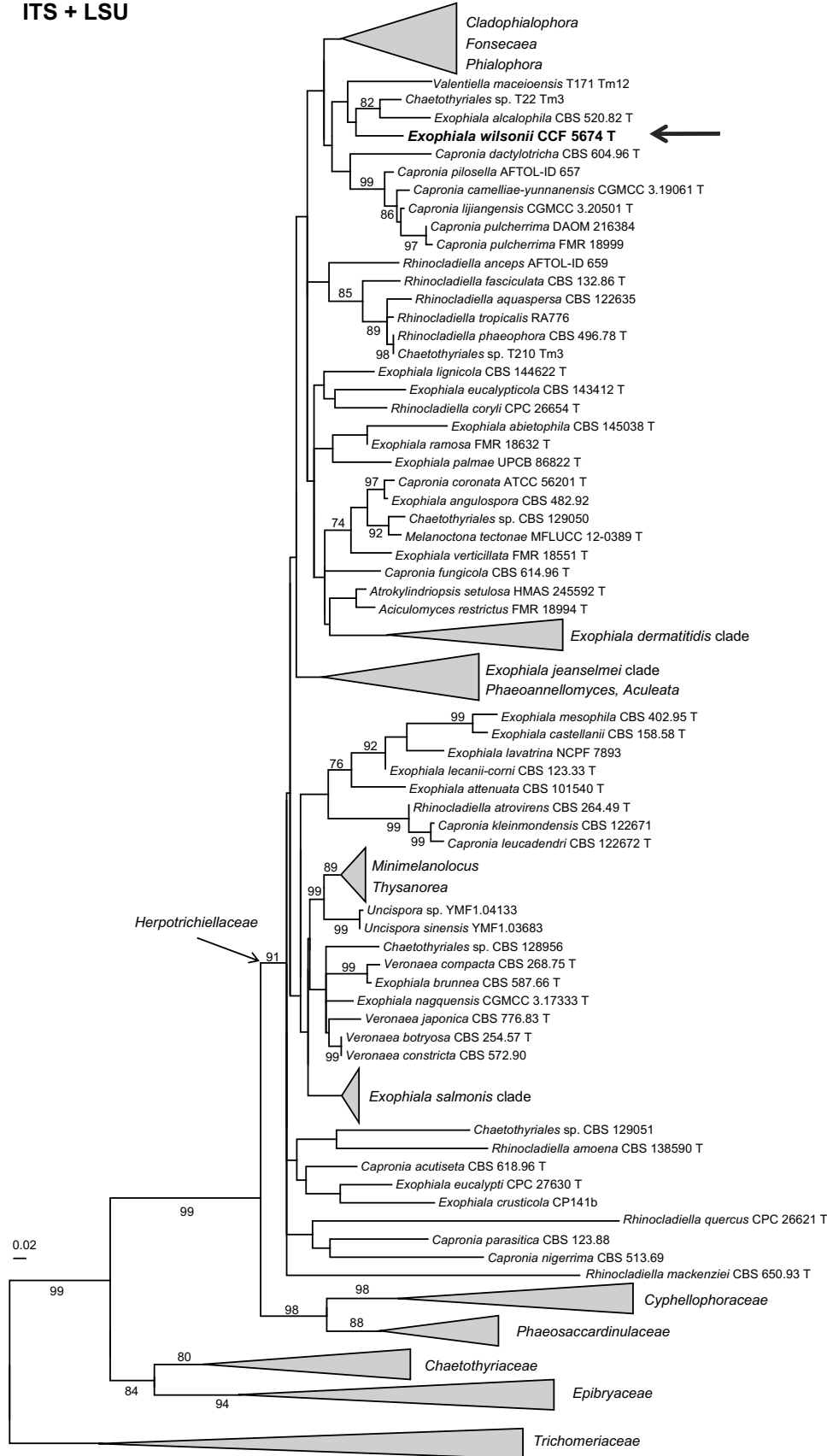
FP1563 A maximum likelihood (ML) tree based on the combined ITS and LSU regions shows the relationships of Exophiala wilsonii with other species and genera in the family Herpotrichiellaceae . The dataset published by Torres-Garcia et al. (2023) was used for the preparation of ITS and LSU alignments (accession numbers to DNA sequences can be found in the same publication). The combined alignment included 191 taxa and a total of 1615 characters of which 941 were variable. For the ML analysis, the GTR+G+I model was selected as the best substitution model for ITS and the K2+G+I model for LSU. The tree was constructed with MEGA v. 6.0 (Tamura et al. 2013). Support values at branches were obtained from 1000 bootstrap replicates. Only support values \geq 70\% are shown; ex-type strains are indicated by letter T. Some nodes were collapsed to facilitate layout; novel species is indicated in bold font and an arrow. The tree was rooted with a clade containing the family Trichomeriaceae .
