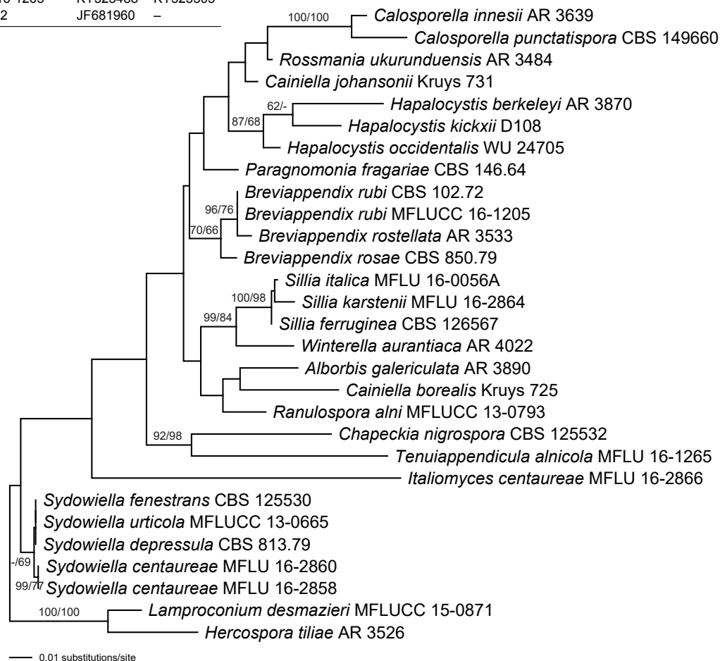
FP1555-2 Maximum likelihood tree revealed by raxmlGUI v. 2.0 (Silvestro & Michalak 2012) from an analysis of the ITS-LSU rDNA matrix, showing the position of Calosporella punctatispora within Sydowiellaceae , with ML/MP bootstrap support values at branches. Maximum parsimony (MP) bootstrap analysis was performed with PAUP v. 4.0a169 (Swofford 2002), with 1000 bootstrap replicates using ten rounds of heuristic search replicates with random addition of sequences and subsequent TBR branch swapping. The tree was rooted with Lamproconiaceae . The trees and alignment were deposited in TreeBASE ( https://purl.org/phylo/treebase/phyloids/study/TB2:S30799 ).
