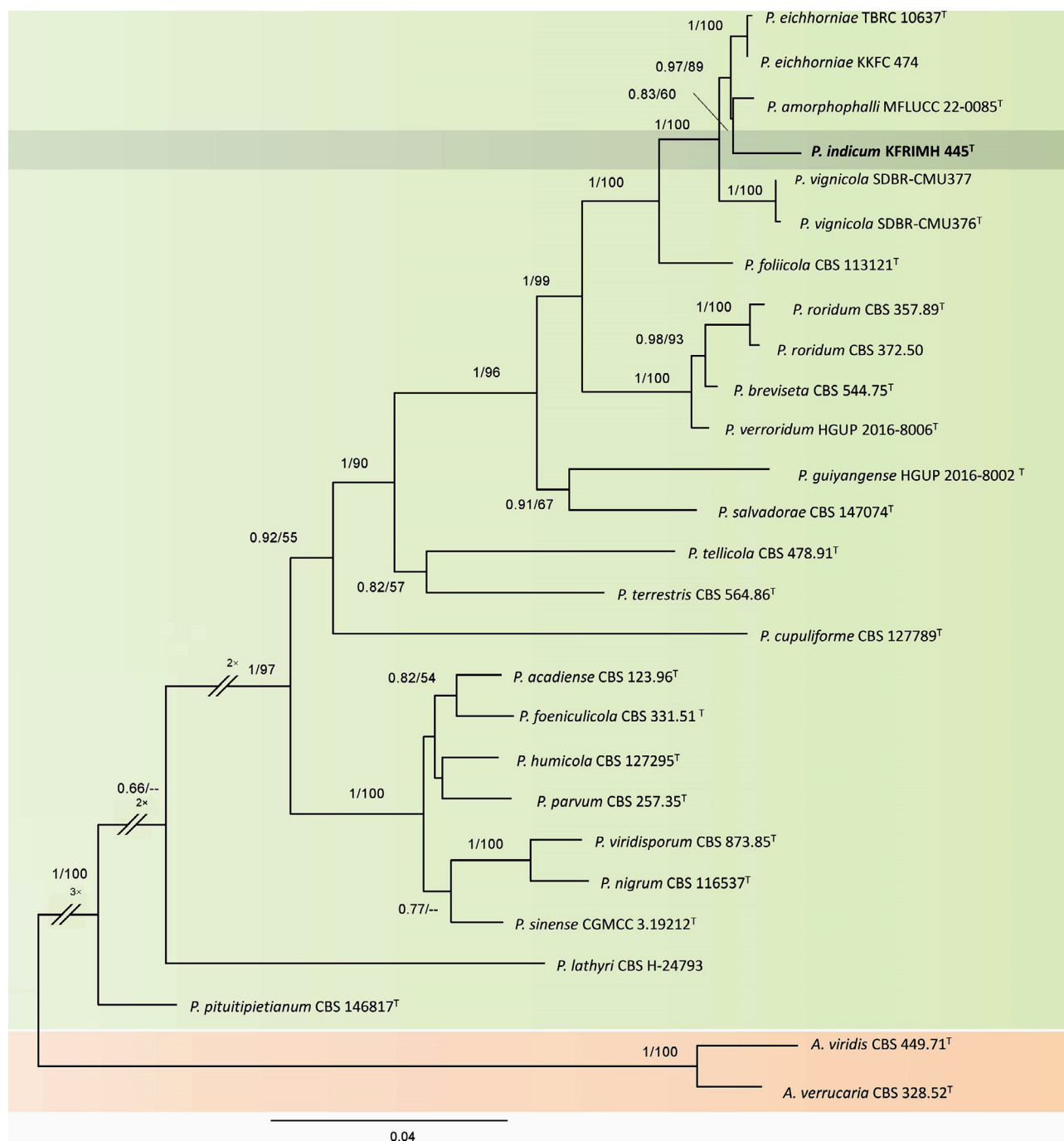
FP1584-1 Phylogenetic tree resulting from a RAxML v. 8 (Stamatakis 2014) analysis based on a five-locus alignment (ITS, LSU, cmdA , tub2 and rpb2 ) representing Paramyrothecium indicum (KFRIMH 445) and related species. The Bayesian posterior probabilities ( \geq 0.50 ; BI-PP) (Rannala & Yang 1996, Ronquist et al. 2012) and maximum likelihood bootstrap support values ( \geq 50\% ; ML-BS) are given at the nodes (BI-PP/ML-BS). The obtained ITS, LSU, cmdA , tub2 and rpb2 sequences were manually edited with Chromas v. 2.6.6. Sequence alignments were generated using MAFFT v. 6.864b (Kato & Toh 2010) whereas BioEdit v. 7.0.9 (Hall 1999) and MEGA-X v. 10.1.8 (Kumar et al. 2018) were used to manually check and edit the aligned sequences. For each terminal, the species name and the voucher/fungarium code are indicated, and the new taxon is in bold . The tree and alignment were deposited in TreeBASE (Study Number: 30806).
