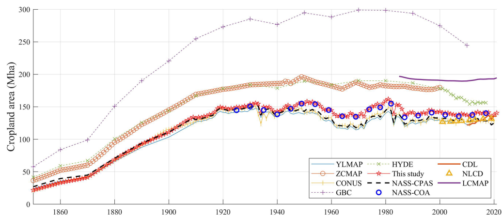
Figure 7. Comparison of the US total cropland area from different sources. The following abbreviations/acronyms are used in the figure: CDL – Cropland Data Layer; NLCD – National Land Cover Database; LCMAP – Land Change Monitoring, Assessment, and Projection; YLMAP – the US cropland map from Yu and Lu (2018); ZCMAP – the US cropland map from Zumkehr and Campbell (2013); CONUS – the cropland map from Li et al. (2023); GBC – the US cropland extracted from the global cropland dataset developed by Cao et al. (2021); HYDE – History database of the Global Environment 3.2 (Klein Goldewijk et al., 2017); NASS-CPAS – the Crop Production Annual Summary data from the National Agricultural Statistics Service of the USDA; and NASS-COA – the Census of Agriculture from the National Agricultural Statistics Service of the USDA. In particular, YLMAP, ZCMAP, CONUS, and GBC are not used in this study to reconstruct crop maps.
