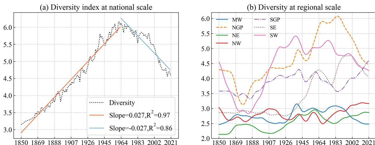
Figure 6. The temporal trend in the diversity value in the US (a) and seven regions (b). NW, SW, NGP, SGP, MW, SE, and NE represent Northwest, Southwest, Northern Great Plains, Southern Great Plains, Midwest, Southeast, and Northeast, respectively. The spatial map of the seven regions is presented in Fig. 5.2-b. To get a better visual pattern, the trends of the seven regions in panel (b) were smoothed by the Gaussian function. The diversity value is calculated based on the reconstructed inventory data.
