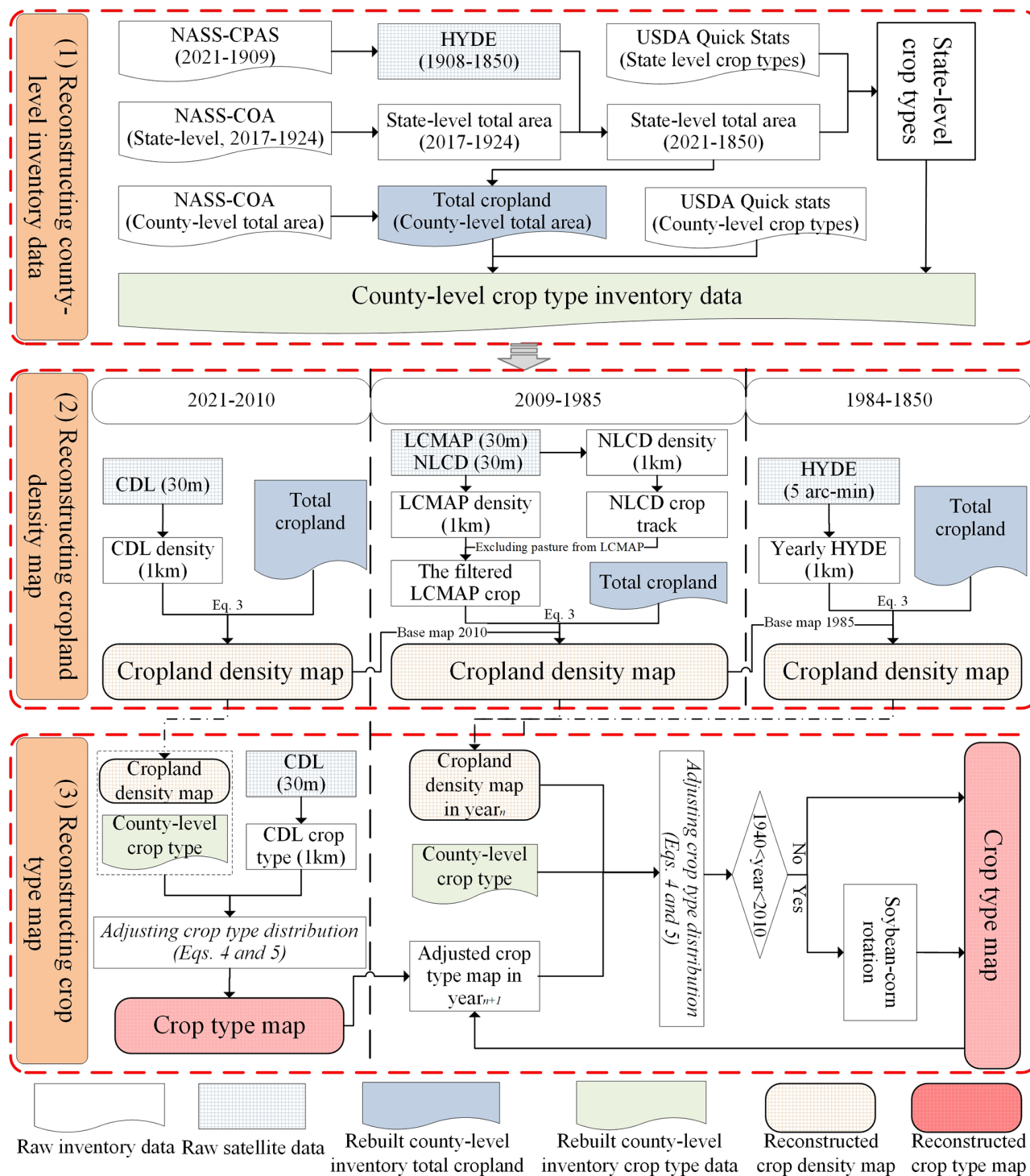
Figure 1. The methodology flow chart. The three boxes with red dashed lines correspond to Sect. 2.2, 2.3, and 2.4, respectively. The county-level total and crop-specific cropland area generated in the box (1) are fed into box (2) and box (3) to reconstruct cropland density and crop type maps, respectively. The following abbreviations/acronyms are used in the figure: NASS-CPAS – Crop Production Annual Summary data from the National Agricultural Statistics Service of the USDA; NASS-COA – Census of Agriculture from the National Agricultural Statistics Service of the USDA; CDL – Cropland Data Layer; NLCD – National Land Cover Database; LCMAP – Land Change Monitoring, Assessment, and Projection; and HYDE – History database of the Global Environment 3.2 (Klein Goldewijk et al., 2017).
