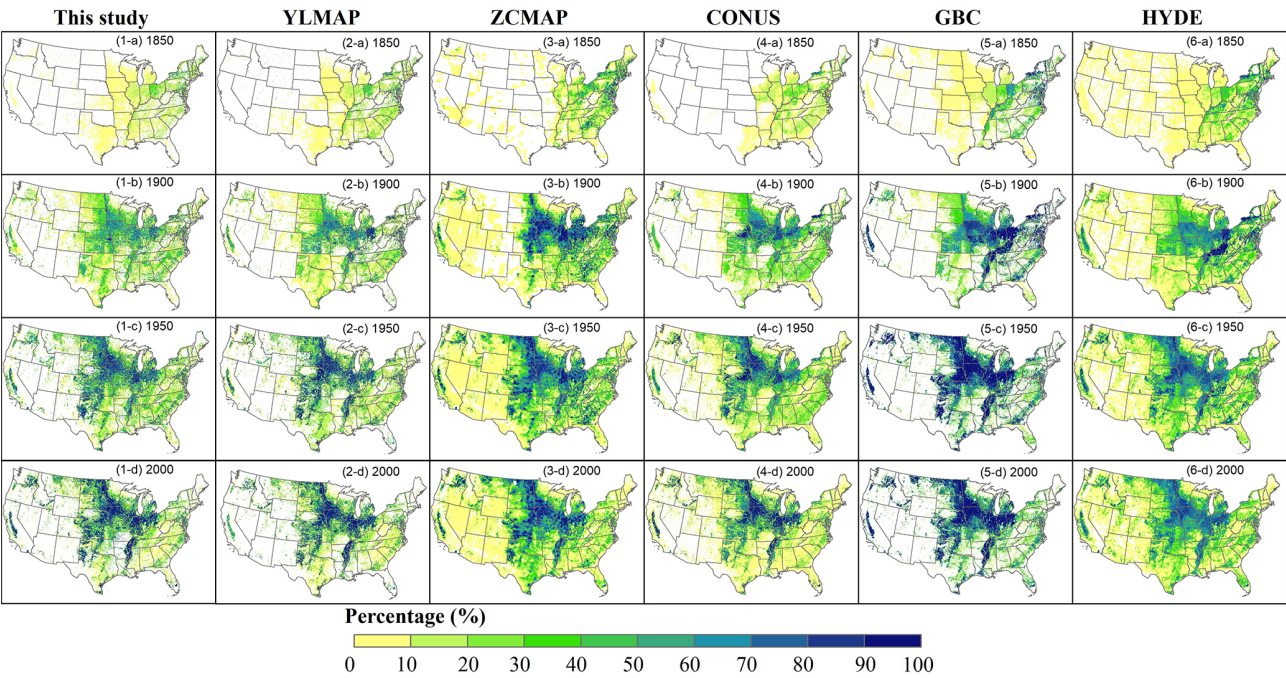
Figure 8. The spatial patterns of cropland from different datasets in the selected years of 1850, 1900, 1950, and 2000. The following abbreviations/acronyms are used in the figure: YLMAP (1 km) – the US cropland map from Yu and Lu (2018); ZCMAP (5 arcmin) – the US cropland map from Zumkehr and Campbell (2013); CONUS (1 km) – the cropland map from Li et al. (2023); GBC (1 km) – the US cropland extracted from the global cropland dataset developed by Cao et al. (2021); and HYDE (5 arcmin) – History database of the Global Environment 3.2 (Klein Goldewijk et al., 2017).
