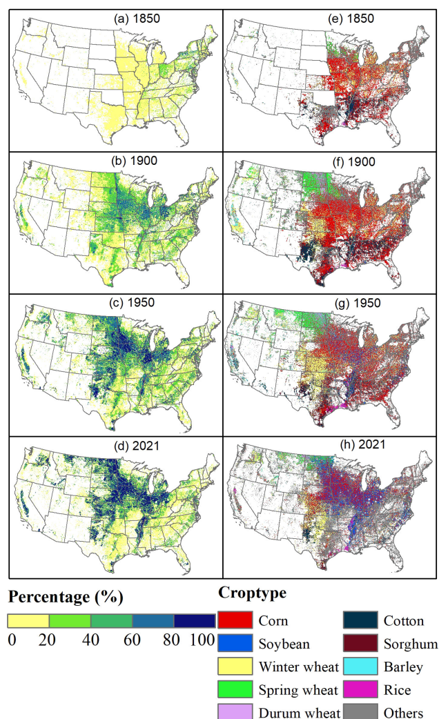
Figure 4. The spatial patterns of cropland percentage (a–d) and dominant crop type (e–h) at a 1 km × 1 km resolution in 1850, 1900, 1950, and 2021. The color bar of “Percentage” indicates the percentage of planting area to the grid area. “Others” represents the remaining crop types.
