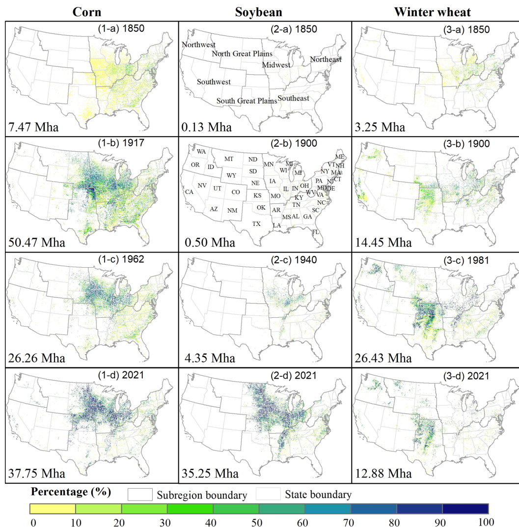
Figure 5. The spatial density pattern of corn, soybean, and winter wheat at a 1 km \times 1 km resolution in the turning point years with abrupt area changes. The first, second, and third columns are the density patterns of corn, soybean, and winter wheat, respectively. The total planting area for each crop type is presented in the bottom left of each panel. The color bar at the bottom indicates the percentage of planting area to the total grid area.
