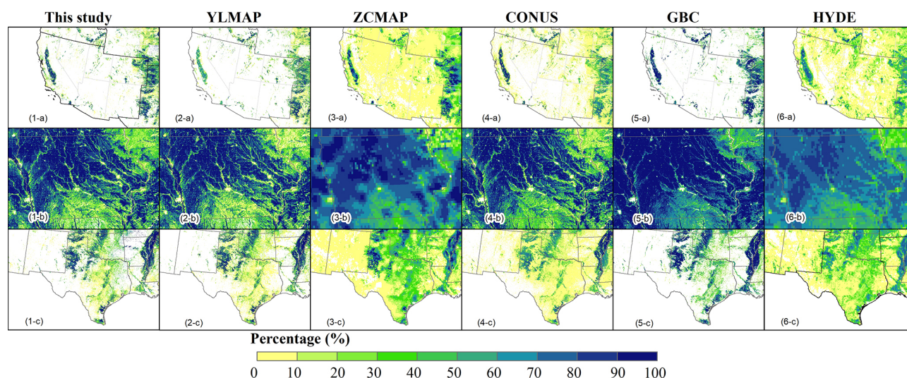
Figure 9. The detailed spatial pattern from different datasets in the year 2000. The following abbreviations/acronyms are used in the figure: YLMAP (1 km) – the US cropland map from Yu and Lu (2018); ZCMAP (5 arcmin) – the US cropland map from Zumkehr and Campbell (2013); CONUS (1 km) – the cropland map from Li et al. (2023); GBC (1 km) – the US cropland extracted from the global cropland dataset developed by Cao et al. (2021); and HYDE (5 arcmin) – History database of the Global Environment 3.2 (Klein Goldewijk et al., 2017). The spatial extent in each row for panels (a), (b), and (c) is for the US Southwest, Iowa, and Texas, respectively.
