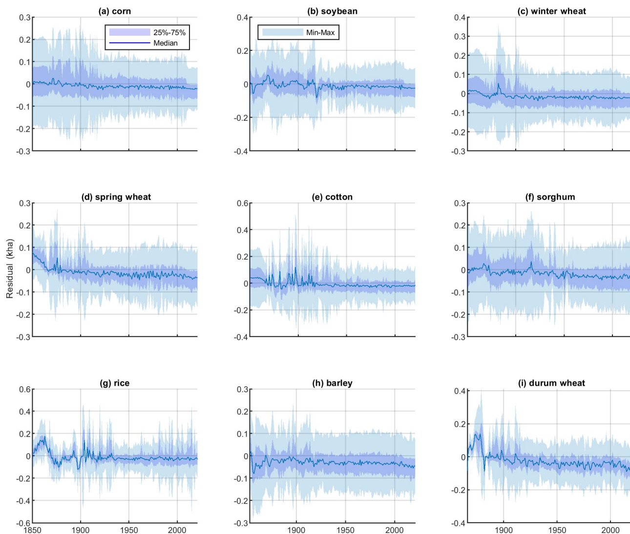
Figure 2. The distribution of residual (the inventory-based crop area minus the rebuilt-map-based crop area, defined by Eq. 6) between the rebuilt inventory and maps from 1850 to 2021 (kha is a thousand hectares). In each year, “Min–Max”, “Median”, and “25 %–75 %” reflect the extent of residual from all counties at levels of “minimum value to maximum value”, “50th percentile”, and “25th percentile to 75th percentile”, respectively.
