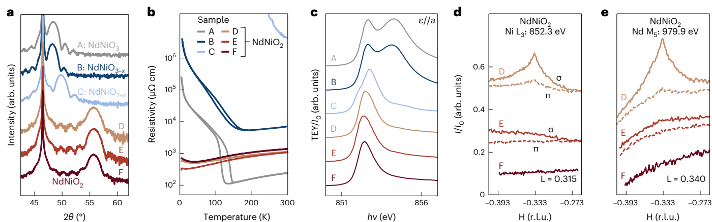
Fig. 1 | Characterization of perovskite NdNiO 3 , oxygen-deficient NdNiO 2-x and infinite-layer NdNiO 2 . a , Cu K \alpha \theta -2 \theta XRD measurements of a sequence of thin films ranging from NdNiO 3 (sample A) to partially reduced NdNiO 2-x (samples B and C) and NdNiO 2 (samples D–F). b , Electrical transport measurements of the same series of samples. c , Total-electron-yield (TEY) XAS measurements of this sample series taken at the Ni L 3 edge with the electric field \epsilon parallel to the
