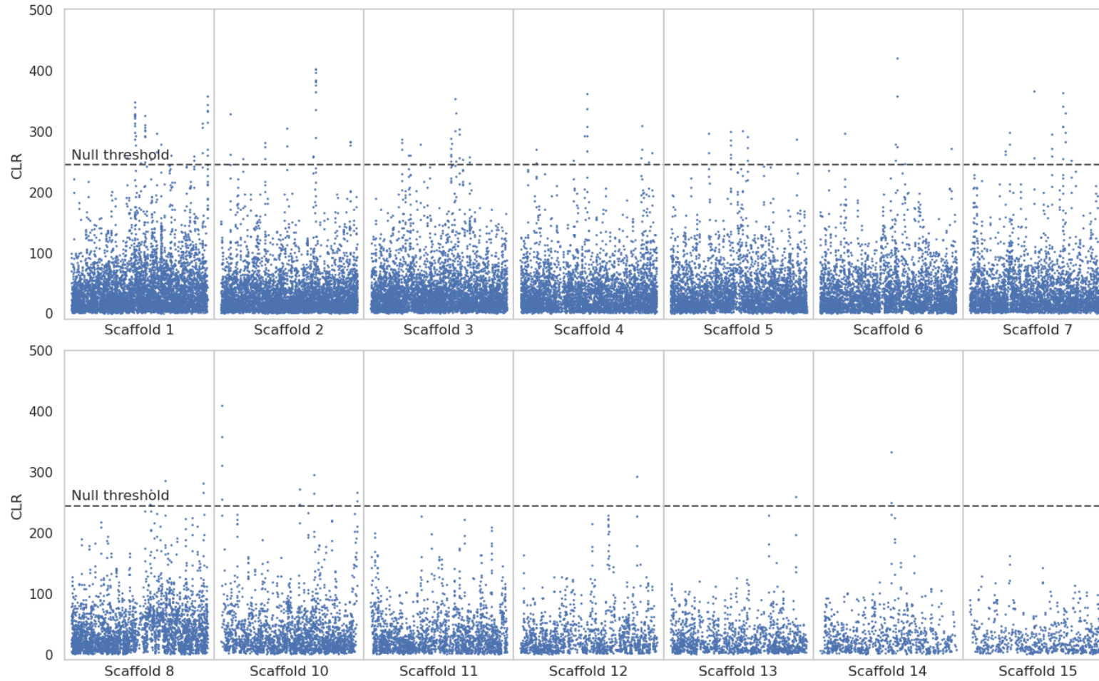
Figure 2: Genome scans for balancing selection using the B_{0MAF} method. Blue data points are CLR values inferred over windows of length 100 SNPs. The dashed line is the threshold for detection, determined by the highest CLR value across 100 simulated replicates of each of the 14 autosomal scaffolds (see "Materials and Methods" section for further details). The x-axis represents the position along the scaffold, and the y-axis represents the CLR value at each window.
