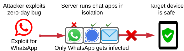
Figure 2. Envisioned Zero-Click Secure Framework: Users access remote, isolated apps via screen sharing, limiting zero-click exploit to the targeted app.
