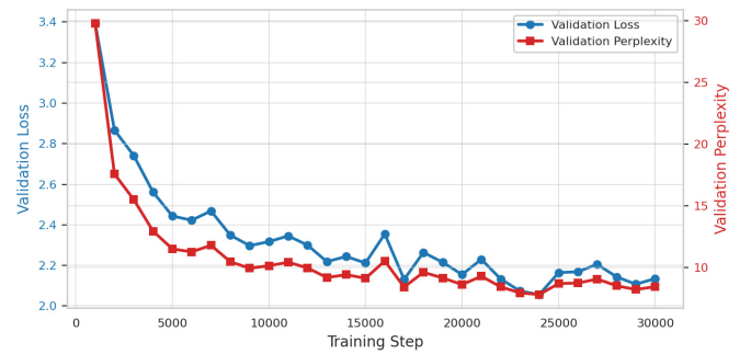
Fig. 6. Validation Loss and Perplexity During Training
