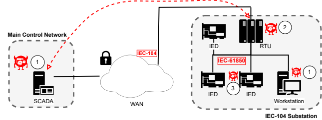
Figure 13: Attack surfaces.
