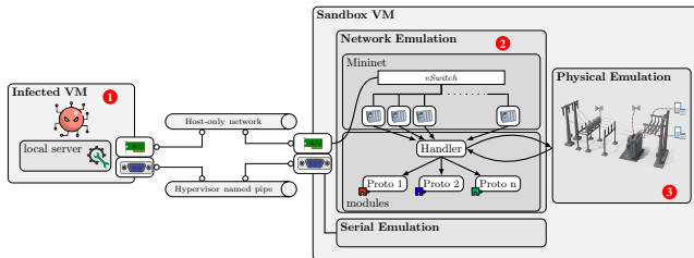
Figure 2: Sandbox architecture.
