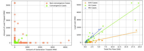
(a) Generation vs. Load. (b) Losses per line attacked.
