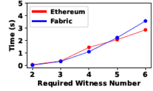
Fig. 7. Time of Getting Data vs. Number of Required Witnesses
