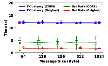
Fig. 10. Transaction Latency in Fabric.
