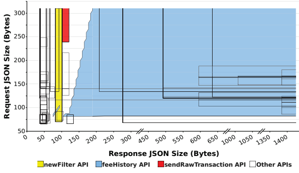
Fig. 3. Area Range of Request/Response JSON Object Size for 44 RPC APIs.
