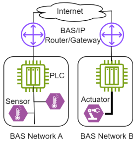
Fig. 1. Example Wired BAS Network
