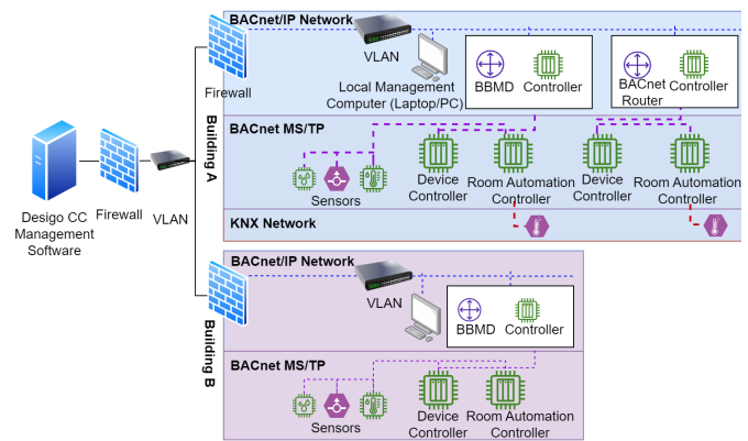
Fig. 5. Simplified Real-world BAS Network
