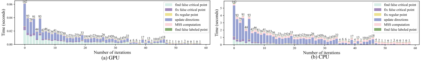
Fig. 11: Timings of outer loop iterations on (a) GPU and (b) CPU with 32 threads; numbers above each bar chart denotes the number of sub-iterations.
