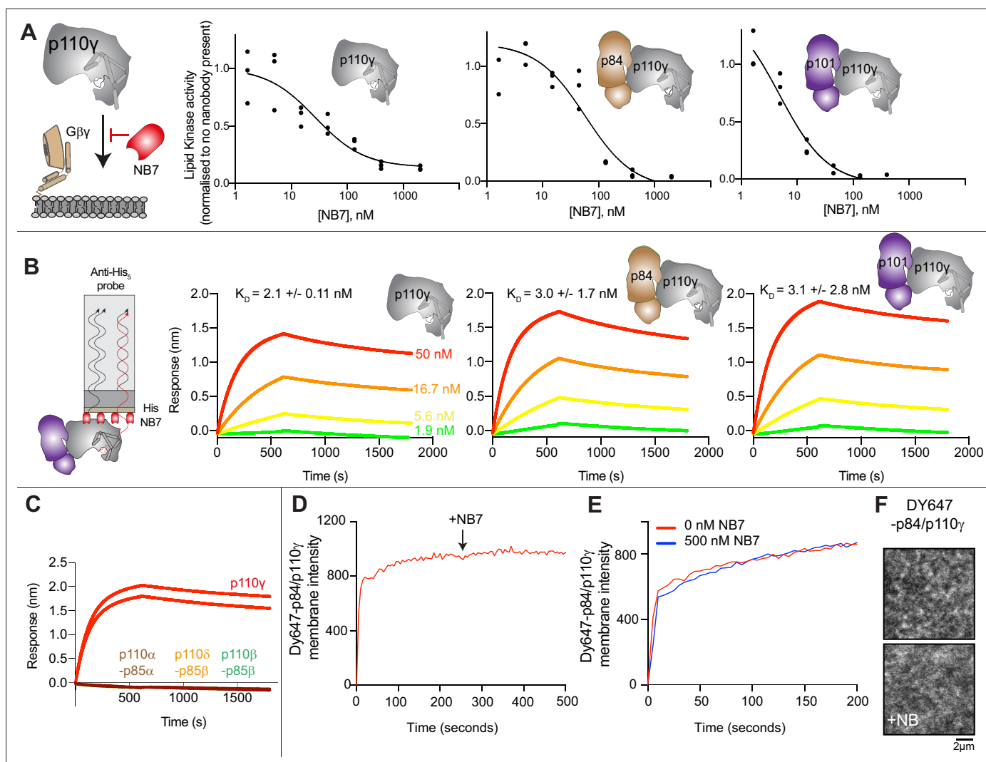
Figure 1. The inhibitory nanobody NB7 binds tightly to all p110γ complexes and inhibits kinase activity, but does not prevent membrane binding. (A) Cartoon schematic depicting nanobody inhibition of activation by lipidated Gβγ (1.5 μM final concentration) on 5% PIP 2 membrane (5% phosphatidylinositol 4,5-bisphosphate [PIP 2 ], 95% phosphatidylserine [PS]) activation. Lipid kinase assays showed a potent inhibition of lipid kinase activity with increasing concentrations of NB7 (3–3000 nM) for the different complexes. Experiments are carried out in triplicate (n=3) with each replicate shown. The y-axis shows lipid kinase activity normalized for each complex activated by Gβγ in the absence of nanobody. Concentrations of each protein were selected to give a lipid kinase value in the detectable range of the ATPase Transcreeper assay. The protein concentration of p110γ (300 nM), p110γ-p84 (330 nM), and p110γ-p101 (12 nM) was different due to intrinsic differences of each complex to be activated by lipidated Gβγ and is likely mainly dependent for the difference seen in NB7 response. (B) Association and dissociation curves for the dose response of His-NB7 binding to p110γ, p110γ-p84, and p110γ-p101 (50–1.9 nM) are shown. A cartoon schematic of biolayer interferometry (BLI) analysis of the binding of immobilized His-NB7 to p110γ is shown on the left. Dissociation constants ( K_D ) were calculated based on a global fit to a 1:1 model for the top three concentrations and averaged with error shown. Error was calculated from the association and dissociation value (n=3) with standard deviation shown. Full details are present in Source data 1 . (C) Association and dissociation curves for His-NB7 binding to p110γ, p110α-p85, p110β-p85, and p110δ-p85. Experiments were performed in duplicate with a final concentration of 50 nM of each class I phosphoinositide 3 kinase (PI3K) complex. (D) Effect of NB7 on PI3Kγ recruitment to supported lipid bilayers containing H-Ras (GTP) and farnesyl-G as measured by total internal reflection fluorescence microscopy (TIRF-M). DY647-p84/p110γ displays rapid equilibration kinetics and is insensitive to the addition of 500 nM nanobody (black arrow, 250 s) on supported lipid bilayers containing H-Ras (GTP) and farnesyl-G. (E) Kinetics of 50 nM DY647-p84/p110γ membrane recruitment appears indistinguishable in the absence and presence of nanobody. Prior to sample injection, DY647-p84/p110γ was incubated for 10 min with 500 nM nanobody. (F) Representative TIRF-M images showing the localization of 50 nM DY647-p84/p110γ visualized in the absence or presence of 500 nM nanobody (+NB7). Membrane composition for panels C–E: 93% DOPC, 5% DOPS, 2% MCC-PE, Ras (GTP) covalently attached to MCC-PE, and 200 nM farnesyl-G.
