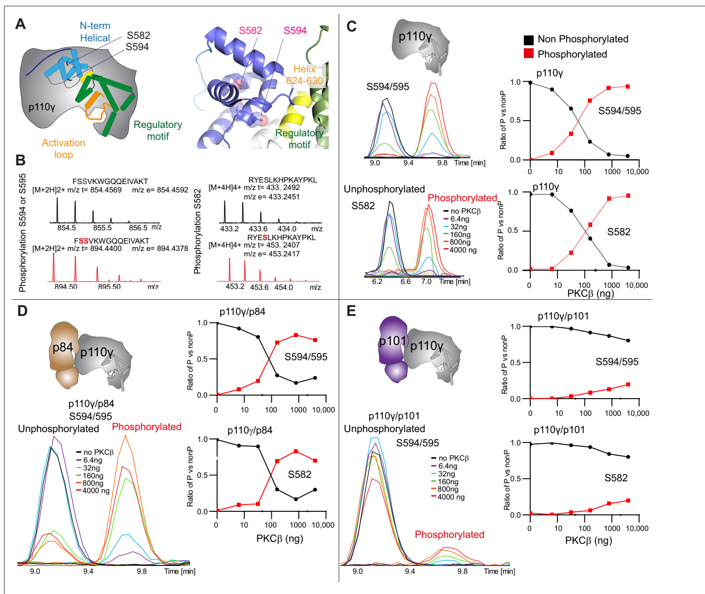
Figure 3. PKCβ leads to dual phosphorylation of internal sites in the helical domain, with selectivity for apo p110γ and p110γ-p84 over p110γ-p101. (A) Putative phosphorylation sites mapped on the structure of p110γ (PDB: 7MEZ) and cartoon schematic. The regions are colored based on domain schematics featured in Figure 2A. (B) Raw MS spectra of the unphosphorylated and phosphorylated peptide for a region spanning 579–592 (RYESLKHPKAYPKL) and 593–607 (FSSVKWGQEQEIVAKT). The putative phosphorylation sites in the sequence are shown in red, with the m/z theoretical ( m/z t) and m/z experimental ( m/z e) shown below each sequence. (C–E) Extracted traces and ratios of the intensity of extracted ion traces of different phosphorylation site peptides (top to bottom: S594/595 and S582) from (C) p110γ, (D) p110γ/p84, or (E) p110γ/p101 samples treated with increasing concentration of PKCβ according to the legend. The black traces in the ratio graphs are the intensity of the non-phosphorylated peptide, and the red traces in the ratio graphs are the intensity of the phosphorylated peptide.
